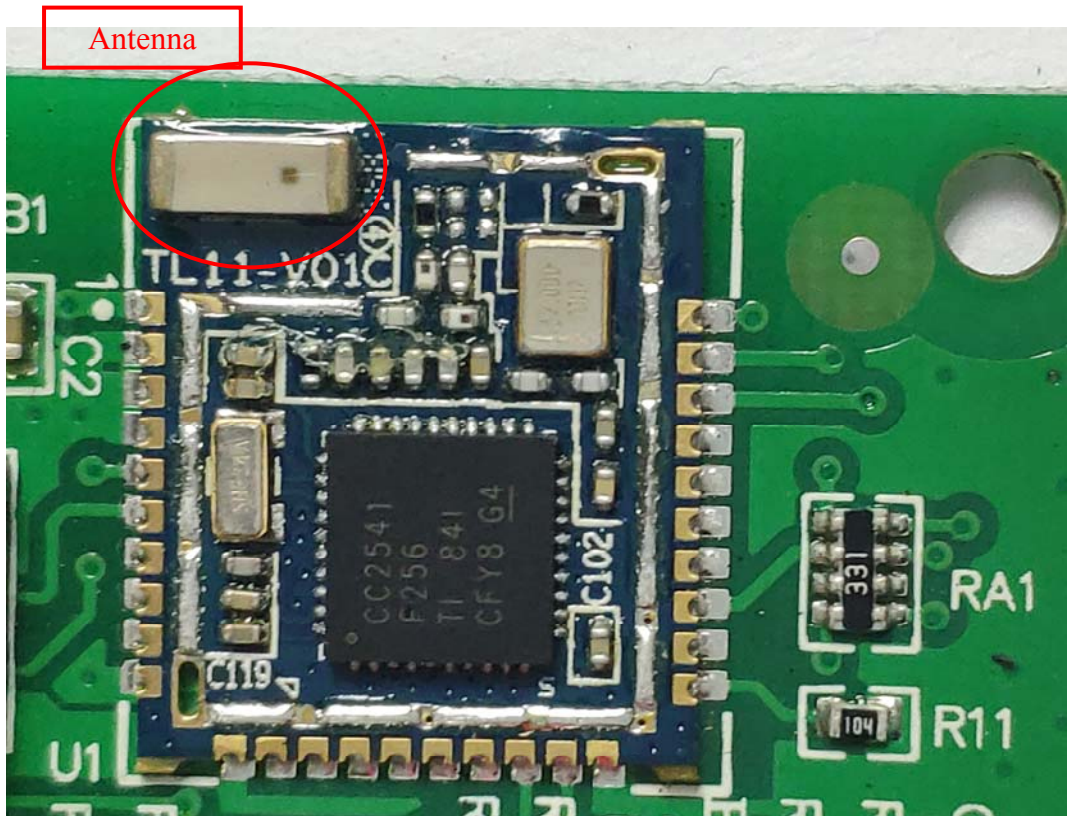
FIGURE 7 UPRIGHT BIKE (M/N: ICR50) CHIP & CRYSTAL ON MAIN BOARD (GENERAL VIEW)
