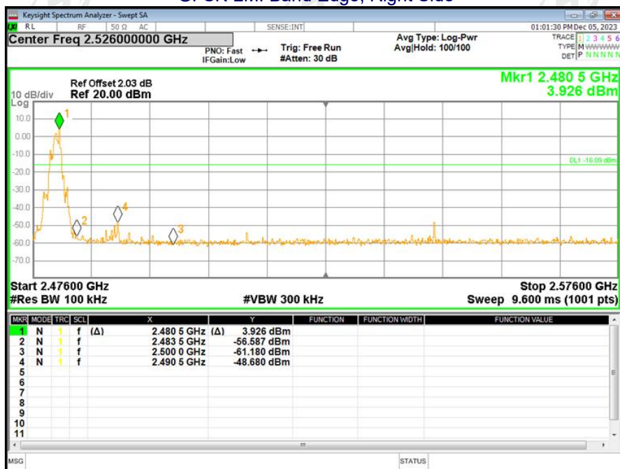
GFSK-2M: Band Edge, Right Side
