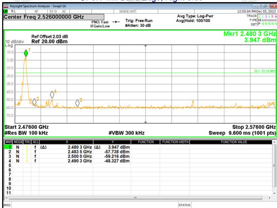
GFSK-1M: Band Edge, Right Side
