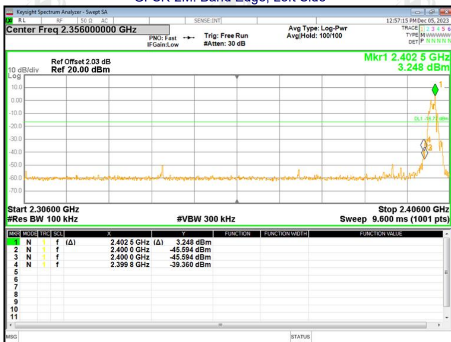
GFSK-2M: Band Edge, Left Side
