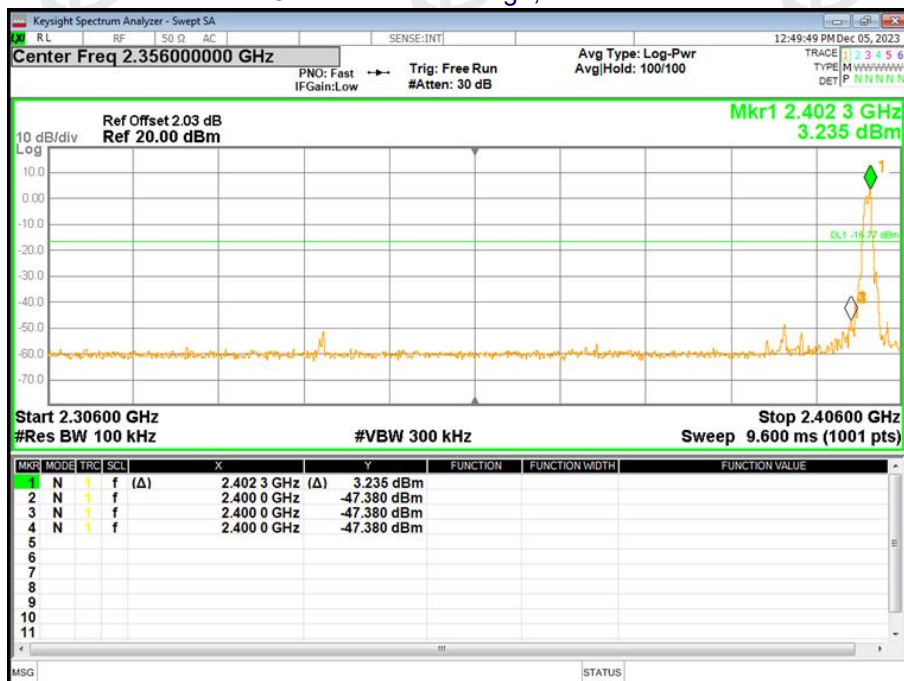
GFSK-1M: Band Edge, Left Side
