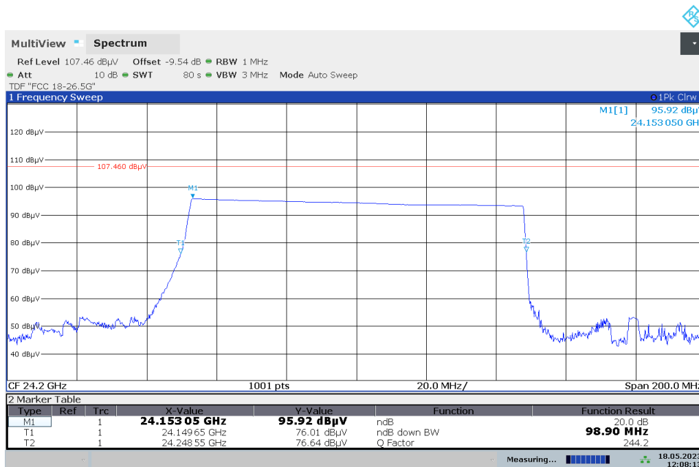
Plots No. 11: 20dB Bandwidth, Horizontal / Vertical Polarization
