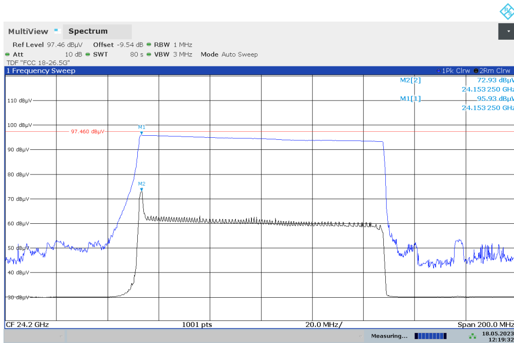
Plots No. 3: Radiated Maximum Field Strength, Horizontal / Vertical Polarization
