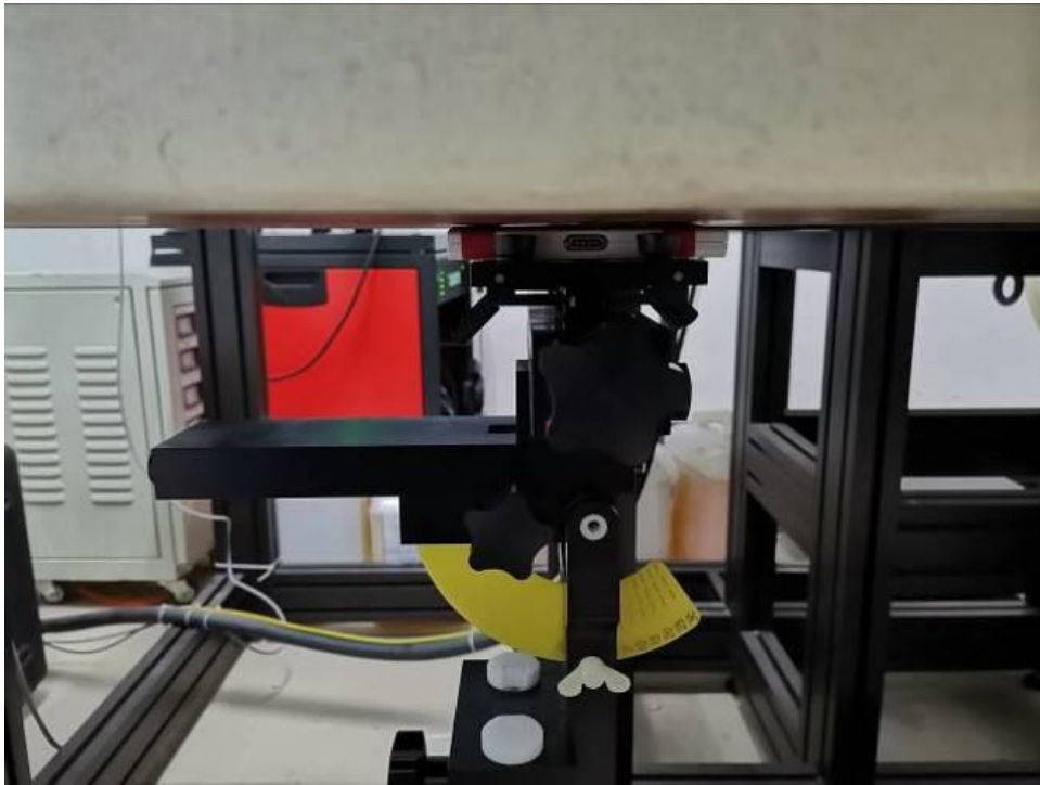
Rear Side (distance 0mm with Flat Phantom)
