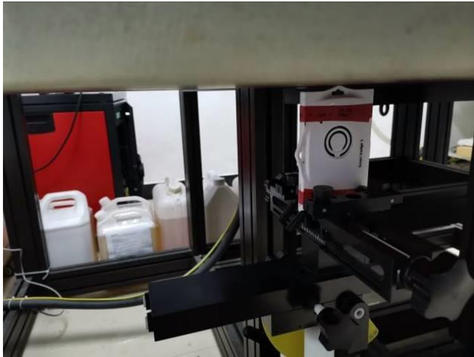
Top Side (distance 0mm with Flat Phantom)
