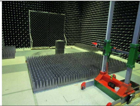
Radiated Emissions Rx 1-25 GHz
