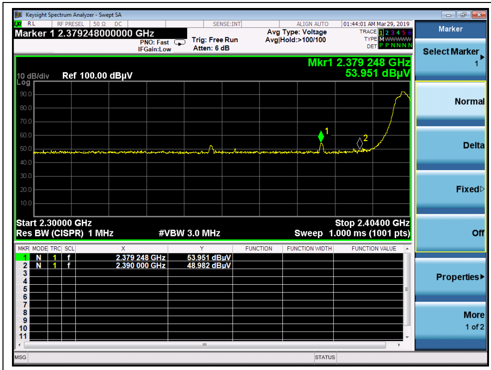
(Channel = 0, PEAK)
