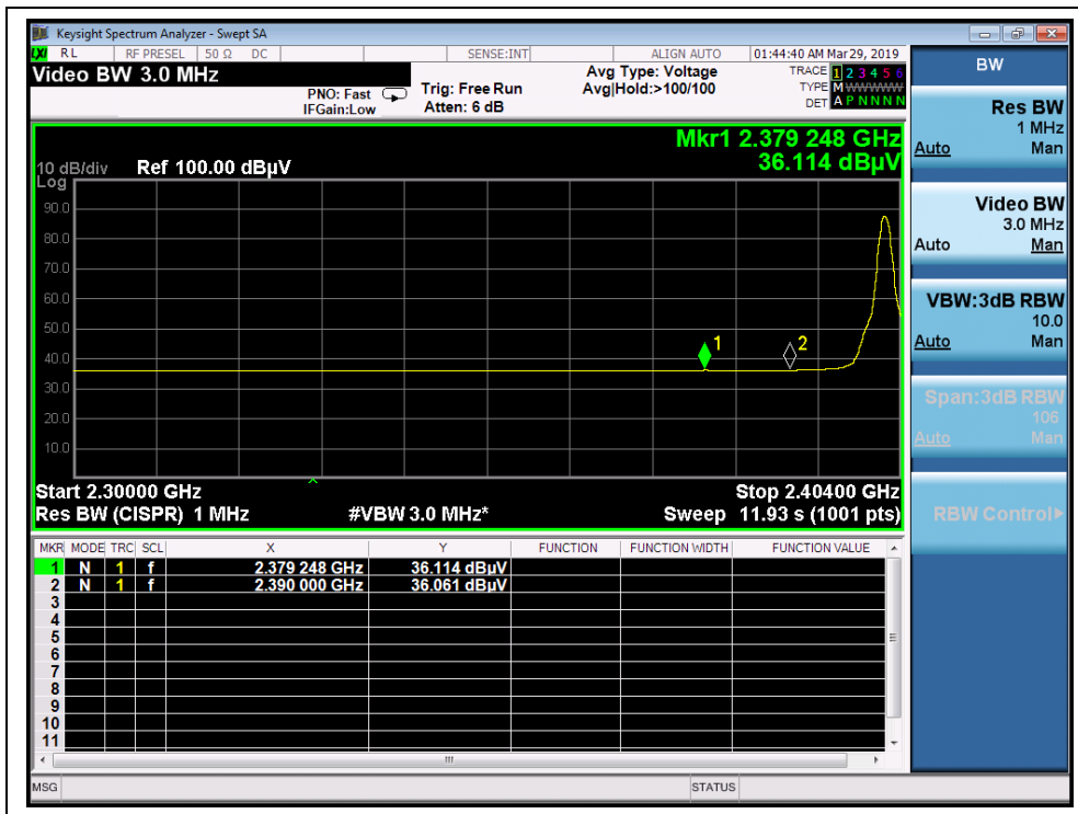
(Channel = 0, AVG)
