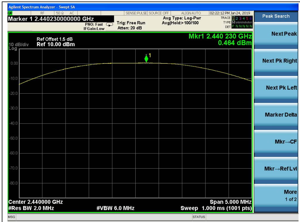
(Channel 3, 2440MHz)
