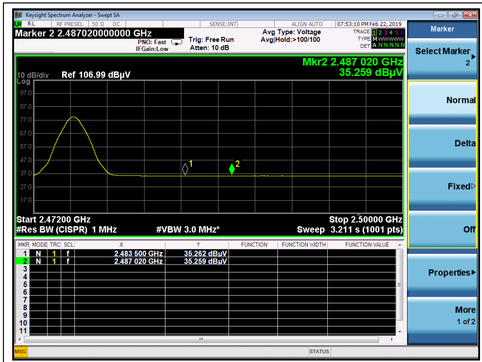
(Channel = 5, AVG)
