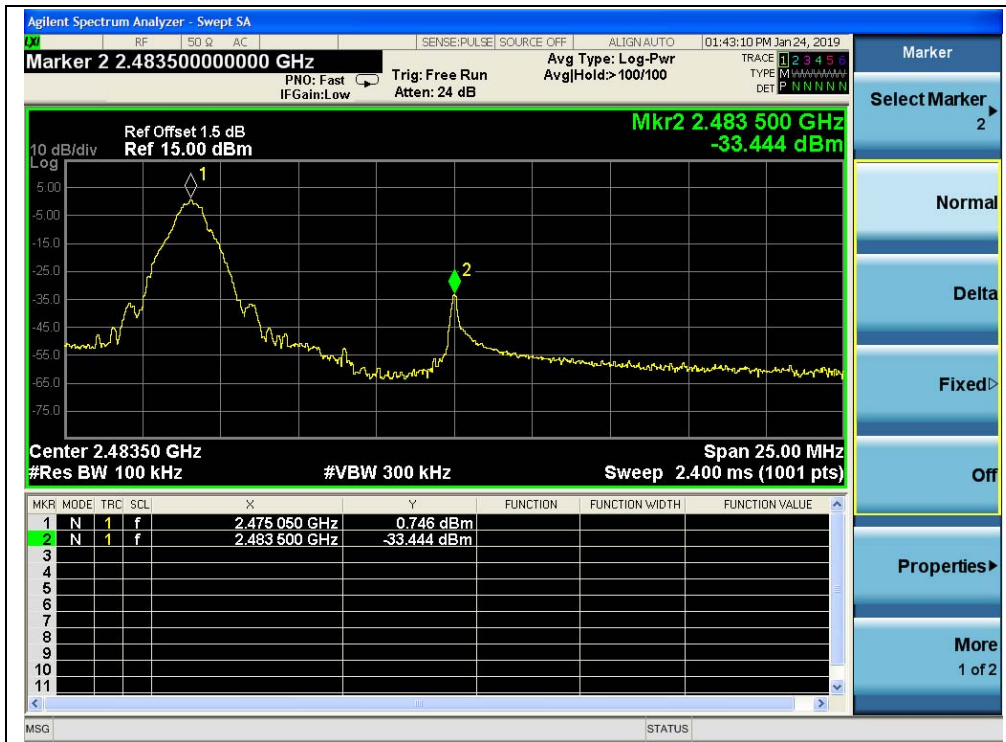
(Band Edge, Channel = 5)
