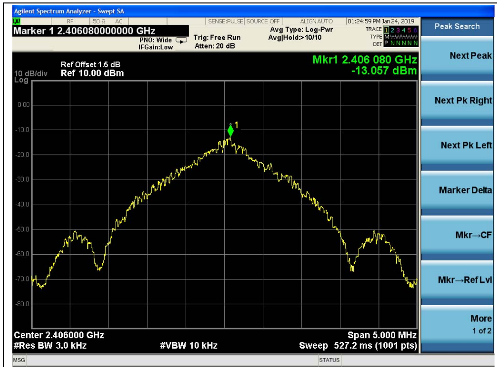
(Channel = 1, 2406MHz)
