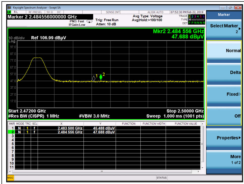
(Channel = 5, PEAK)
