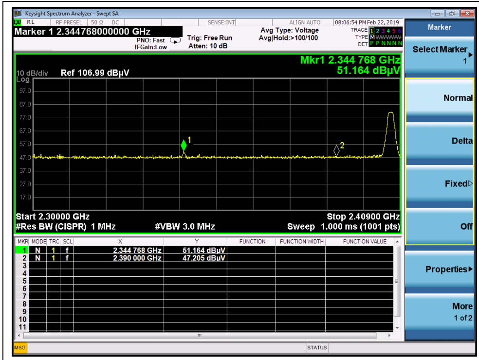
(Channel = 1, PEAK)
