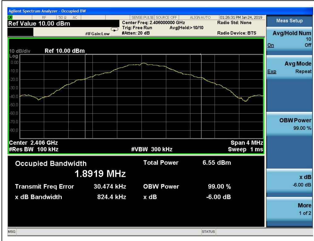
(Channel 1, 2406MHz)
