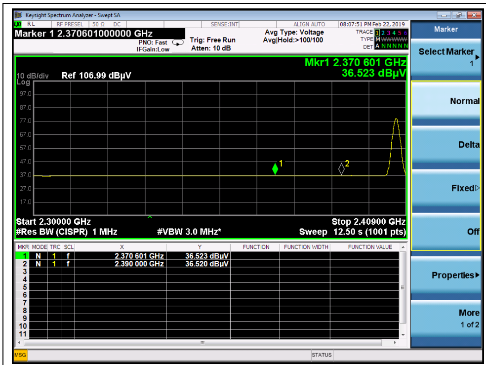
(Channel = 1, AVG)
