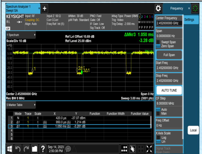
NTNV-11N40MIMO-Ant1-2452
