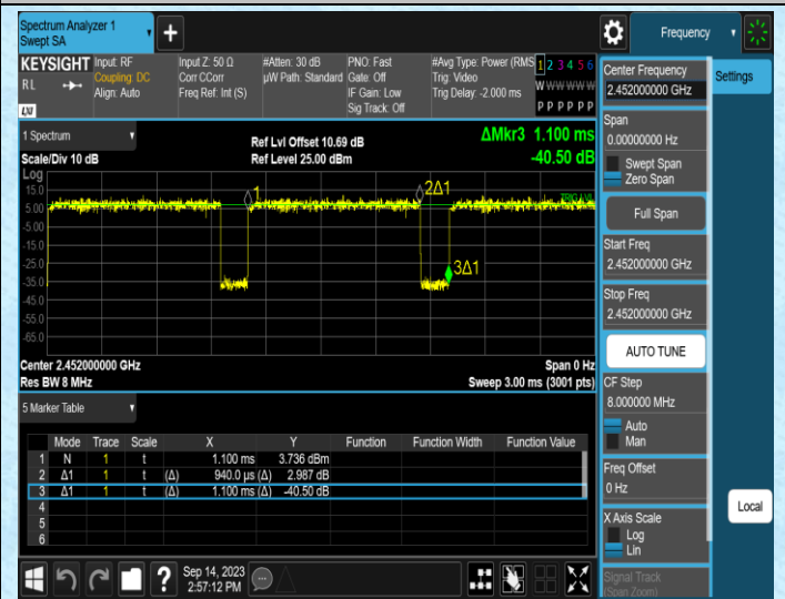
NTNV-11N40MIMO-Ant2-2452
