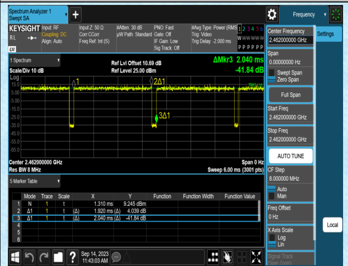
NTNV-11N20SISO-Ant2-2462
