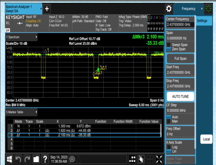
NTNV-11N20SISO-Ant2-2437
