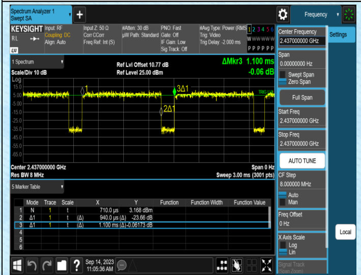
NTNV-11N40SISO-Ant1-2437
