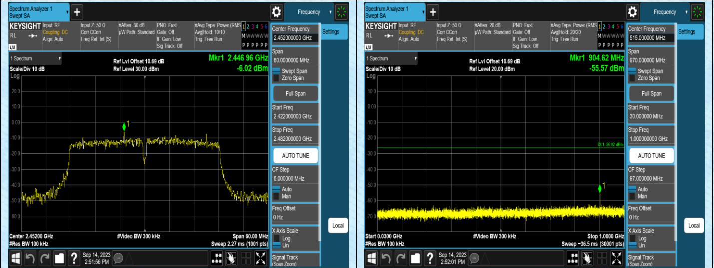
11N40MIMO-Ant1-2452-0~Reference
