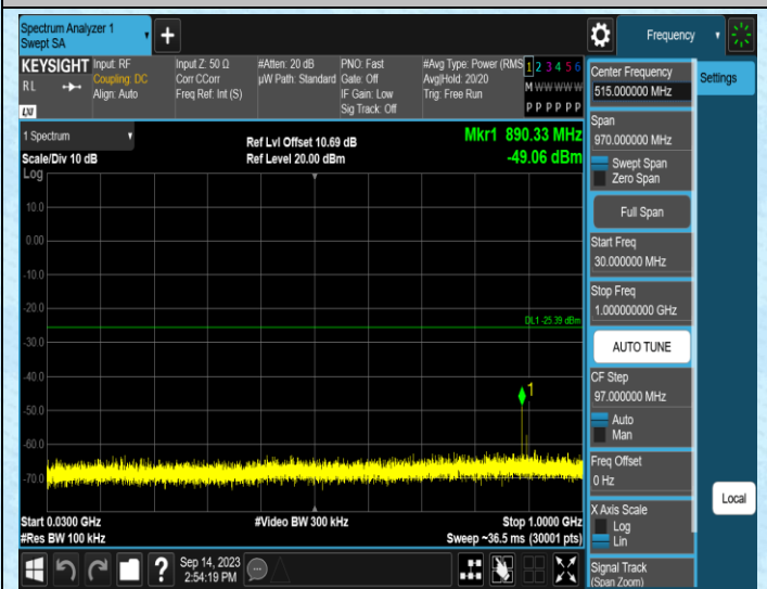
11N40MIMO-Ant2-2452-30~1000
