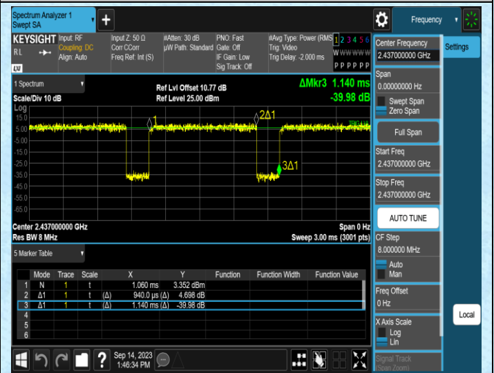
NTNV-11N40SISO-Ant2-2437
