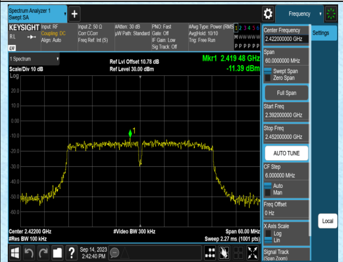
11N40MIMO-Ant2-2422-0~Reference
