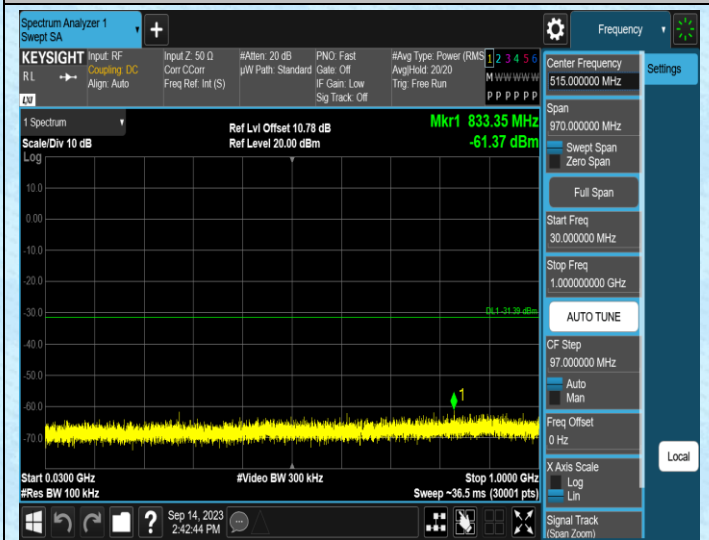
11N40MIMO-Ant2-2422-30~1000
