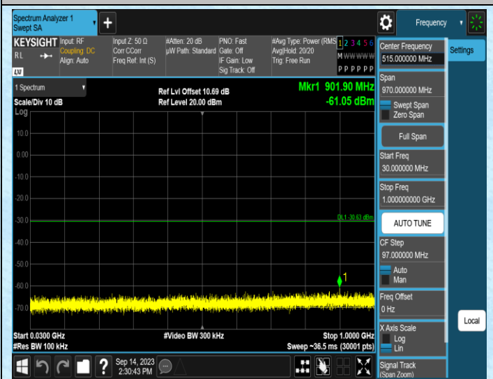
11N20MIMO-Ant2-2462-30~1000
