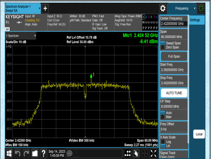
11N40SISO-Ant2-2422-0~Reference
