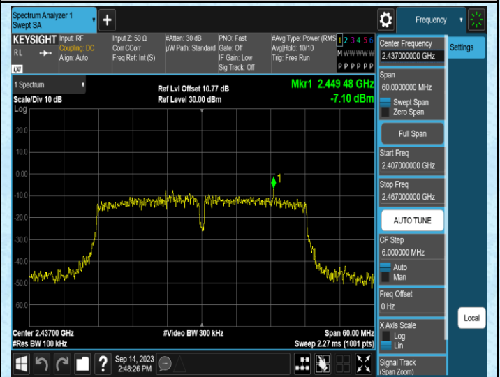
11N40MIMO-Ant2-2437-0~Reference
