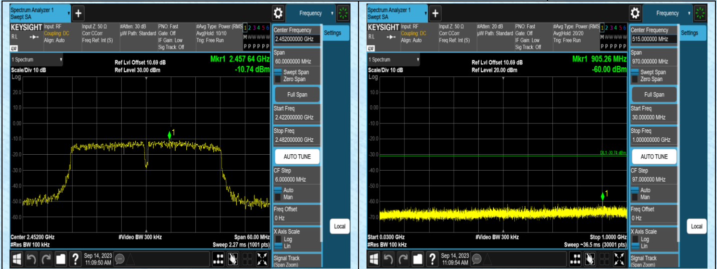
11N40SISO-Ant1-2452-0~Reference
