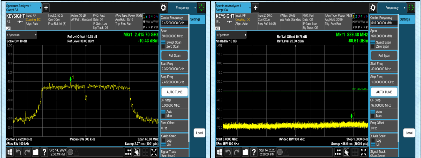
11N40MIMO-Ant1-2422-0~Reference
