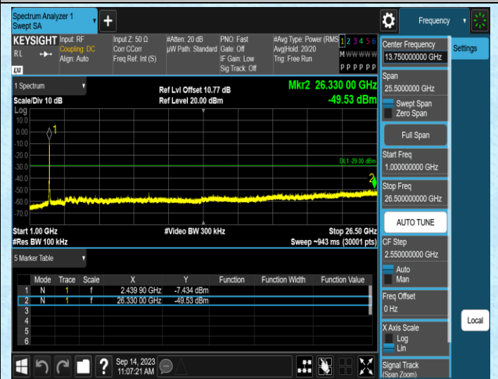
11N40SISO-Ant1-2437-1000~26500
