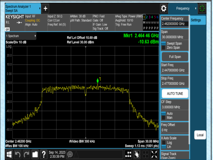
11N20MIMO-Ant2-2462-0~Reference
