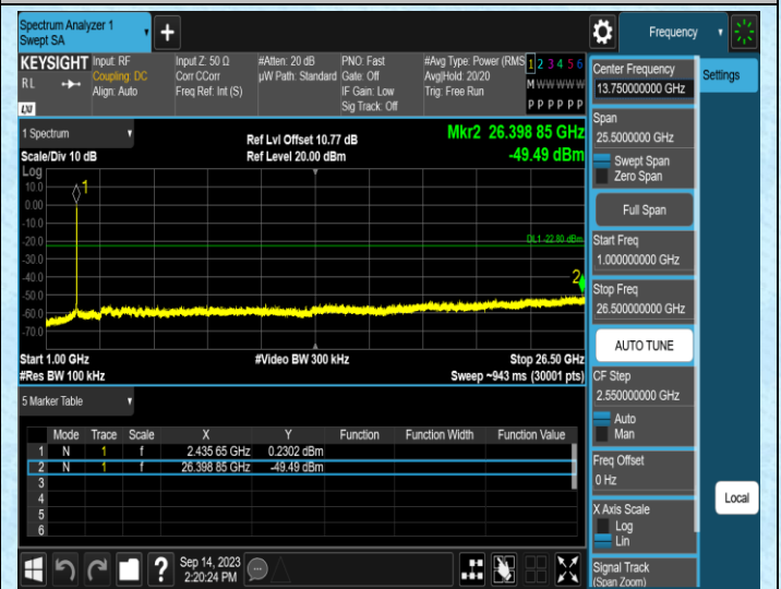
11N20MIMO-Ant2-2437-1000~26500
