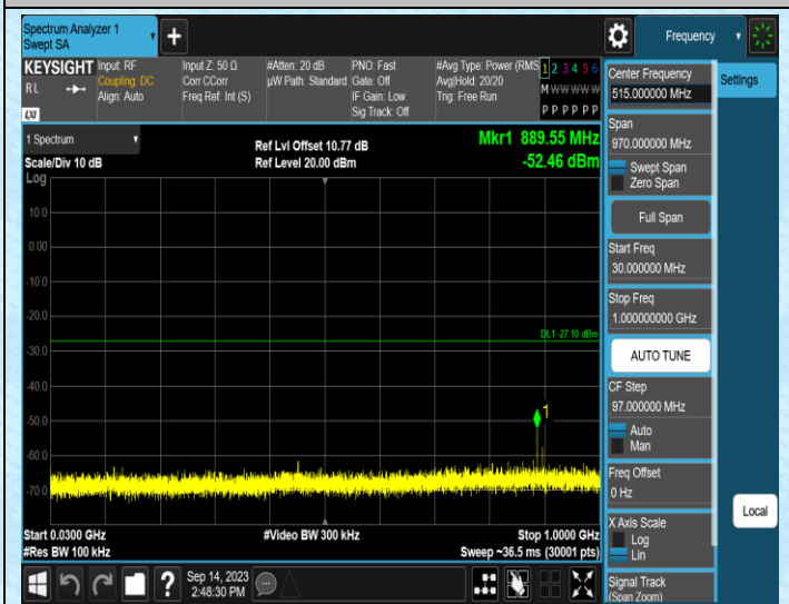
11N40MIMO-Ant2-2437-30~1000
