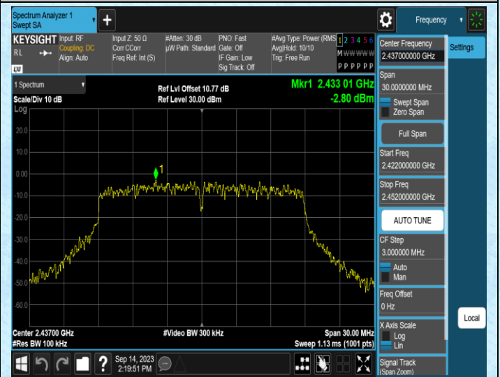
11N20MIMO-Ant2-2437-0~Reference
