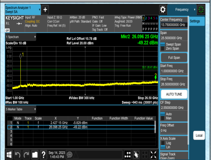
11N40SISO-Ant2-2422-1000~26500
