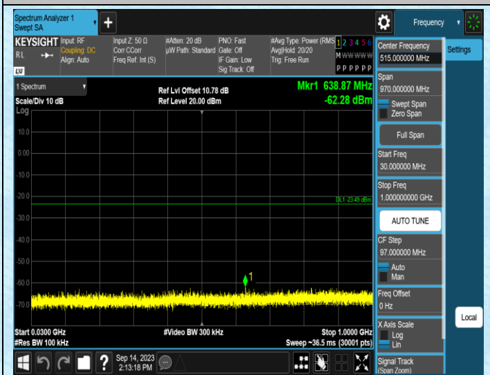
11N20MIMO-Ant2-2412-30~1000
