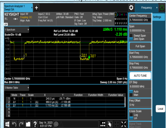
NTNV-11AC40SISO-Ant2-5795
