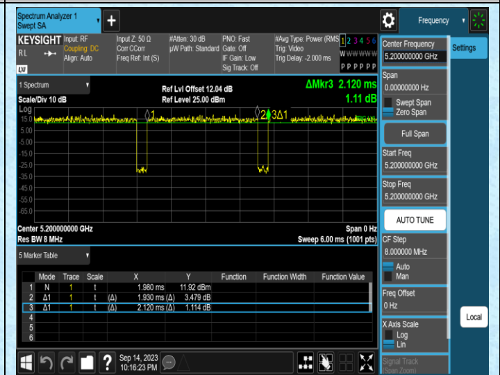
NTNV-11AC20MIMO-Ant2-5200
