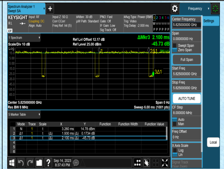
NTNV-11AC20SISO-Ant2-5825
