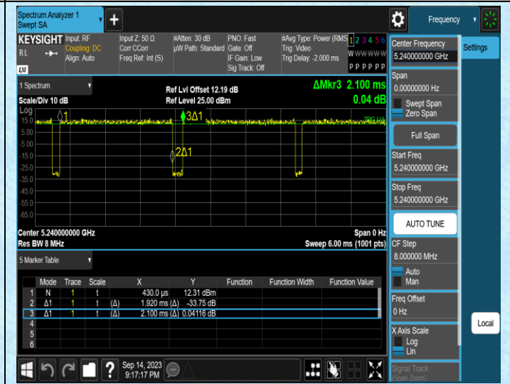
NTNV-11N20MIMO-Ant2-5240
