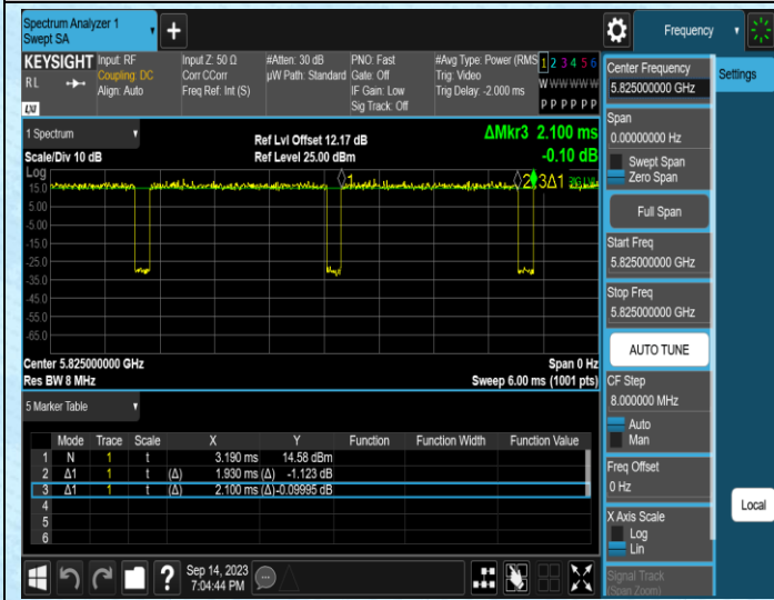
NTNV-11AC20SISO-Ant1-5825
