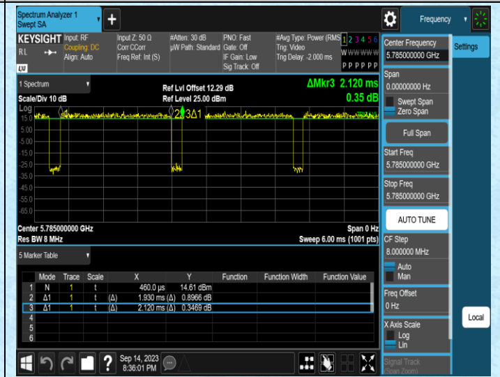
NTNV-11AC20SISO-Ant2-5785
