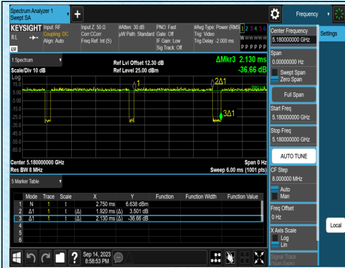
NTNV-11N20MIMO-Ant1-5180
