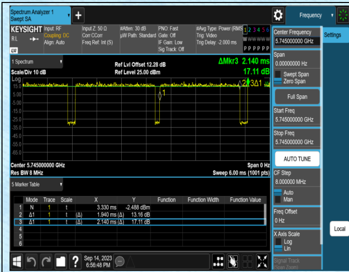
NTNV-11AC20SISO-Ant1-5745
