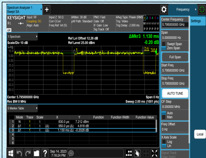
NTNV-11AC40SISO-Ant1-5795
