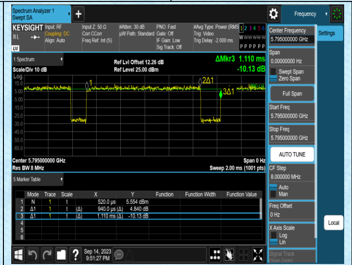
NTNV-11N40MIMO-Ant2-5795
