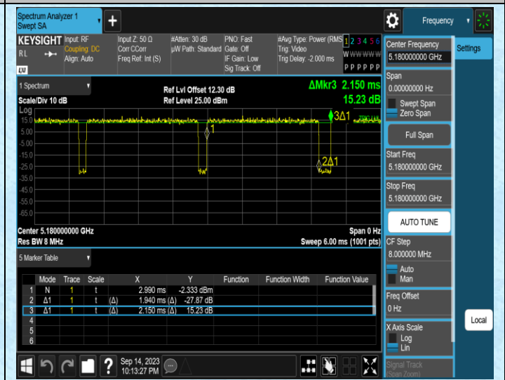
NTNV-11AC20MIMO-Ant2-5180
