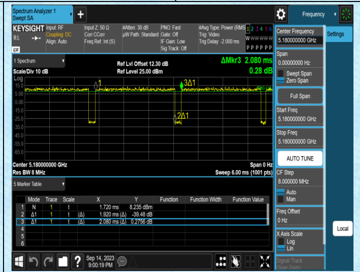
NTNV-11N20MIMO-Ant2-5180
