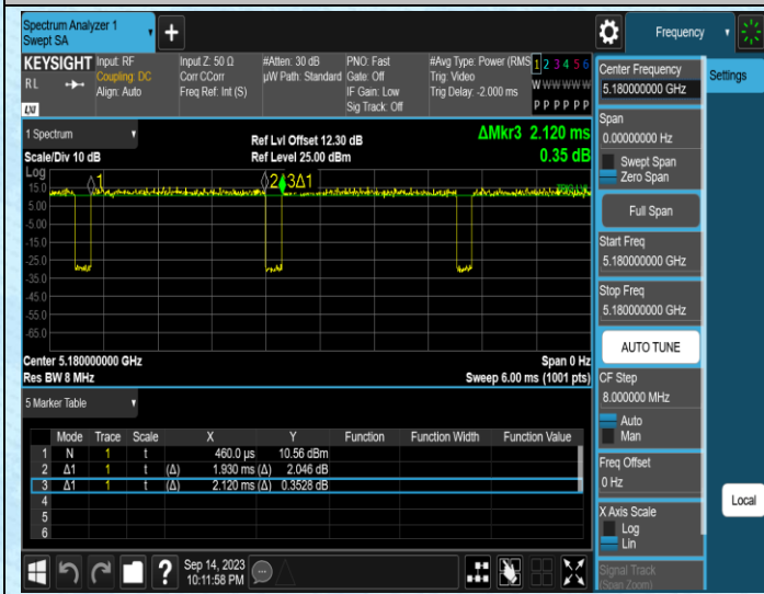
NTNV-11AC20MIMO-Ant1-5180
