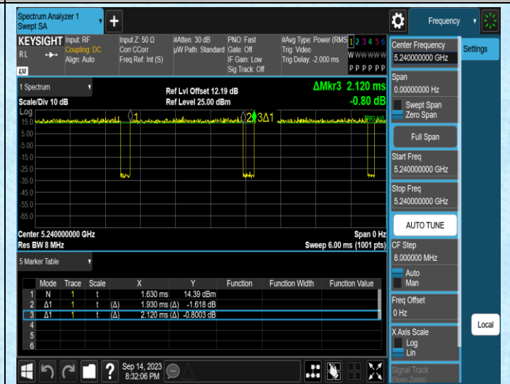
NTNV-11AC20SISO-Ant2-5240
