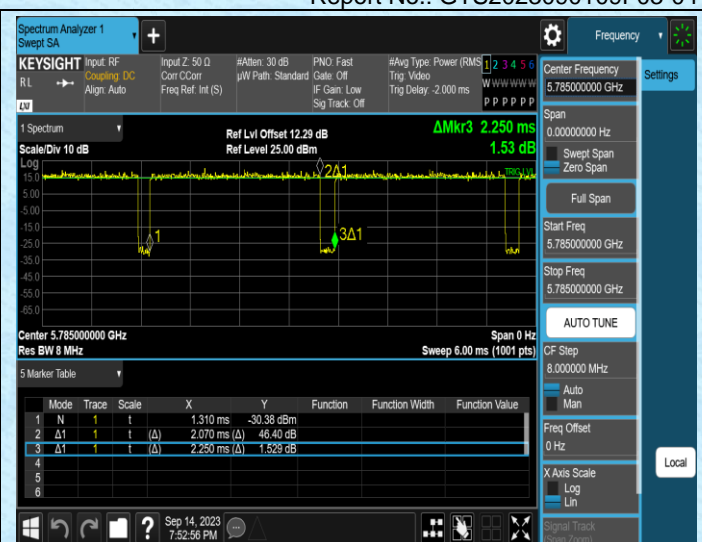
NTNV-11A-Ant2-5785
