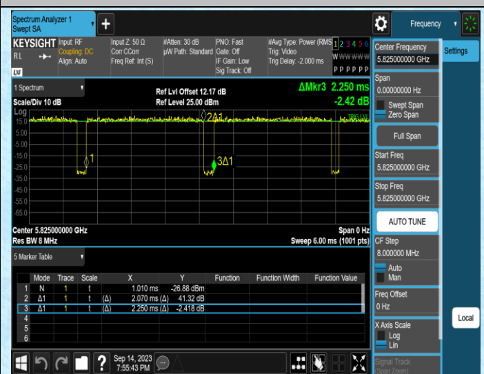
NTNV-11A-Ant2-5825
