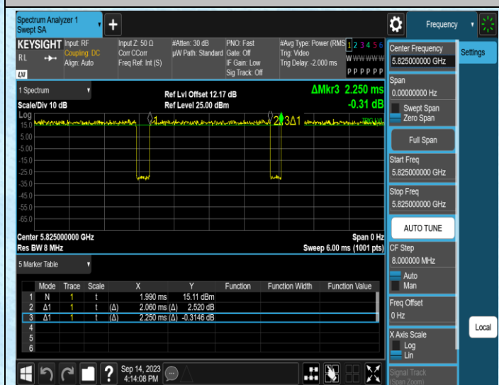
NTNV-11A-Ant1-5825
