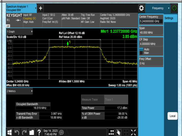
11A-Ant2-5240
