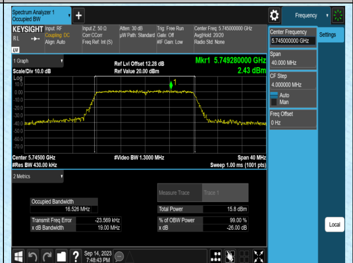
11A-Ant2-5745
