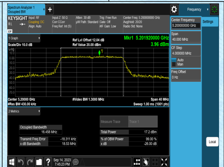
11A-Ant2-5200
