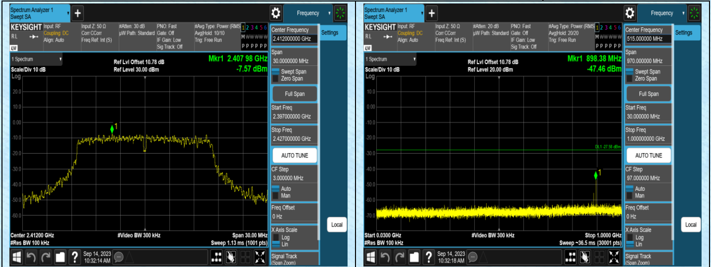
11G-Ant1-2412-0~Reference
