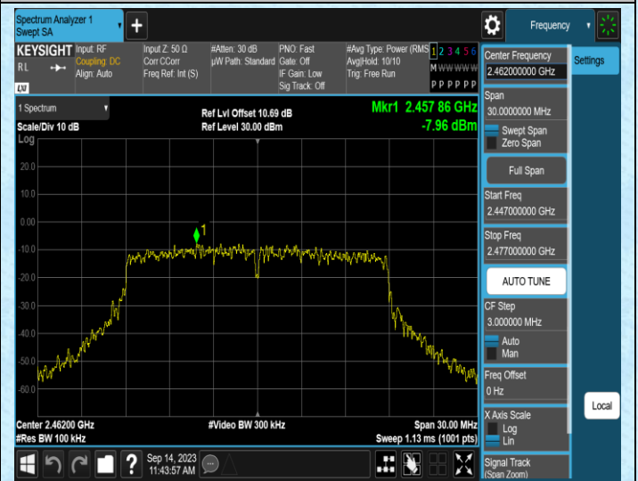
11N20SISO-Ant2-2462-0~Reference
