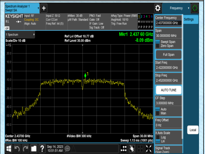
11N20SISO-Ant1-2437-0~Reference
