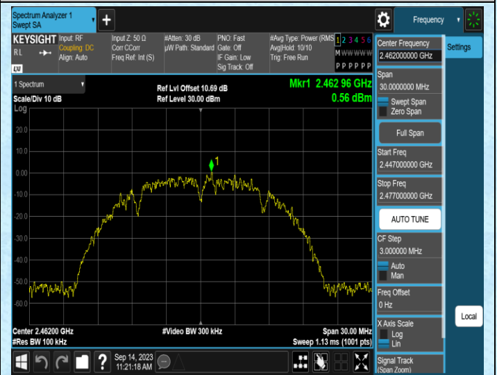
11B-Ant2-2462-0~Reference
