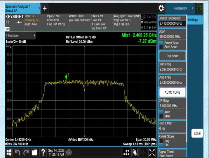
11G-Ant2-2412-0~Reference
