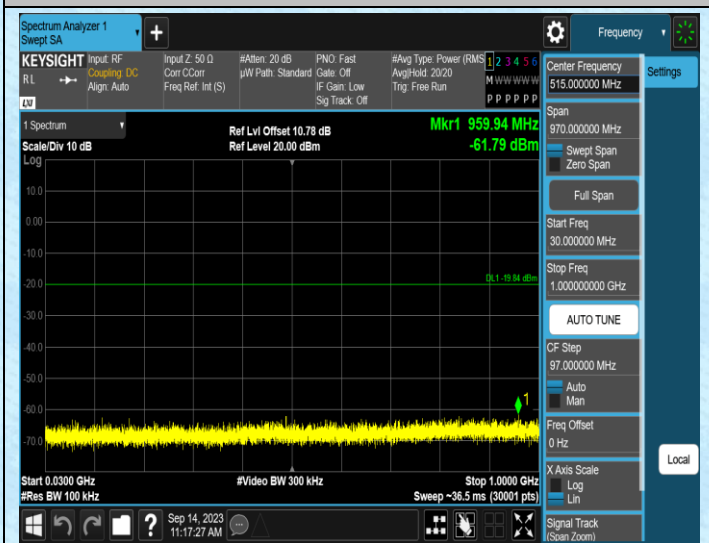
11B-Ant2-2412-30~1000
