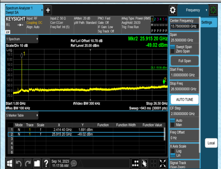
11B-Ant2-2412-1000~26500
