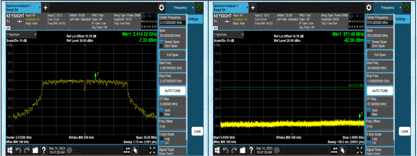
11N20SISO-Ant1-2412-0~Reference
