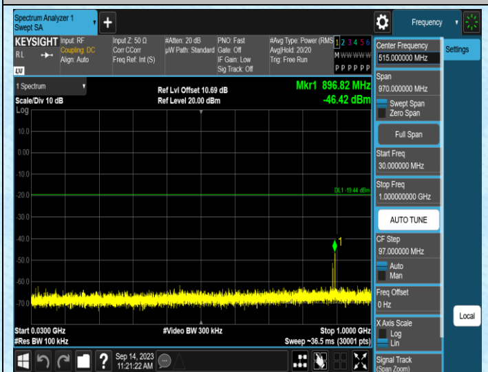
11B-Ant2-2462-30~1000
