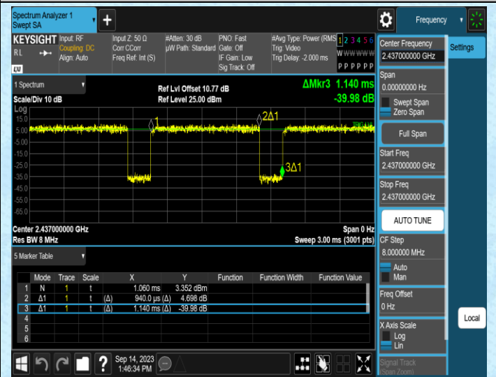
NTNV-11N40SISO-Ant2-2437
