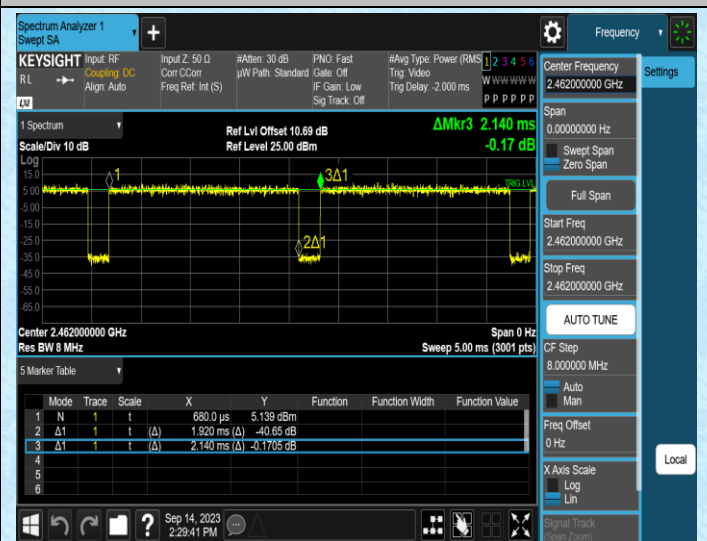
NTNV-11N20MIMO-Ant2-2462
