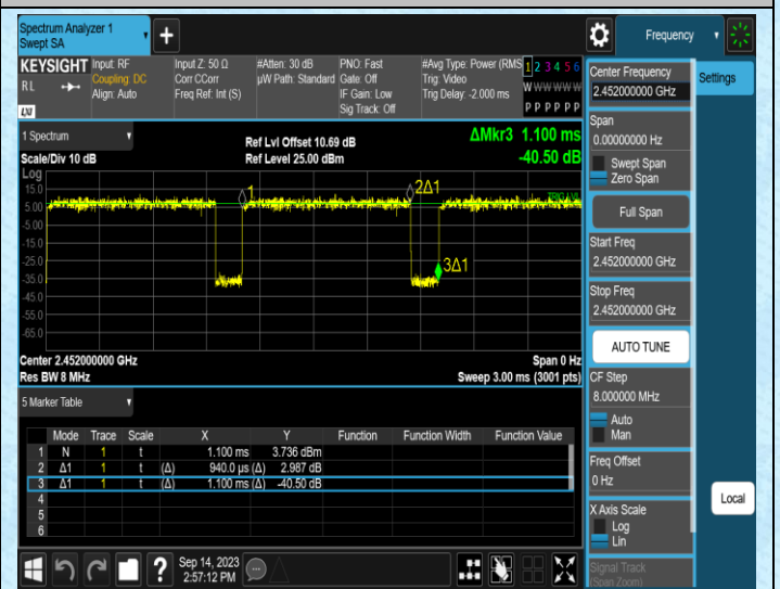
NTNV-11N40MIMO-Ant2-2452
