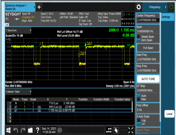
NTNV-11N40SISO-Ant1-2437
