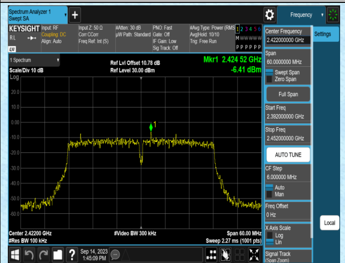
11N40SISO-Ant2-2422-0~Reference
