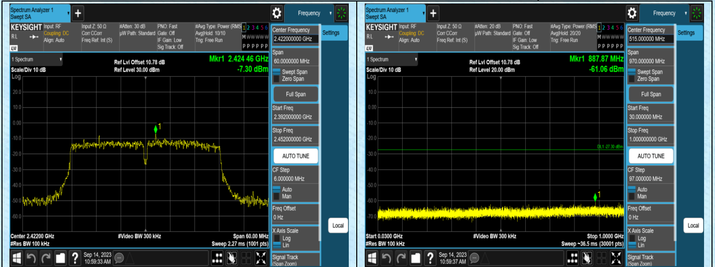
11N40SISO-Ant1-2422-0~Reference
