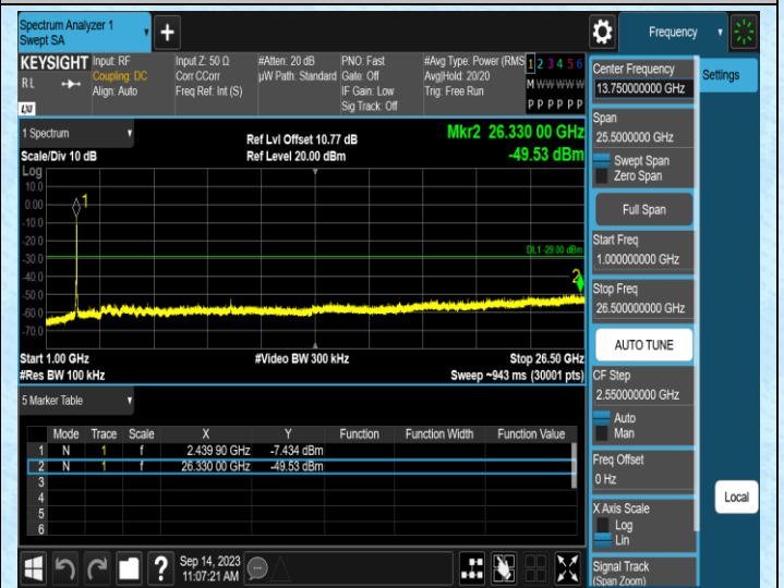
11N40SISO-Ant1-2437-1000~26500
