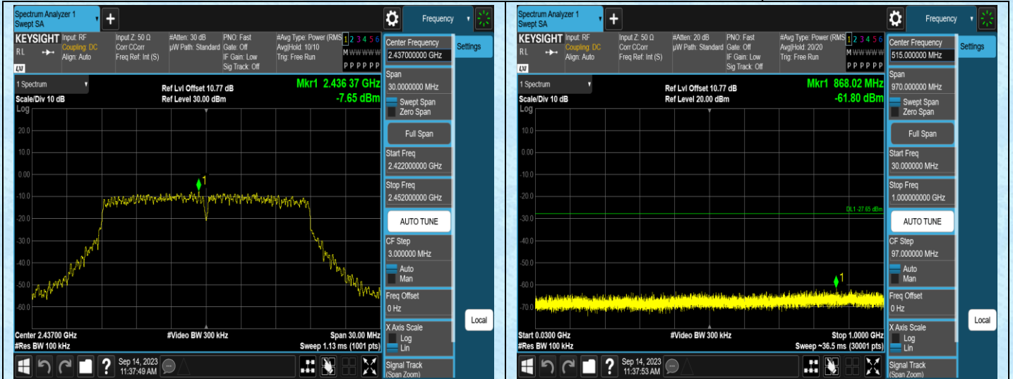
11N20SISO-Ant2-2437-0~Reference
