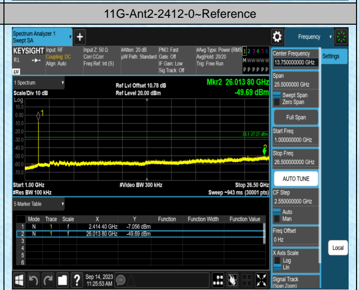
11G-Ant2-2412-1000-26500
