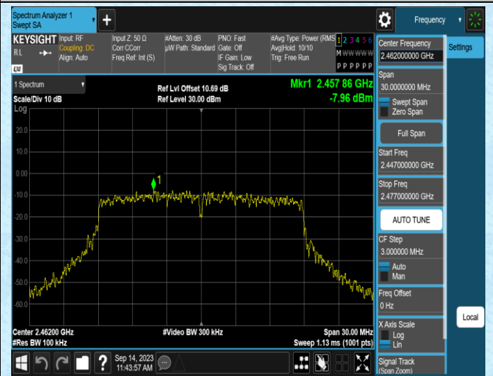
11N20SISO-Ant2-2462-0~Reference
