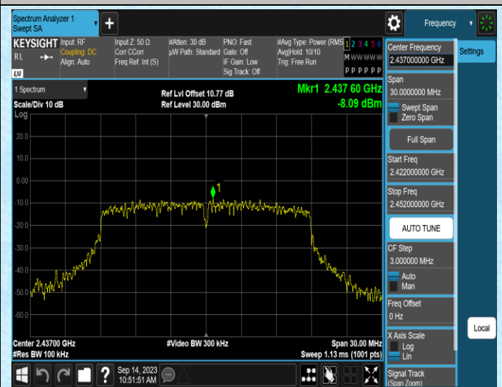
11N20SISO-Ant1-2437-0~Reference
