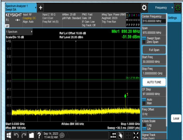
11N20SISO-Ant2-2462-30~1000
