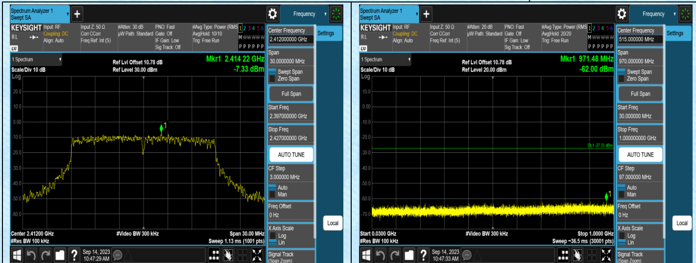
11N20SISO-Ant1-2412-0~Reference
