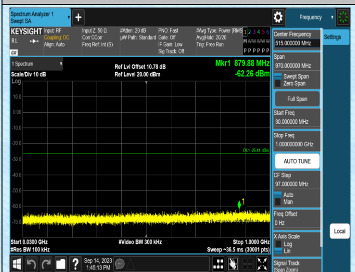
11N40SISO-Ant2-2422-30~1000
