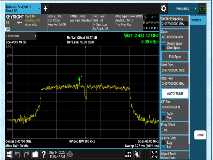
11N40SISO-Ant1-2437-0~Reference
