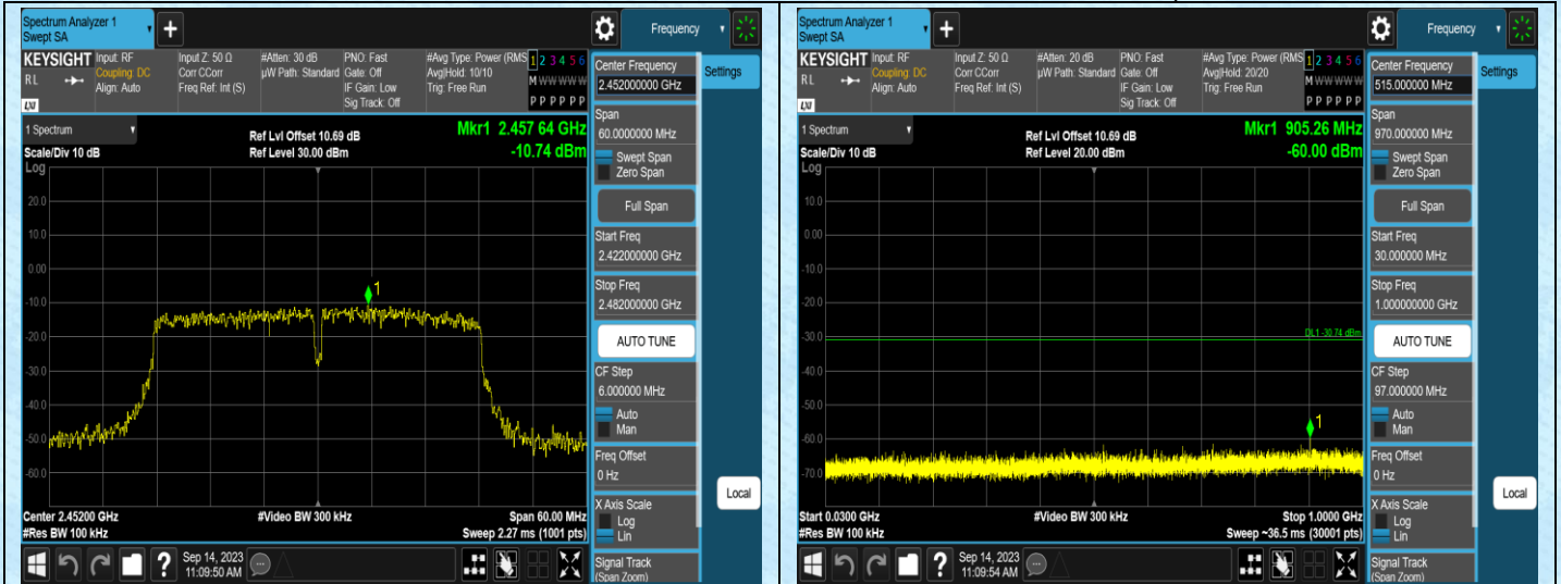
11N40SISO-Ant1-2452-0~Reference
