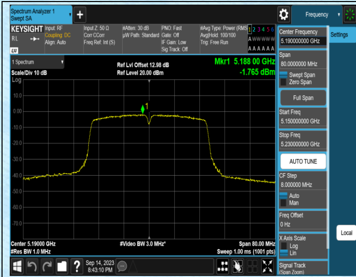
11AC40SISO-Ant2-5190
