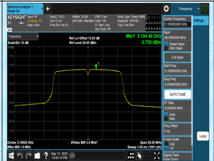
11AC40MIMO-Ant2-5190
