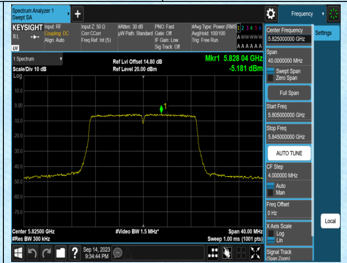
11N20MIMO-Ant2-5825
