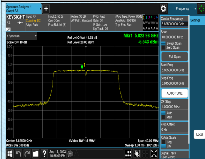
11AC20MIMO-Ant1-5825
