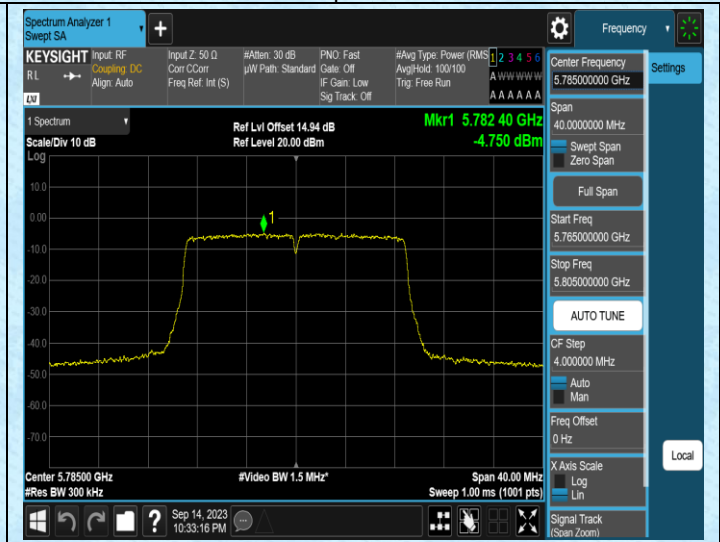
11AC20MIMO-Ant2-5785
