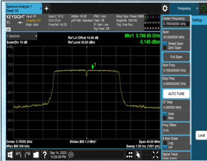
11AC20MIMO-Ant1-5785
