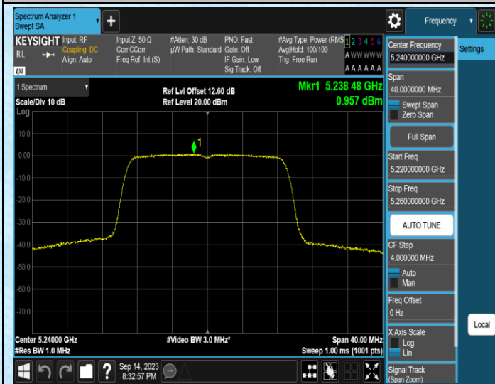
11AC20SISO-Ant2-5240
