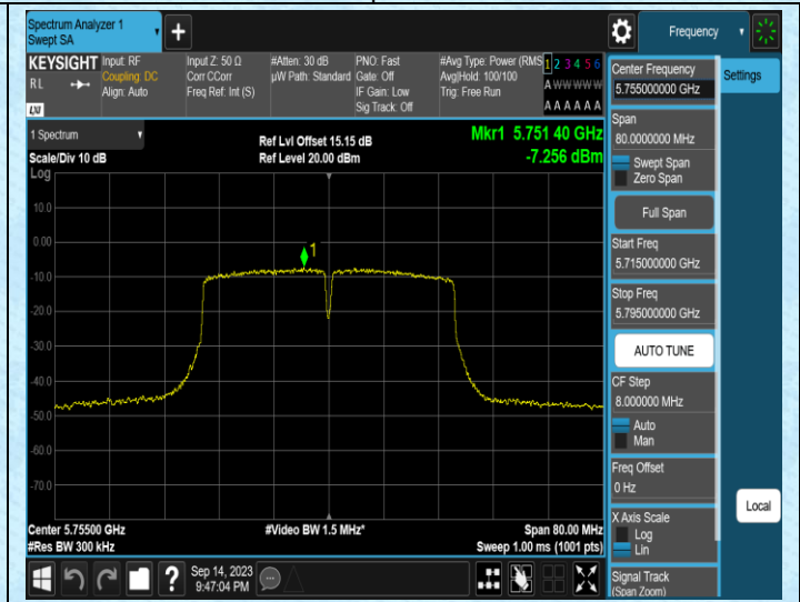
11N40MIMO-Ant2-5755
