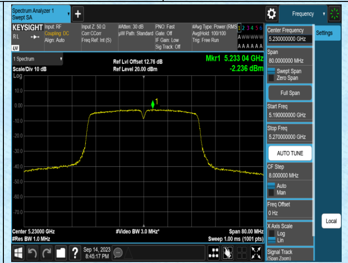
11AC40SISO-Ant2-5230
