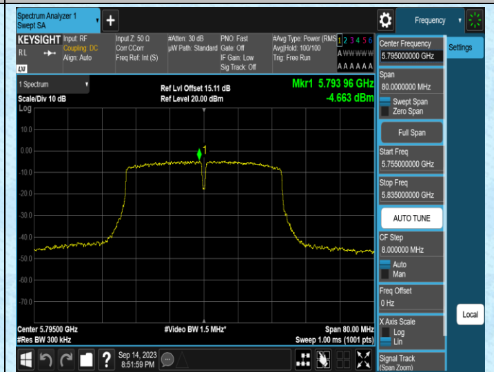
11AC40SISO-Ant2-5795
