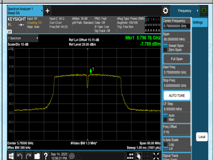
11AC40MIMO-Ant2-5795
