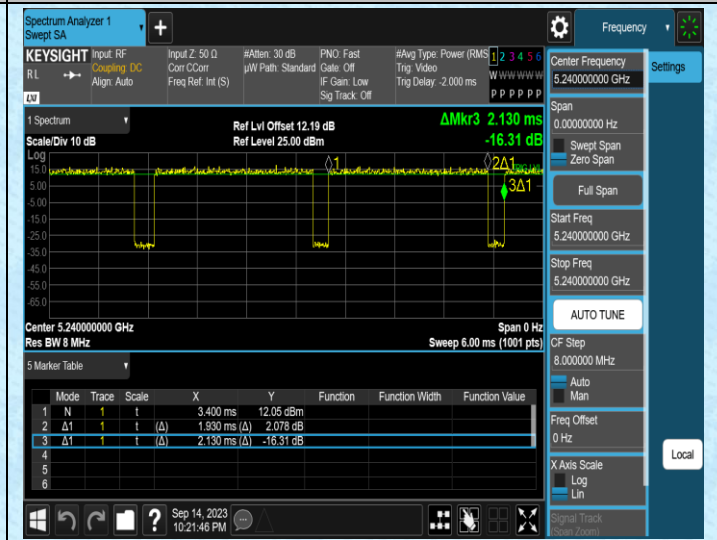
NTNV-11AC20MIMO-Ant2-5240
