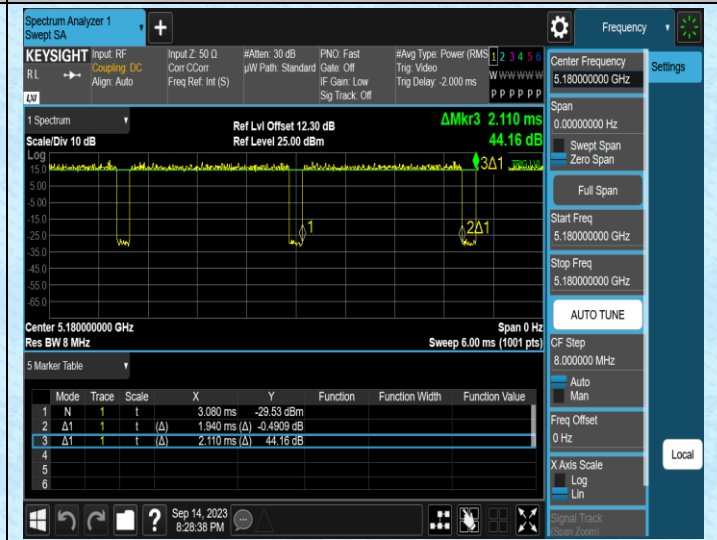
NTVN-11AC20SISO-Ant2-5180
