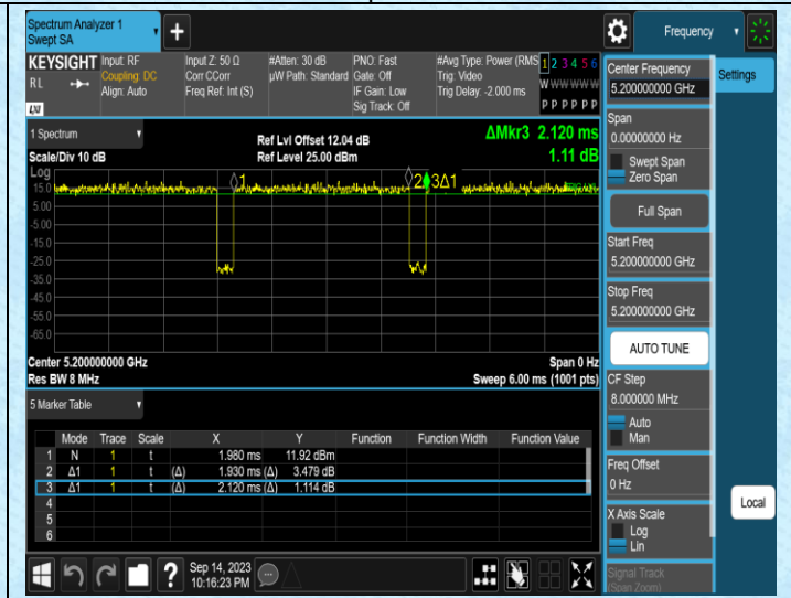
NTNV-11AC20MIMO-Ant2-5200
