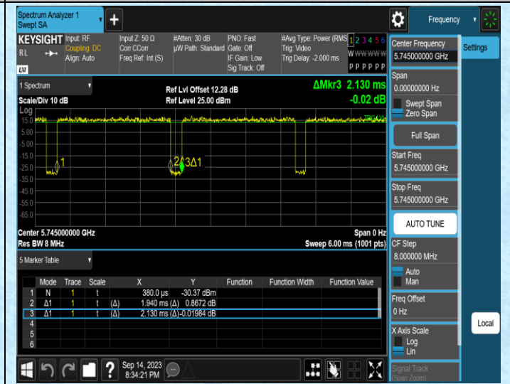
NTNV-11AC20SISO-Ant2-5745
