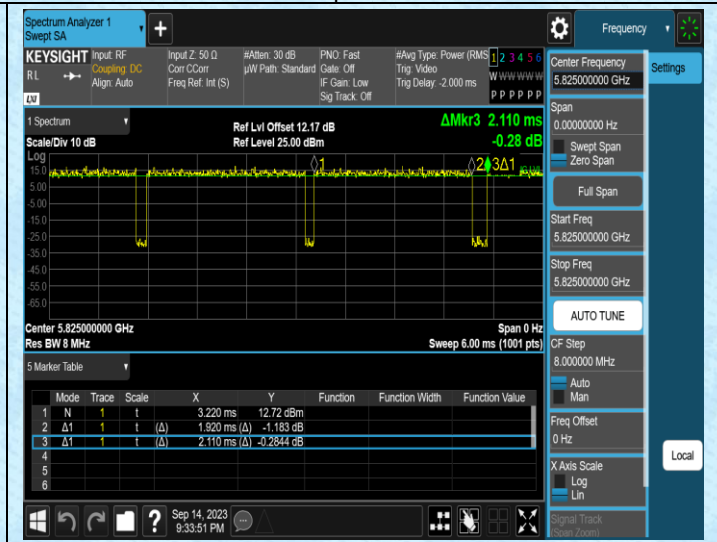
NTNV-11N20MIMO-Ant2-5825
