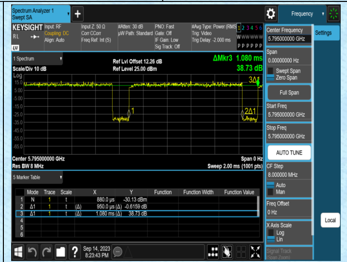
NTVN-11N40SISO-Ant2-5795
