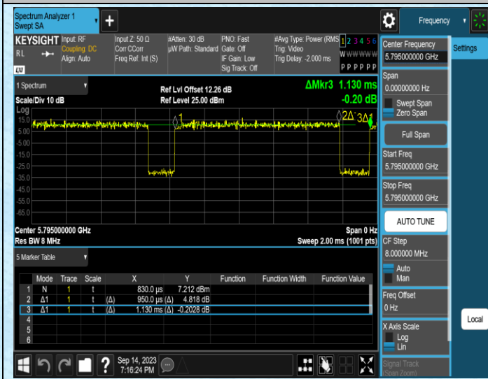
NTNV-11AC40SISO-Ant1-5795
