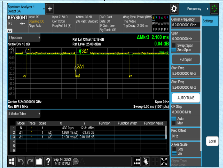
NTNV-11N20MIMO-Ant2-5240
