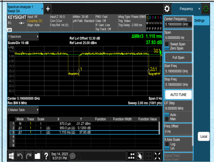
NTNV-11N40MIMO-Ant2-5190
