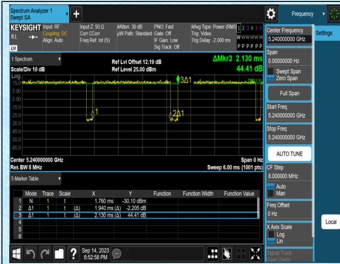
NTNV-11AC20SISO-Ant1-5240
