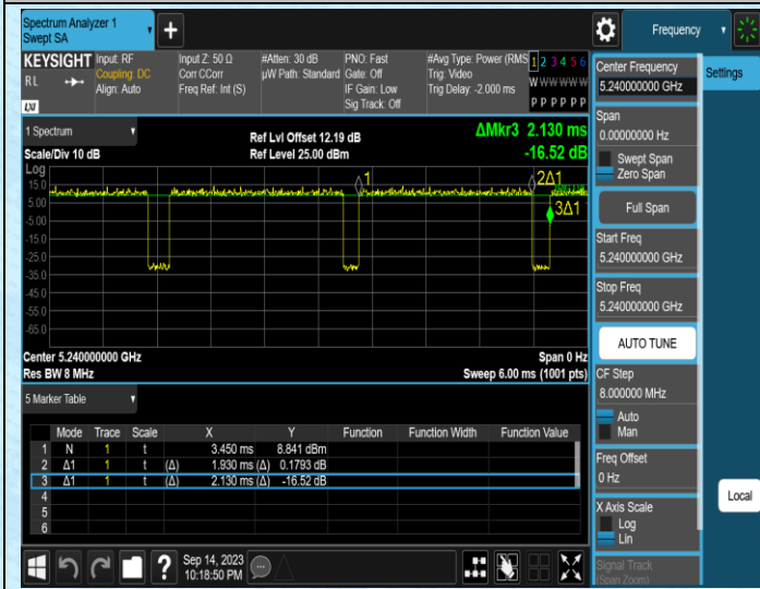
NTNV-11AC20MIMO-Ant1-5240
