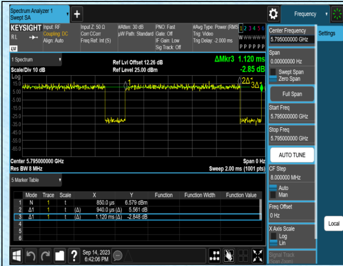
NTVN-11N40SISO-Ant1-5795
