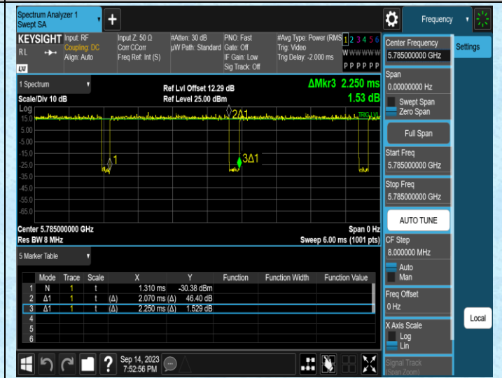
NTNV-11A-Ant2-5785
