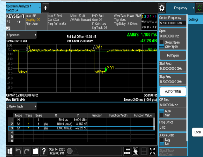
NTVN-11N40SISO-Ant1-5230
