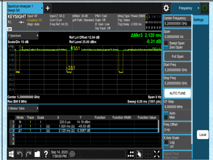
NTNV-11N20SISO-Ant2-5200
