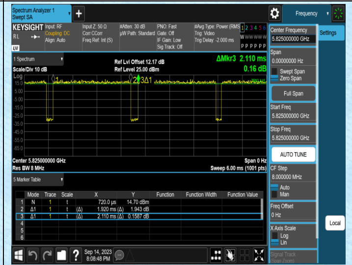
NTNV-11N20SISO-Ant2-5825
