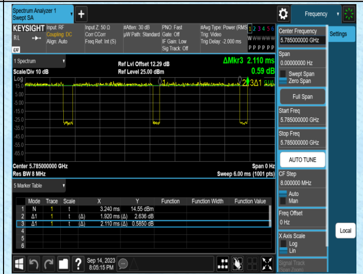
NTNV-11N20SISO-Ant2-5785
