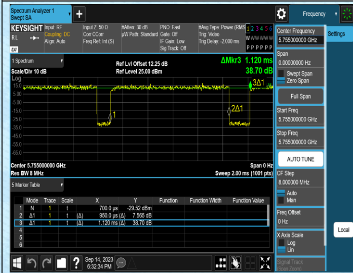
NTVN-11N40SISO-Ant1-5755
