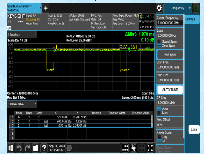
NTVN-11N40SISO-Ant2-5190
