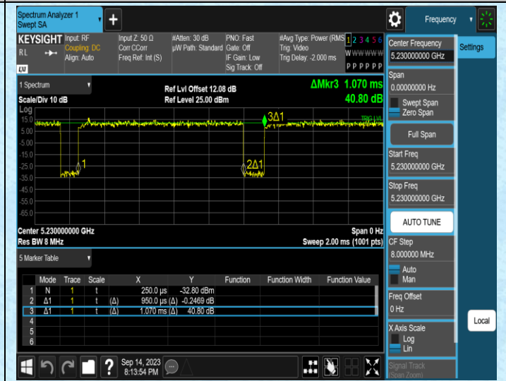
NTVN-11N40SISO-Ant2-5230
