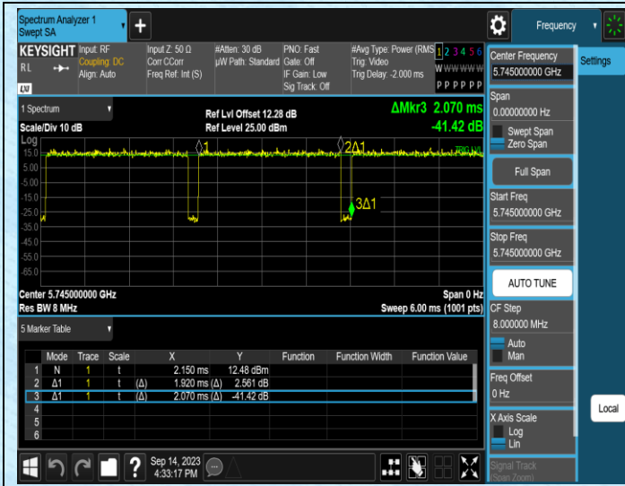
NTNV-11N20SISO-Ant1-5745
