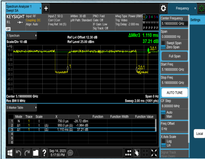
NTVN-11N40SISO-Ant1-5190
