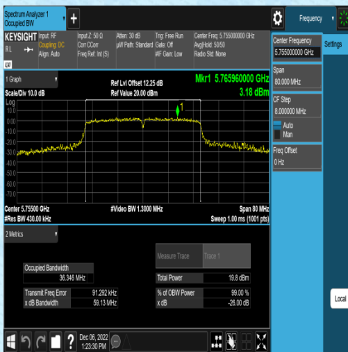
11AC40MIMO-Ant2-5755
