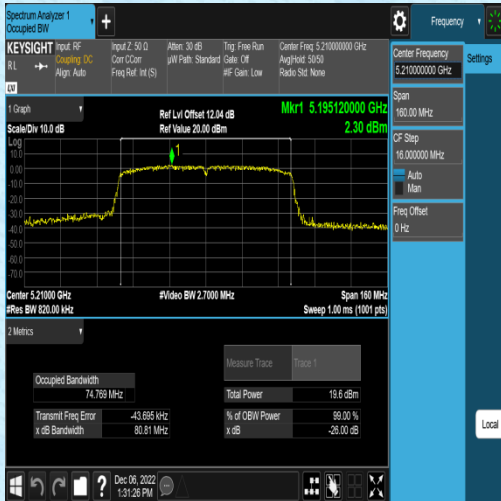
11AC80MIMO-Ant2-5210
