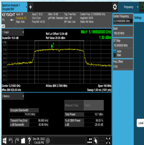
11AC80MIMO-Ant2-5210
