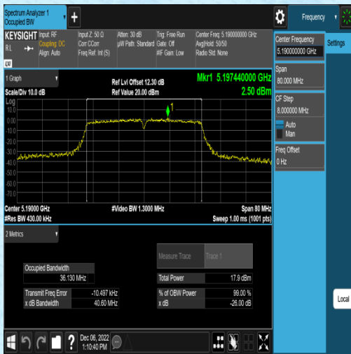
11AC40MIMO-Ant2-5190
