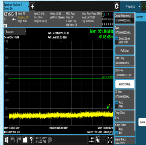
11N20MIMO-Ant2-2412-0~Reference--2.73
