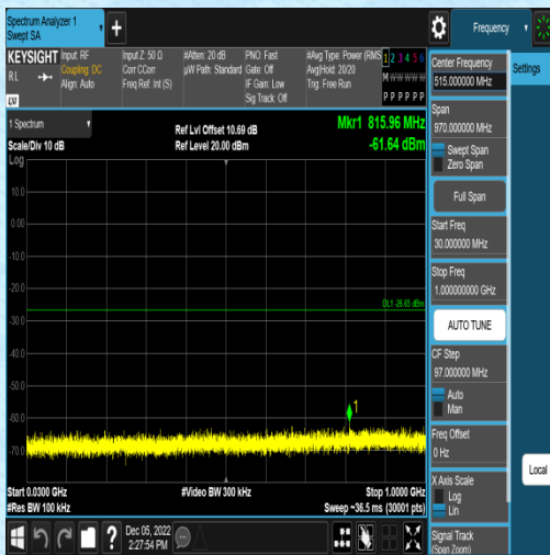
11N40MIMO-Ant1-2422-0~Reference--4.83
