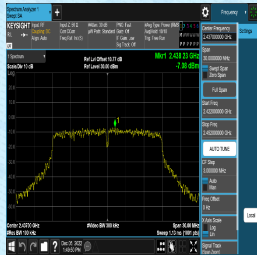
11N20SISO-Ant2-2437-1000~26500~-7.08
