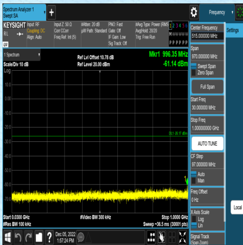
11N40SISO-Ant2-2437-0~Reference--7.81
