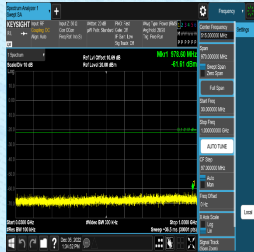
11G-Ant2-2412-0~Reference--3.62
