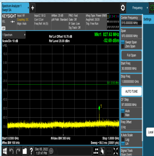
11G-Ant2-2437-0~Reference--6.22
