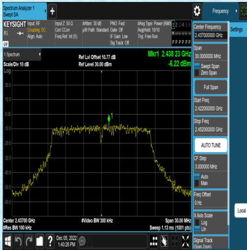
11G-Ant2-2437-1000~26500~-6.22
