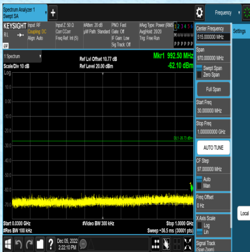
11N20MIMO-Ant1-2462-0~Reference--5.74
