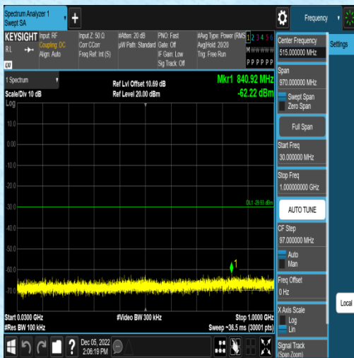
11N20MIMO-Ant1-2412-0~Reference--4.25
