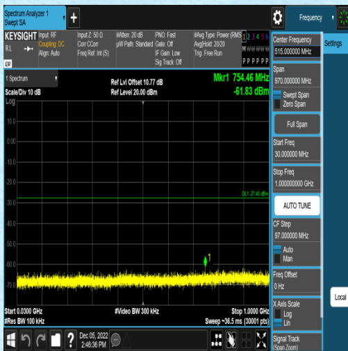
11N40MIMO-Ant1-2452-0~Reference--5.76
