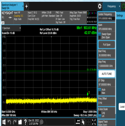
11N40MIMO-Ant1-2437-0~Reference--5.47
