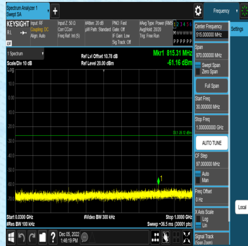
11N20SISO-Ant2-2437-0~Reference--7.08
