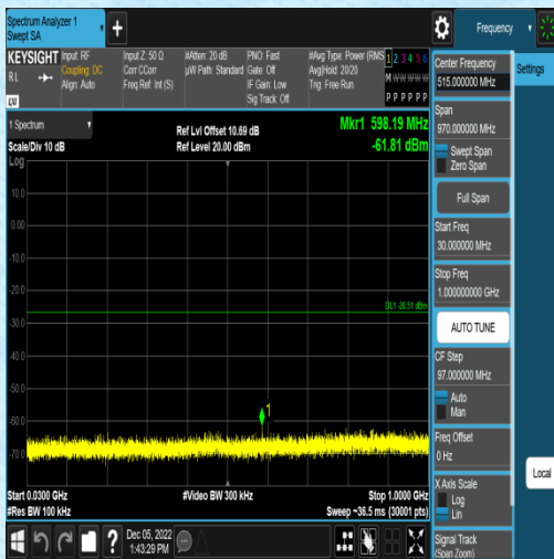
11N20SISO-Ant2-2412-0~Reference~-6.12
