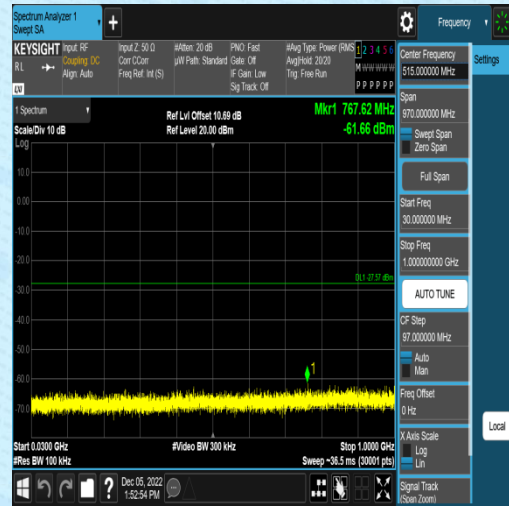
11N40SISO-Ant2-2422-0~Reference--6.17
