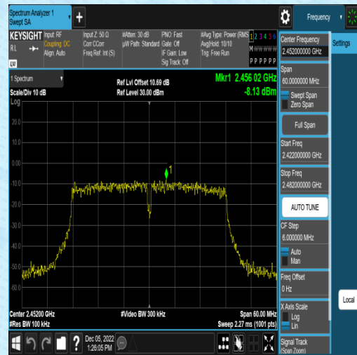
11N40SISO-Ant1-2452-1000~26500~-8.13
