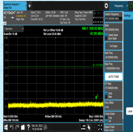
11G-Ant1-2412-0~Reference-1.94
