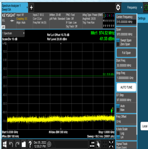
11G-Ant1-2437-0~Reference-0.85
