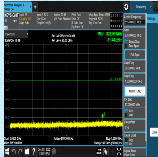
11B-Ant2-2437-0~Reference--0.28
