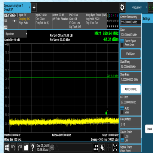
11B-Ant1-2437-0-Reference-2.24
