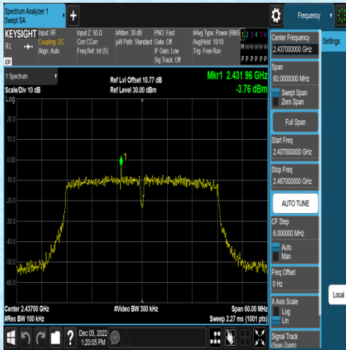
11N40SISO-Ant1-2437-1000~26500~-3.76
