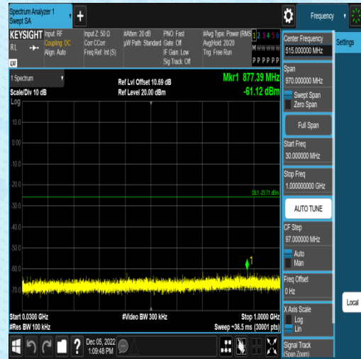
11N40SISO-Ant1-2422-0~Reference--4.16
