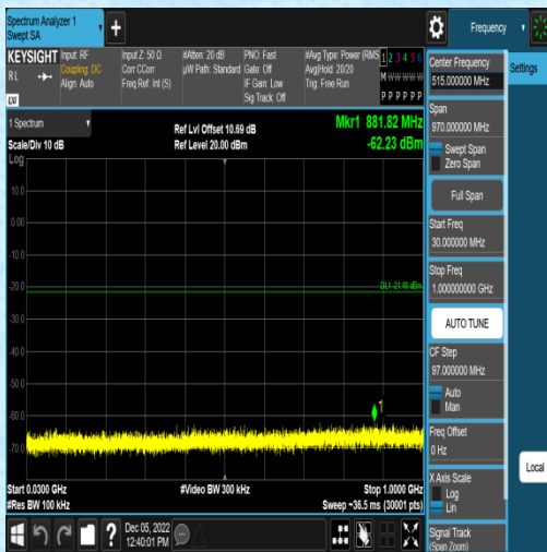
11N20SISO-Ant1-2412-0~Reference--2.37
