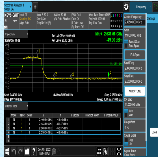
11N40SISO-Ant2-High-2452--6.20
