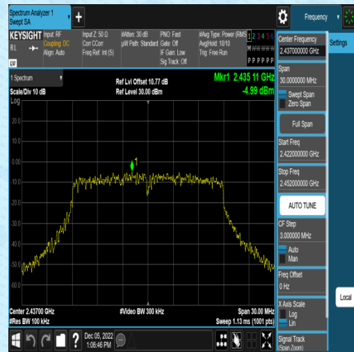
11N20SISO-Ant1-2437-1000~26500~-4.99
