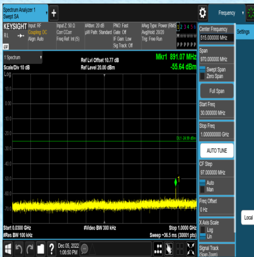
11N20SISO-Ant1-2462-0~Reference--5.71
