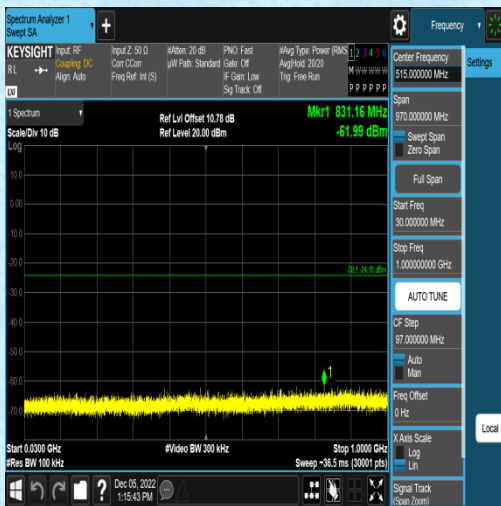
11N40SISO-Ant1-2437-0~Reference--3.76
