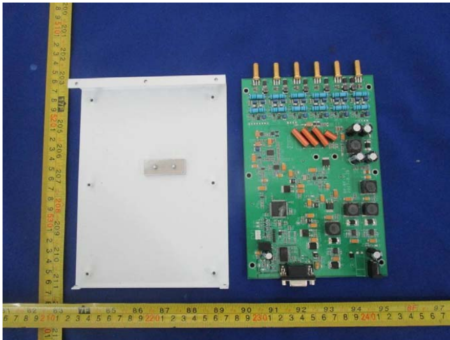
EUT – Signal Box Uncover View
