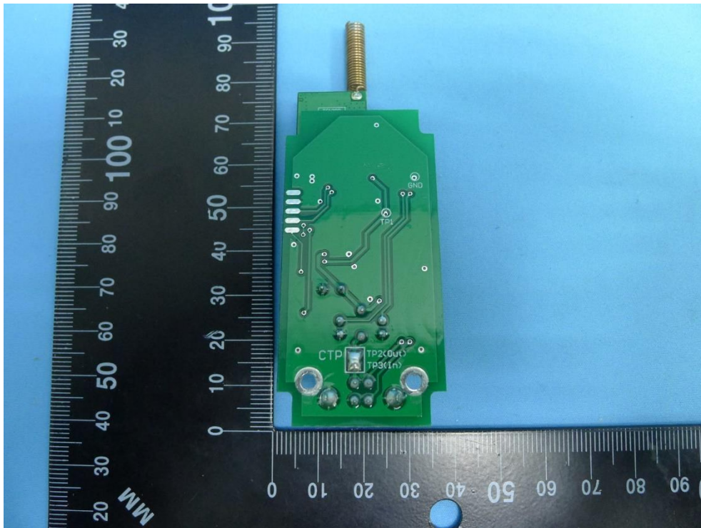
(22) Host Photo (RFD)
