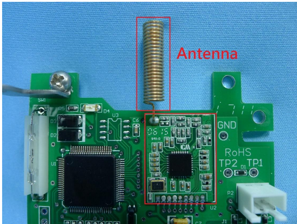
(2) EUT Photo (434MHz RF Module)
