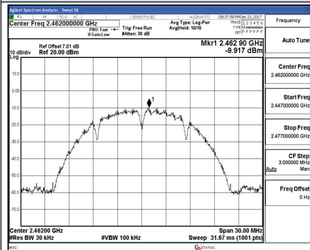
Channel 11 / 2462 MHz
