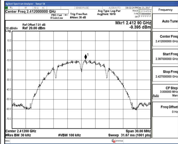
Channel 1 / 2412 MHz
