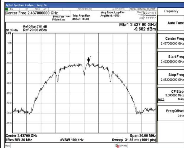
Channel 6 / 2437 MHz
