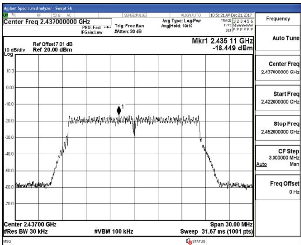
Channel 6 / 2437 MHz
