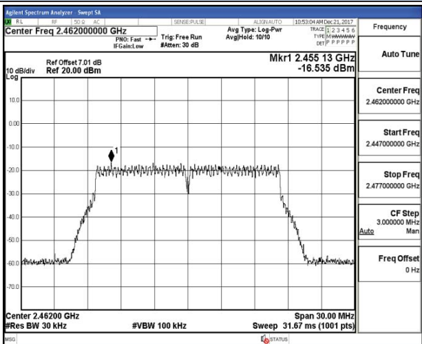
Channel 11 / 2462 MHz
