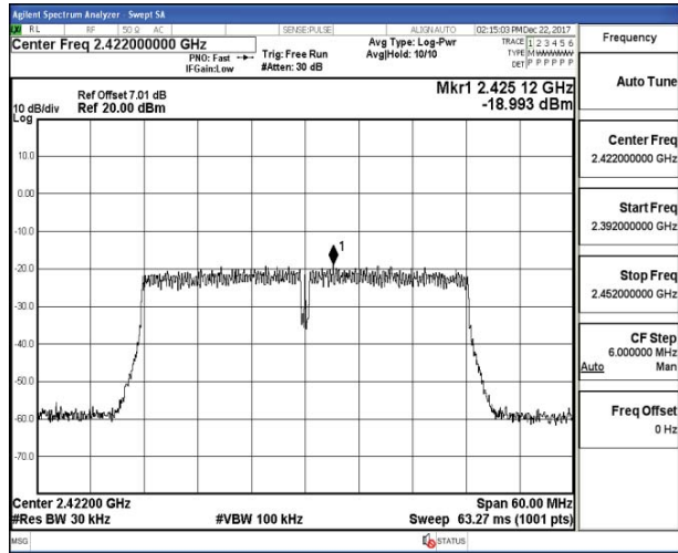
Channel 3 / 2422 MHz
