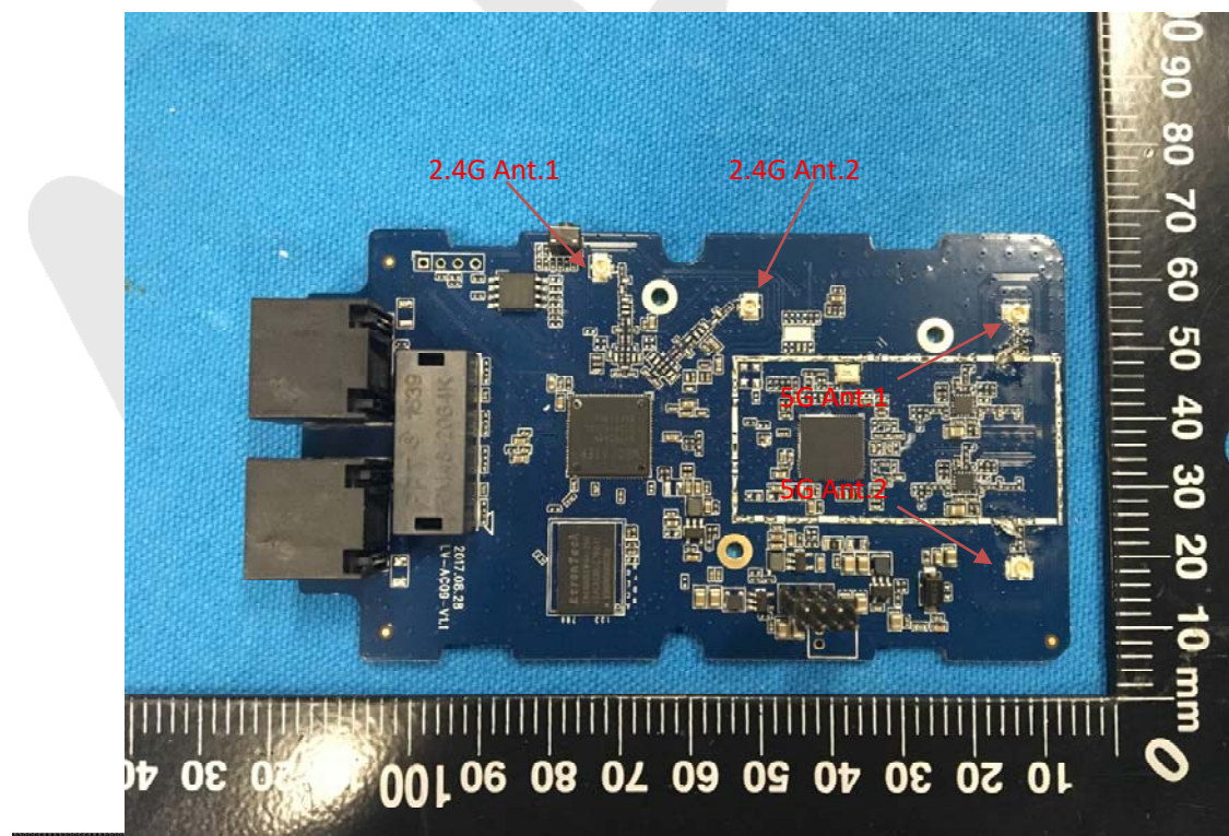
WIFI Antenna
