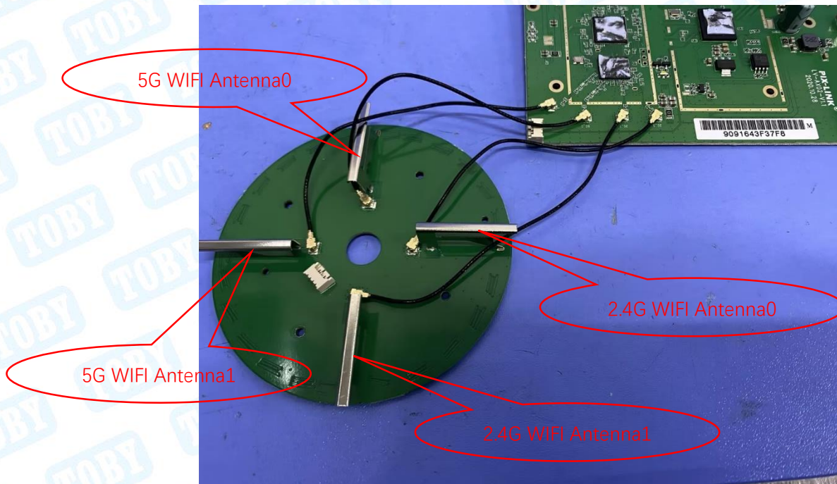
Photo 14 Internal of PCB
