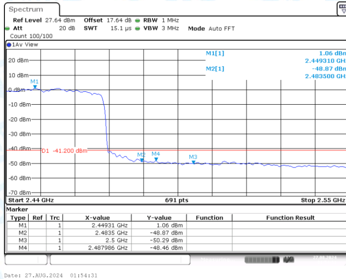
11AX40MIMO_Ant0_High_2452_Peak
