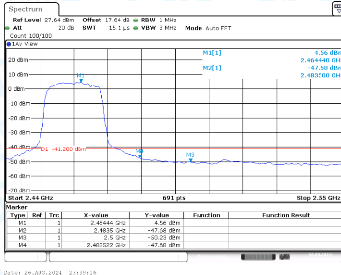
11N20MIMO_Ant0_High_2462_Peak
