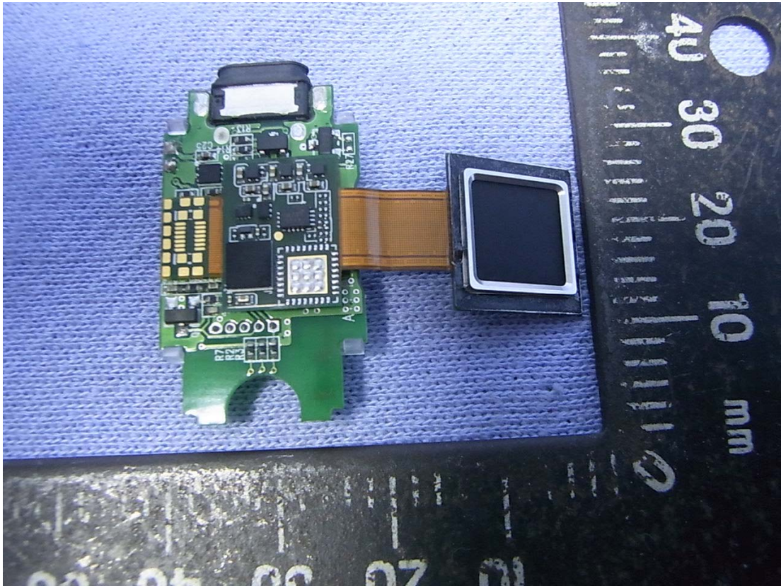
Figure 8 Internal View (Main Board/Back View, Touch Board/Front View)
