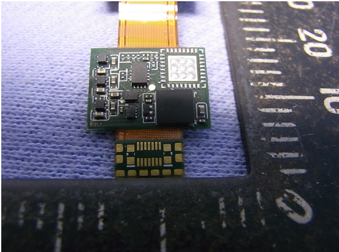
Figure 9 Internal View (Internal Board, Front View)
