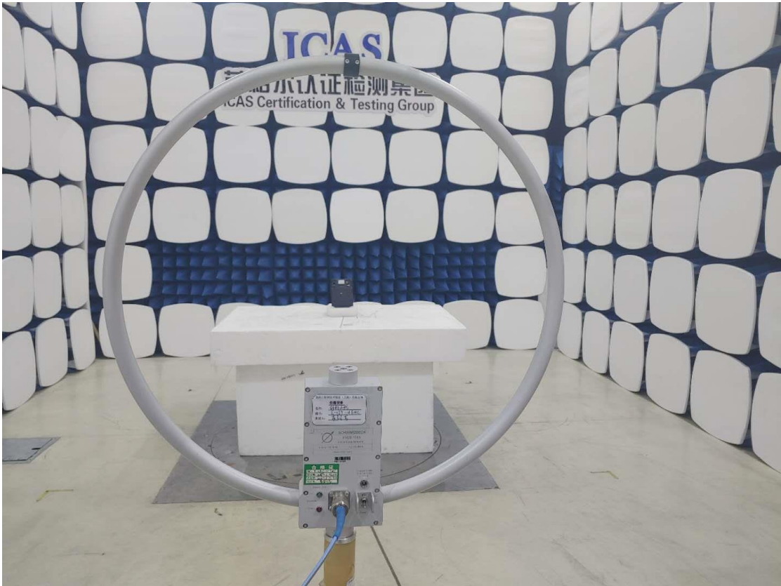
NFC test setup
