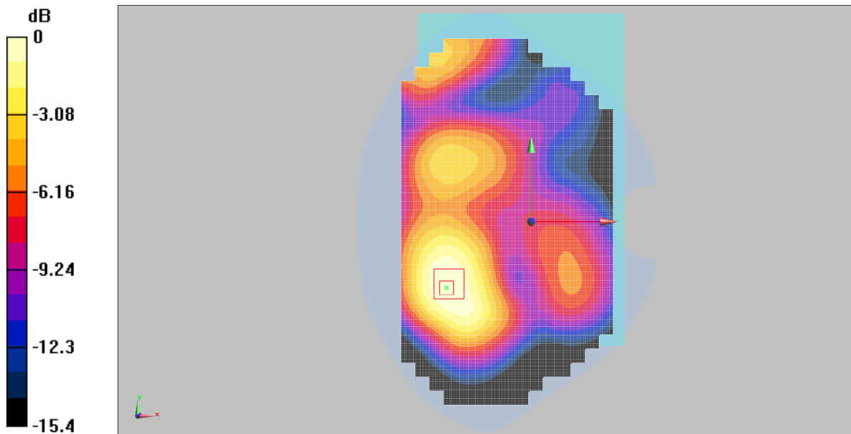
0 dB = 0.386W/Kg
