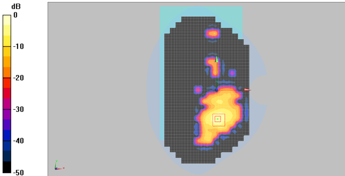
0 dB = 0.728W/Kg
