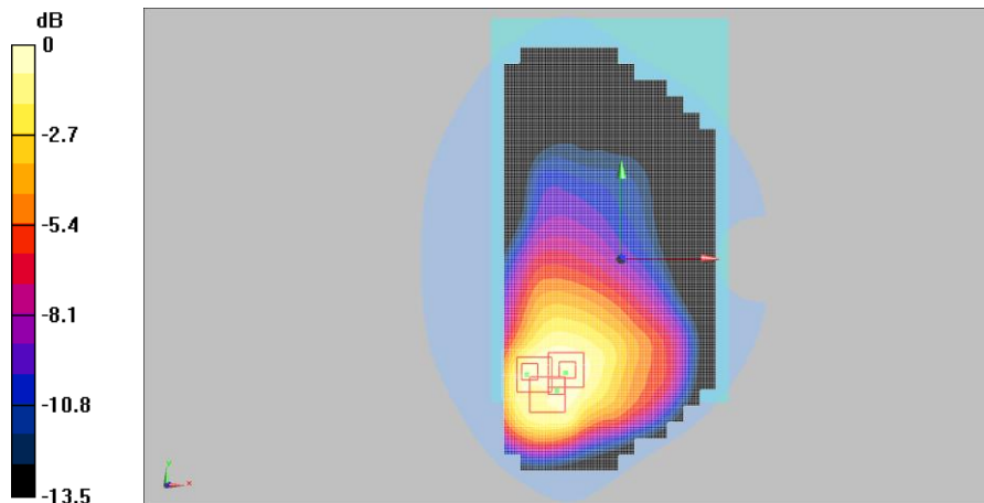
0 dB = 0.756W/Kg
