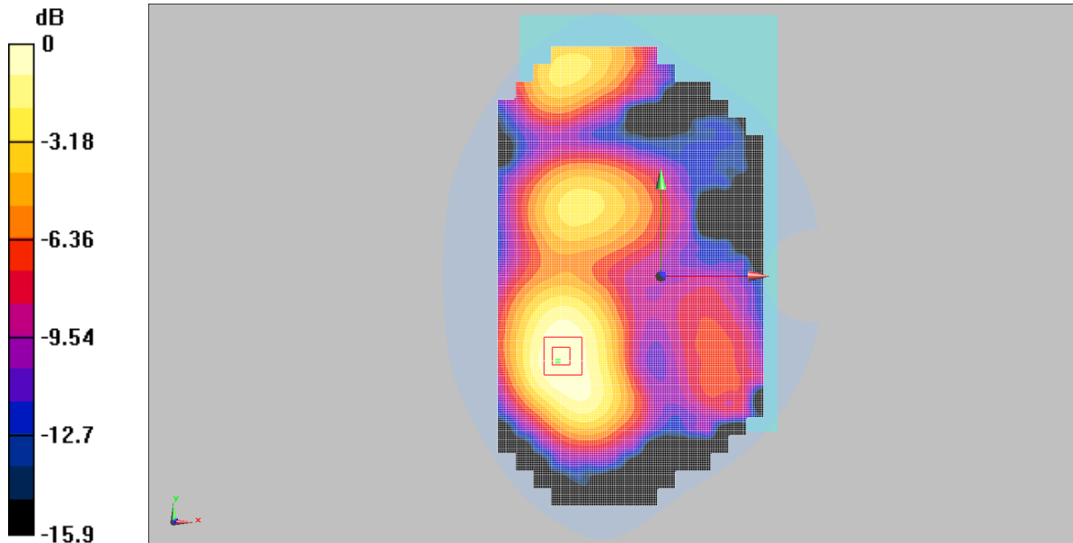
0 dB = 0.118W/Kg
