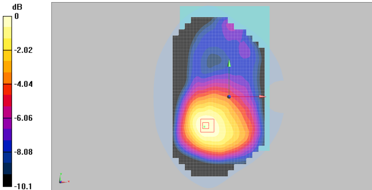
0 dB = 0.335W/Kg
