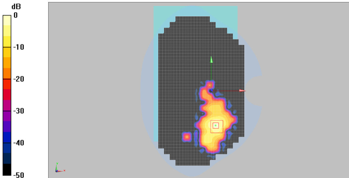
0 dB = 0.707W/Kg
