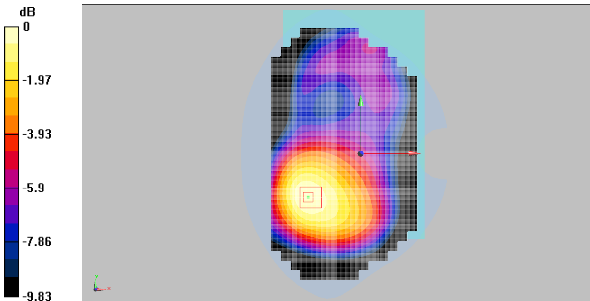
0 dB = 0.236W/Kg
