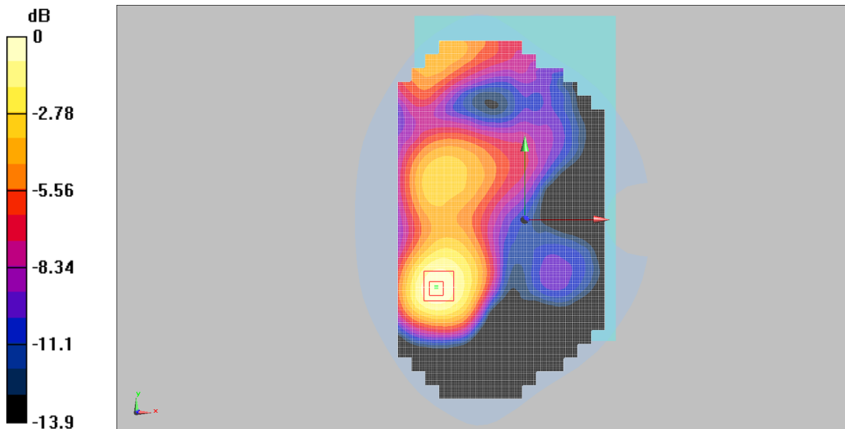
0 dB = 0.241W/Kg
