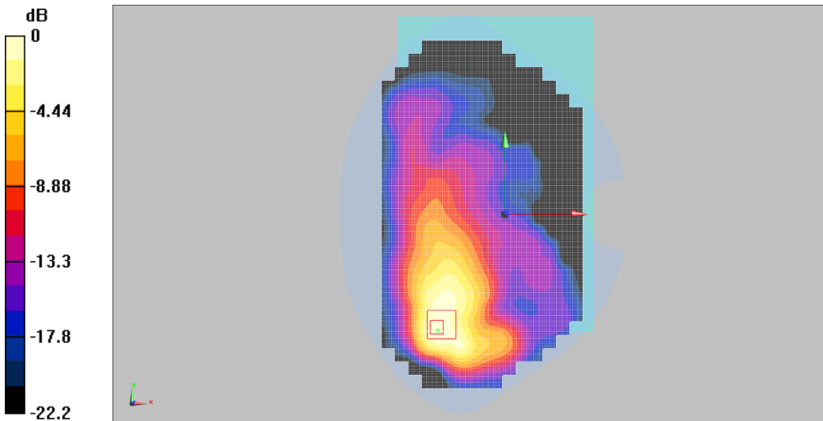
0 dB = 0.452W/Kg
