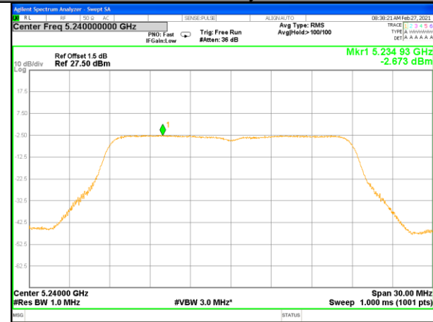
W52_11ac20_Higher_Power Spectrum Density
