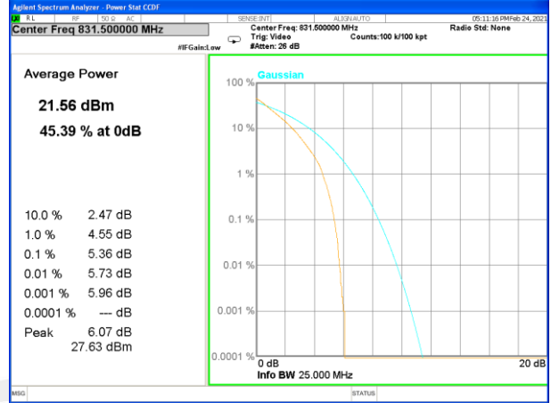
Band 26_75_Q16_Low
