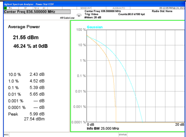
Band 26_75_QPSK_Middle
