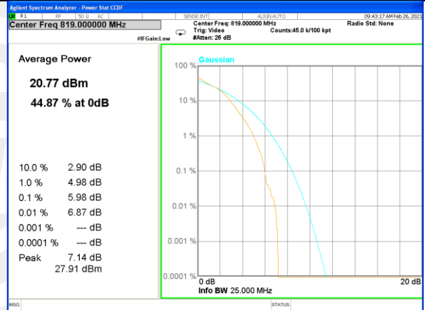
Band 26_50_Q16_Middle
