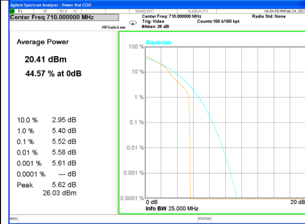
Band 17_1_QPSK_High
