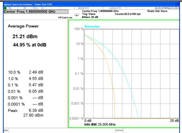
Band 2_100_QPSK_Middle
