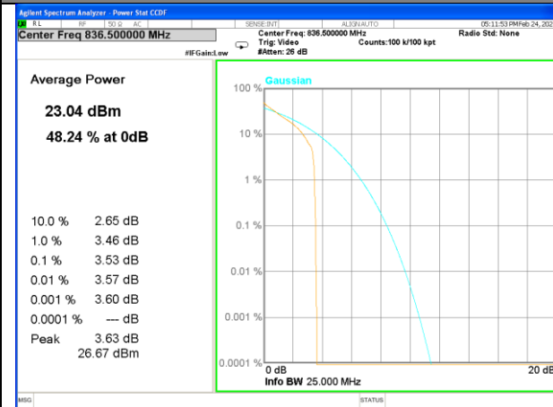
Band 26_1_QPSK_Middle
