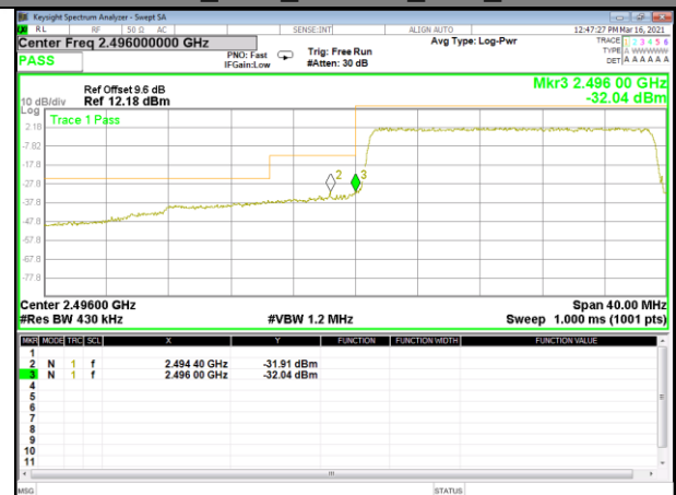
Band 41_20M_16QAM_Low_Full-RB
