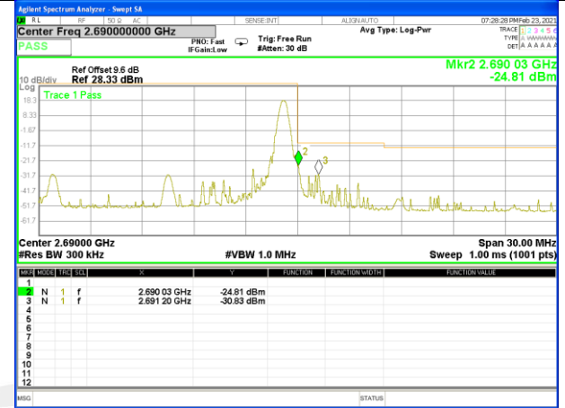
Band 41_15M_QPSK_High_Full-RB
