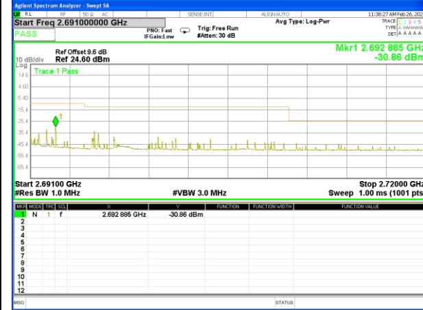
Band 41_20M_16QAM_High_Full-RB
