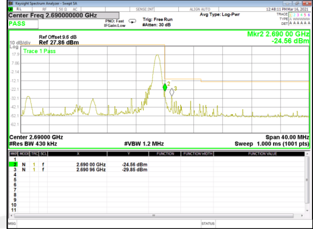
Band 41_20M_16QAM_High_Full-RB
