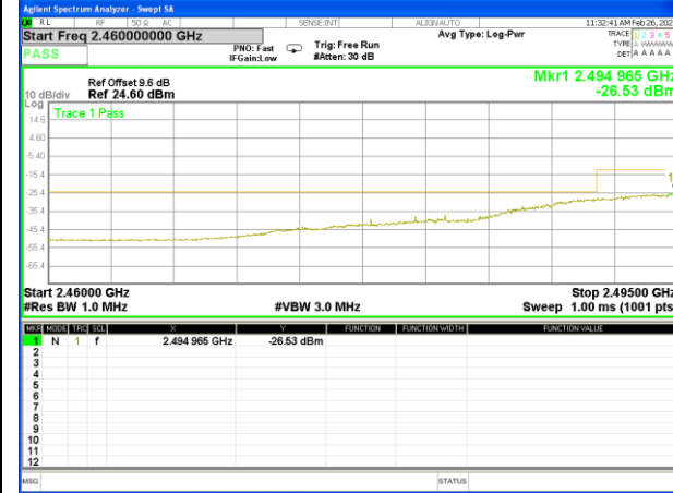
Band 41_15M_16QAM_High_1-RB
