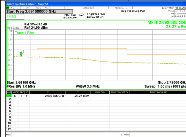
Band 41_20M_16QAM_High_Full-RB
