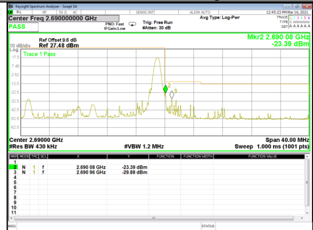
Band 41_20M_QPSK_High_1-RB
