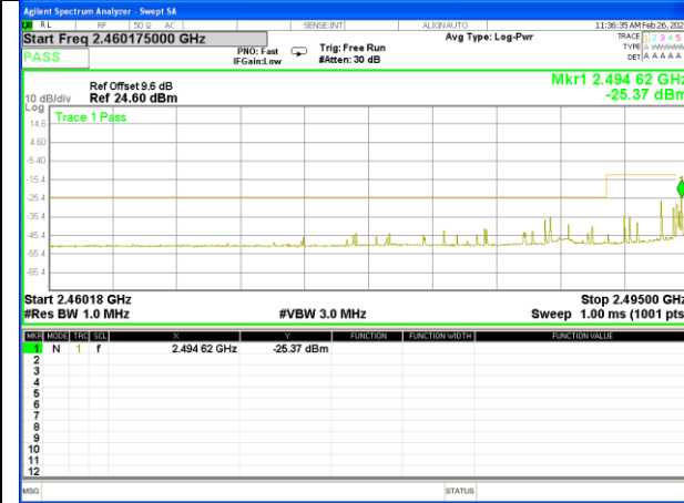
Band 41_20M_QPSK_Low_Full-RB
