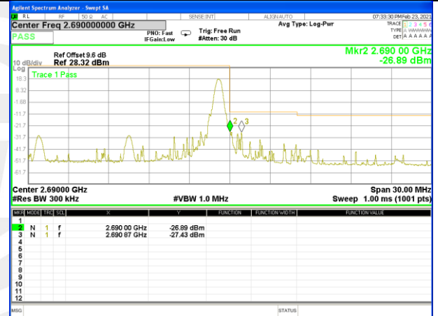
Band 41_15M_16QAM_High_Full-RB
