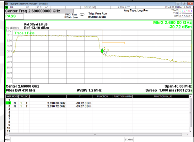
Band 41_20M_16QAM_High_Full-RB
