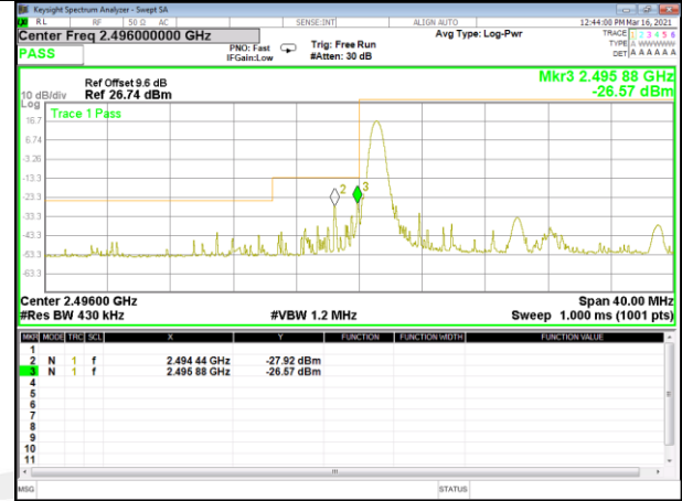
Band 41_20M_QPSK_Low_Full-RB
