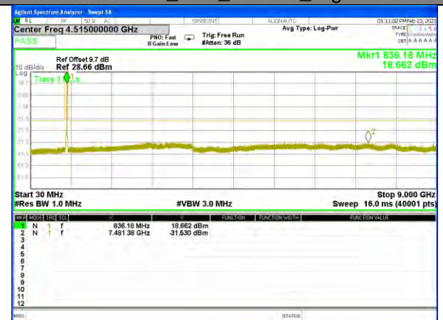
Band26_15M_16QAM_High
