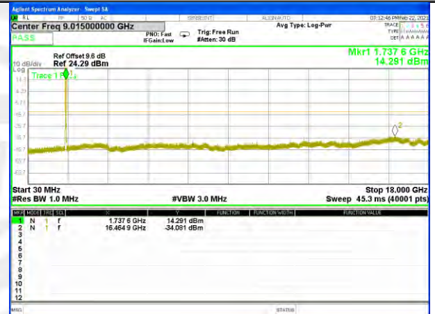
Band4_20M_16QAM_High
