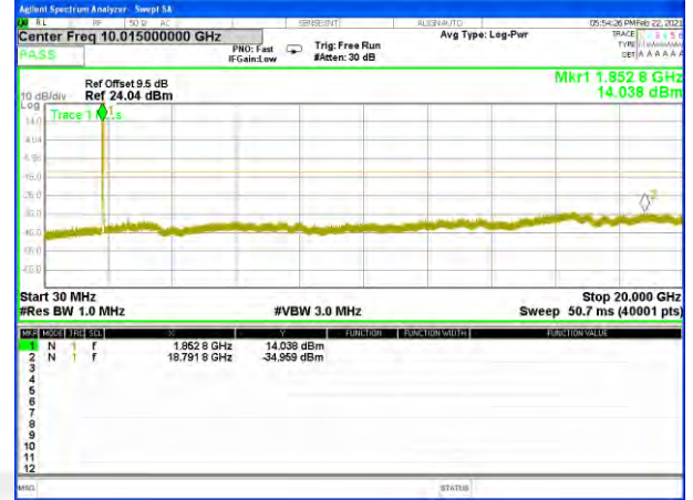
Band2_20M_16QAM_Middle
