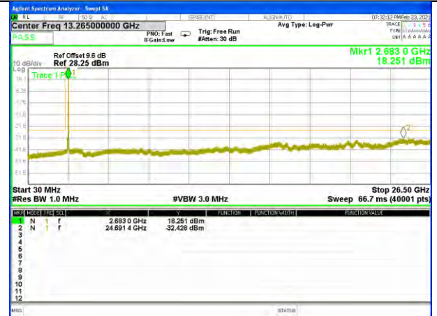
Band41_15M_16QAM_High
