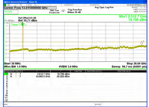
Band7_15M_16QAM_Middle
