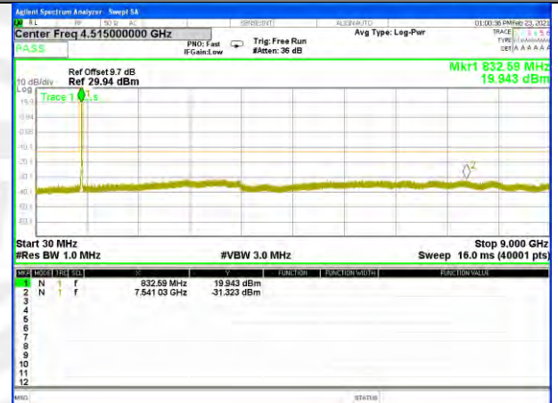
Band26_10M_16QAM_High
