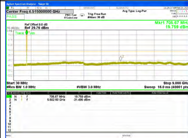
Band12_10M_QPSK_High
