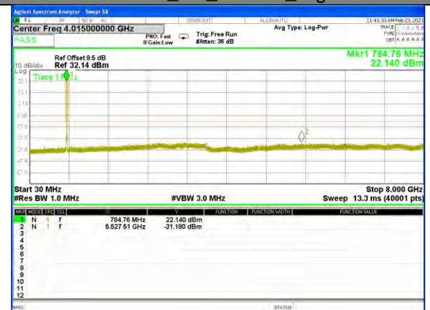
Band13_5M_16QAM_High
