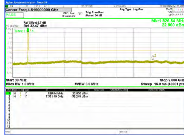
Band26_3M_QPSK_Middle
