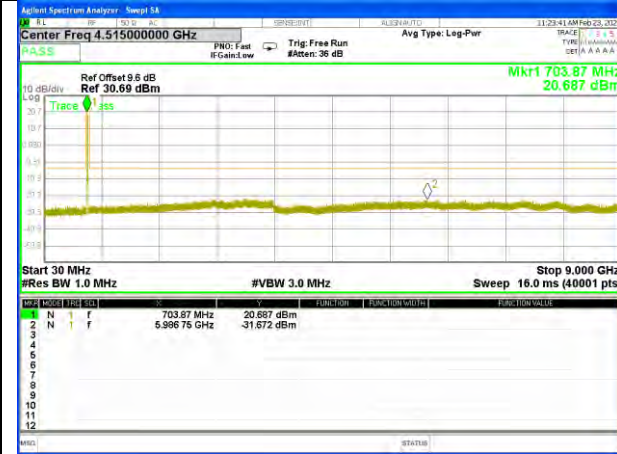
Band12_10M_QPSK_Middle
