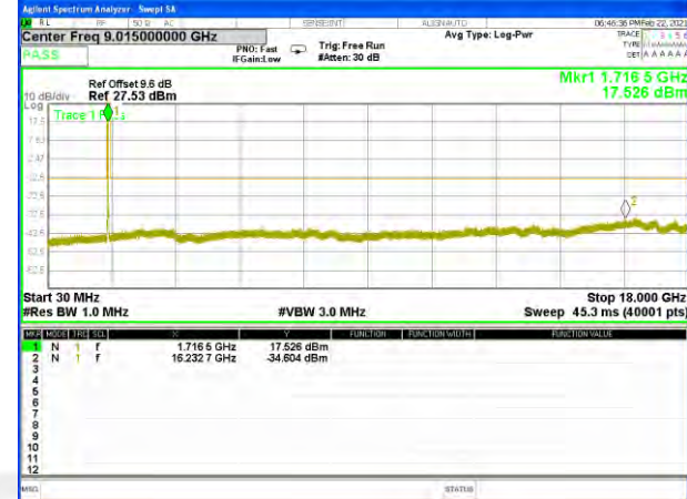
Band4_10M_16QAM_Middle
