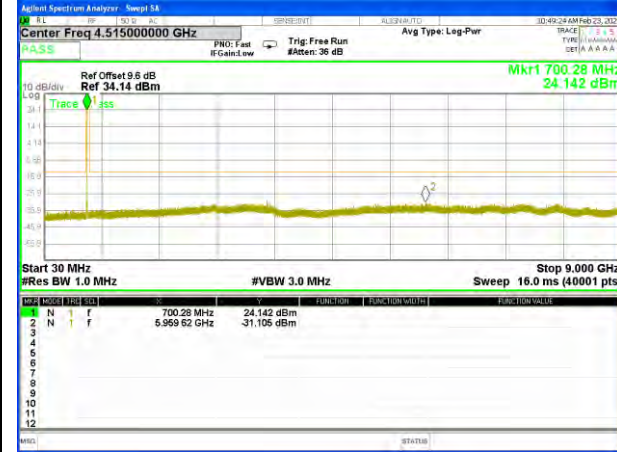
Band12_1.4M_QPSK_Middle
