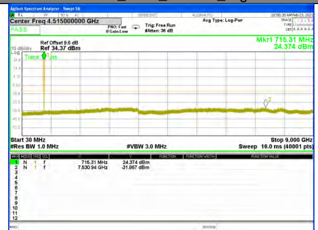
Band12_1.4M_16QAM_High
