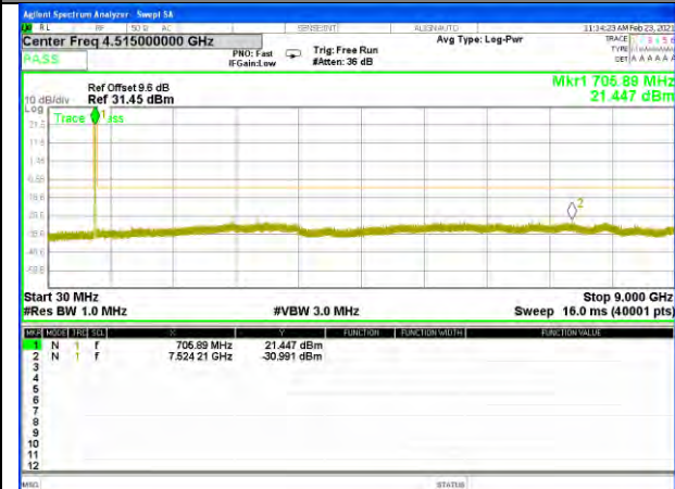
Band12_5M_QPSK_High
