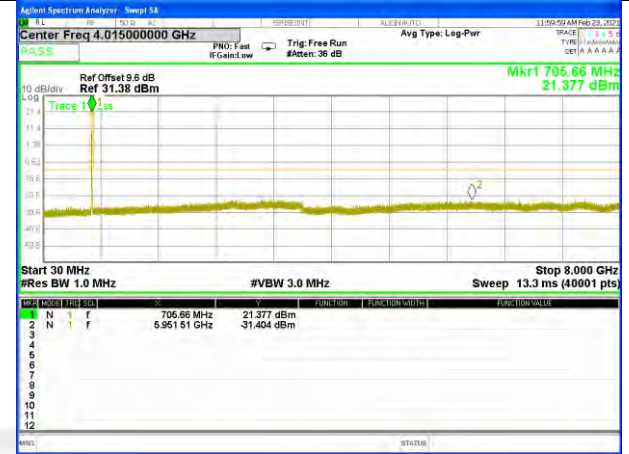
Band17_5M_16QAM_Middle
