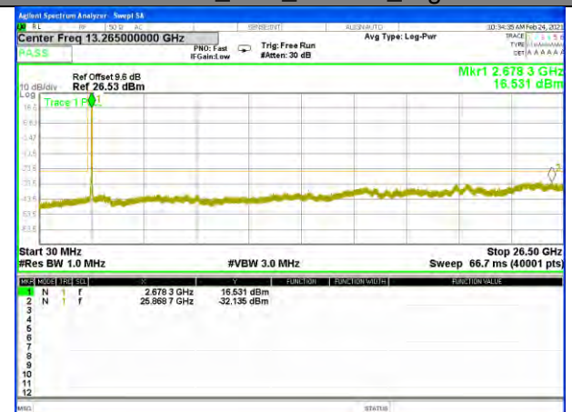
Band41_20M_16QAM_High
