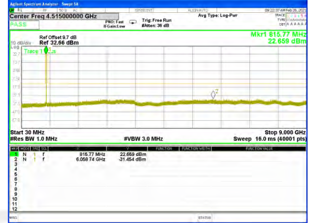
Band26_3M_16QAM_Middle
