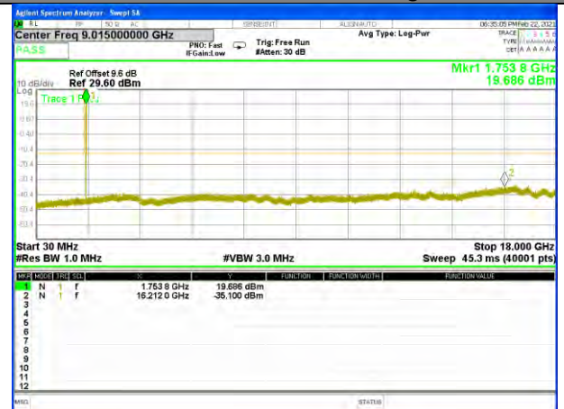
Band4_5M_16QAM_High
