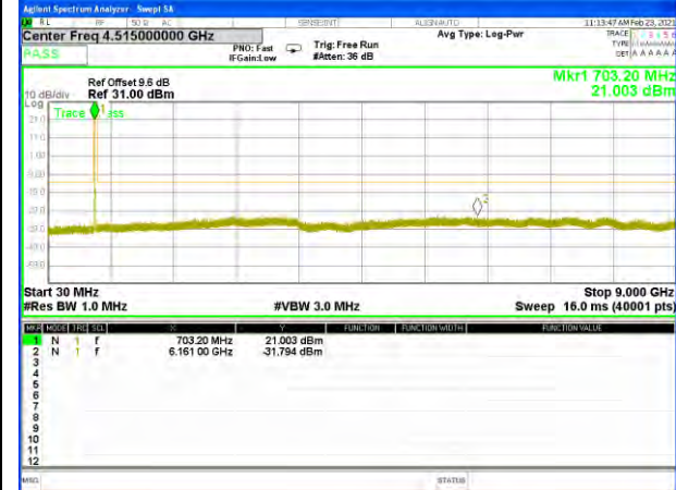
Band12_5M_QPSK_Middle
