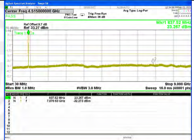
Band26_3M_16QAM_High
