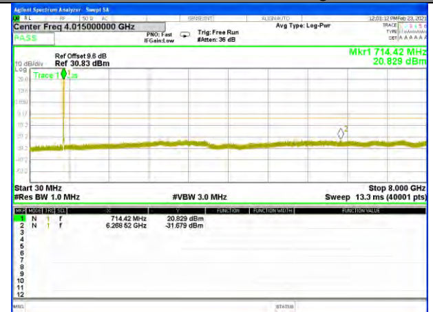
Band17_5M_16QAM_High
