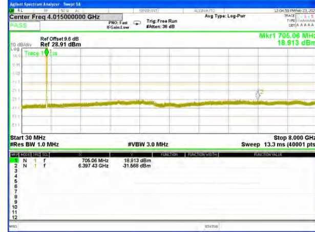
Band17_10M_QPSK_Middle
