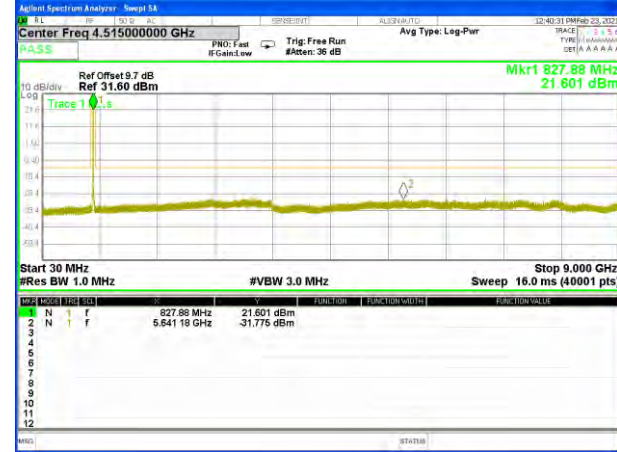
Band26_5M_QPSK_Middle
