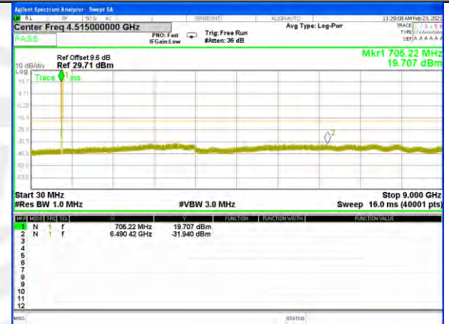
Band12_10M_16QAM_High
