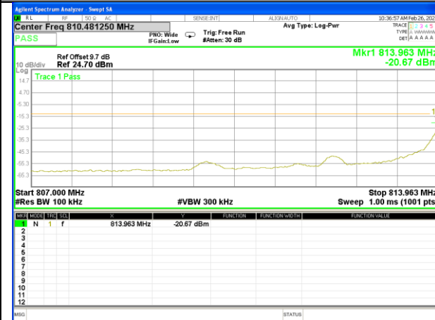
Band 26_5M_QPSK_Low_Full-RB
