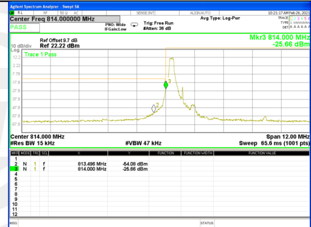
Band 26_1.4M_16QAM_Low_Full-RB
