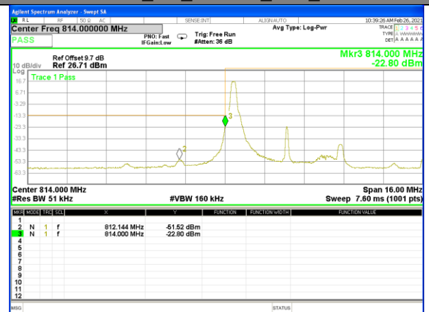
Band 26_5M_16QAM_Low_1-RB
