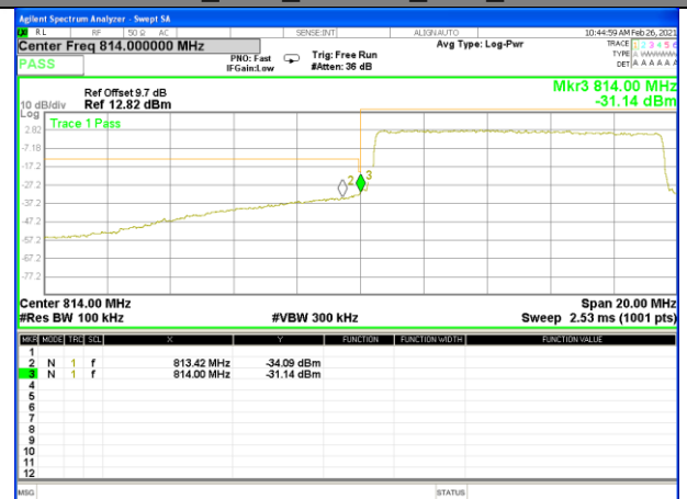
Band 26_10M_16QAM_Low_Full-RB
