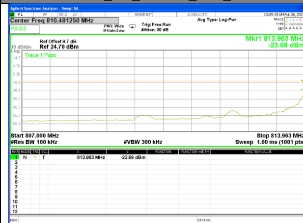
Band 26_5M_16QAM_Low_1-RB
