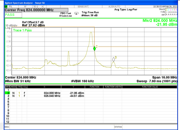
Band 26_5M_QPSK_High_Full-RB
