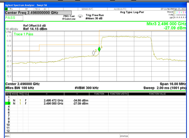
Band 41_5M_16QAM_Low_Full-RB
