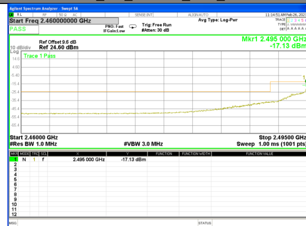
Band 41_5M_16QAM_Low_Full-RB
