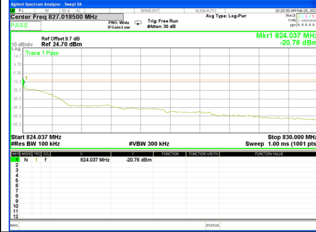
Band 26_1.4M_16QAM_Low_1-RB
