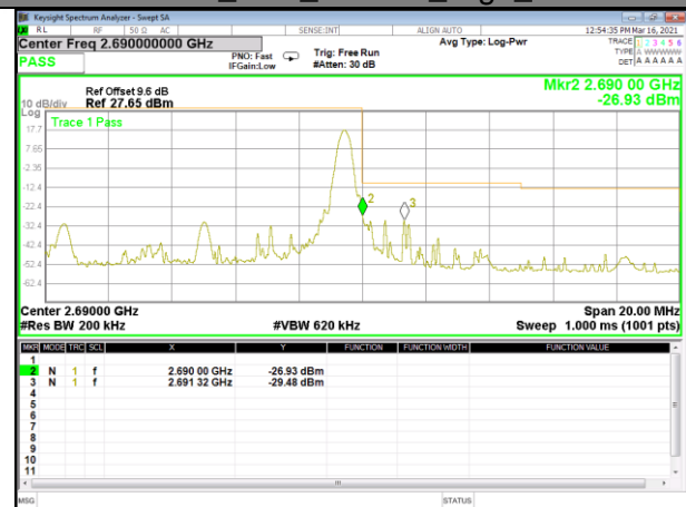
Band 41_10M_16QAM_High_1-RB
