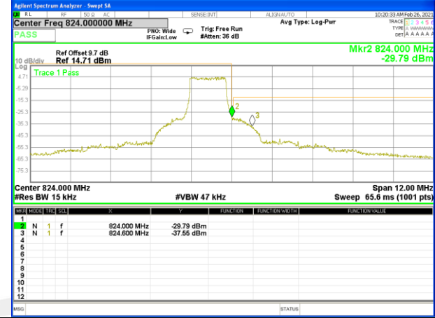
Band 26_1.4M_16QAM_Low_1-RB
