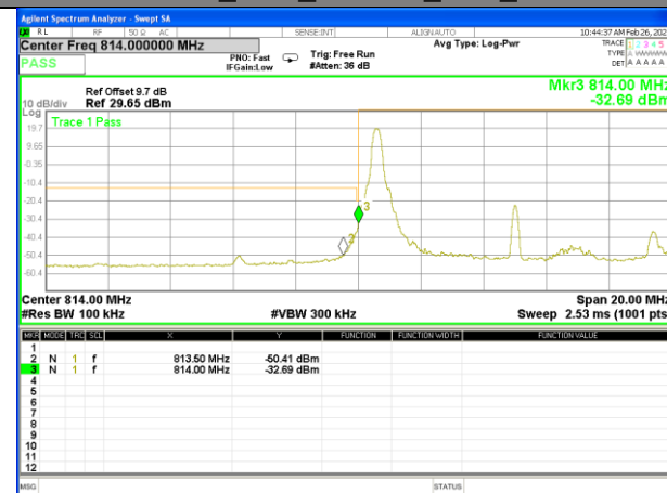
Band 26_10M_16QAM_Low_1-RB
