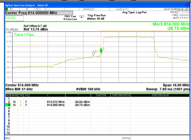
Band 26_5M_QPSK_Low_Full-RB
