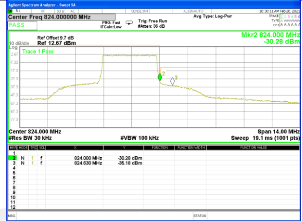
Band 26_5M_QPSK_Low_1-RB
