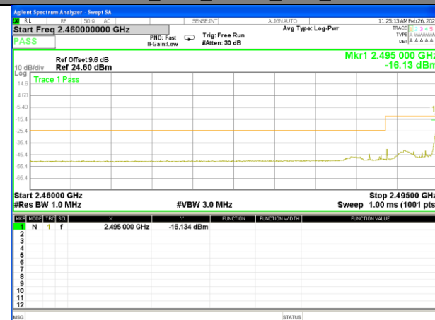
Band 41_10M_QPSK_Low_1-RB
