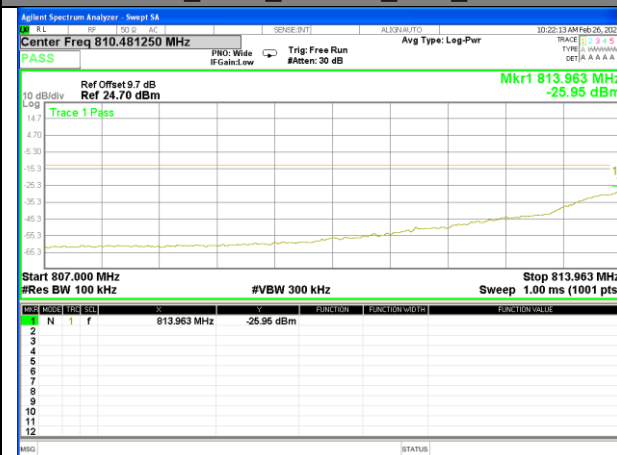
Band 26_1.4M_16QAM_Low_Full-RB
