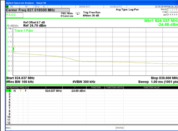
Band 26_5M_QPSK_Low_1-RB
