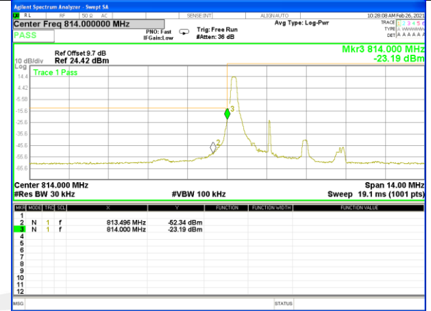
Band 26_3M_16QAM_Low_Full-RB
