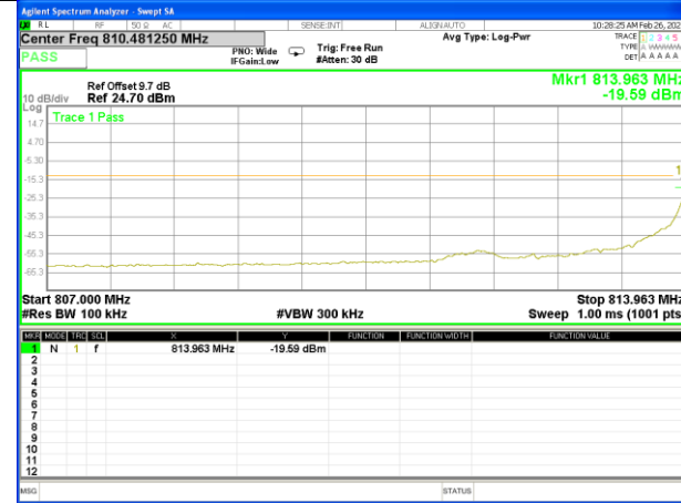
Band 26_3M_16QAM_Low_Full-RB
