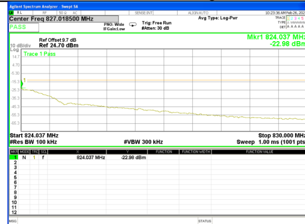
Band 26_3M_QPSK_Low_1-RB
