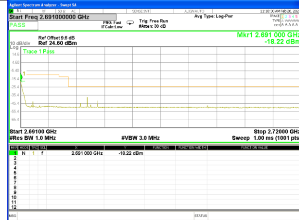
Band 41_5M_16QAM_High_Full-RB
