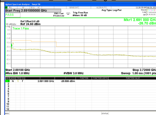
Band 41_10M_QPSK_High_Full-RB
