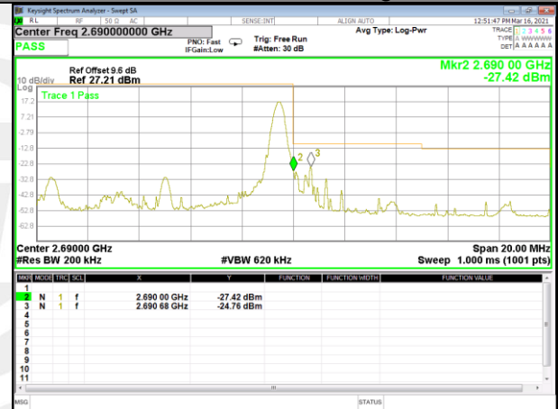
Band 41_10M_QPSK_High_Full-RB
