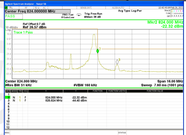
Band 26_5M_16QAM_High_Full-RB
