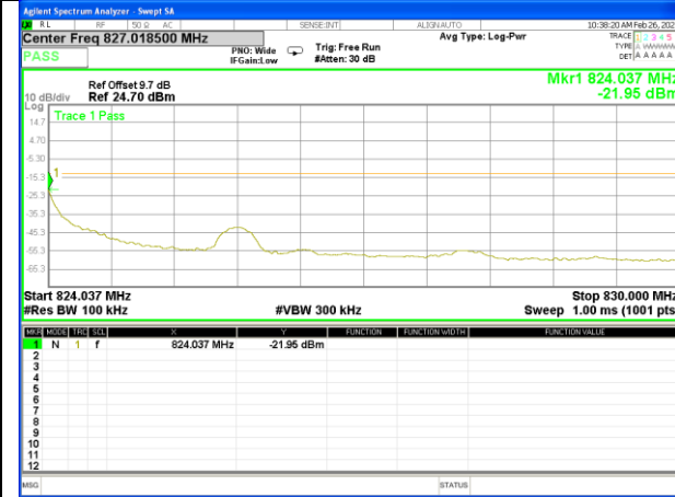
Band 26_5M_QPSK_High_Full-RB
