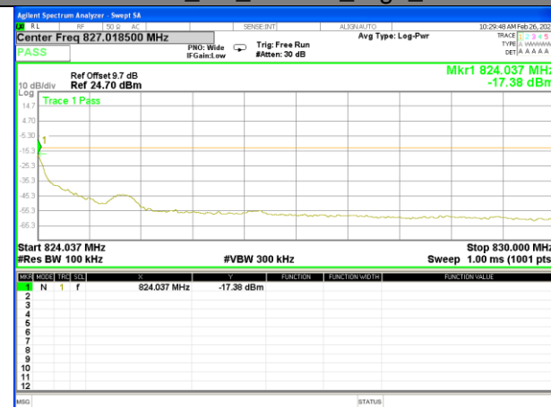
Band 26_3M_16QAM_High_1-RB
