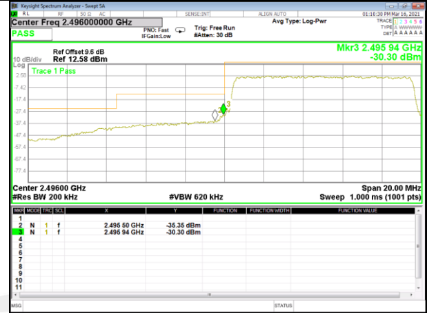
Band 41_10M_QPSK_High_1-RB
