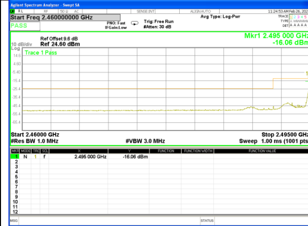
Band 41_10M_16QAM_Low_Full-RB
