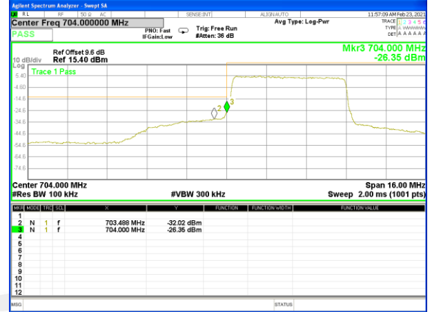
Band17_5M_QPSK_High_Full-RB
