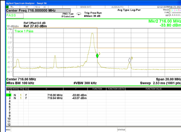
Band17_10M_16QAM_High_1-RB
