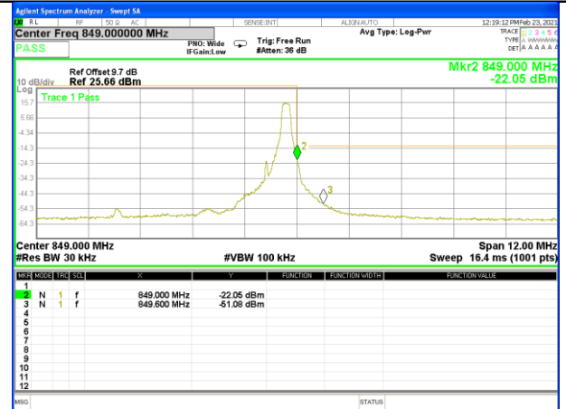
Band26_1.4M_QPSK_High_1-RB
