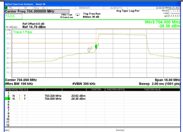
Band17_5M_16QAM_Low_Full-RB
