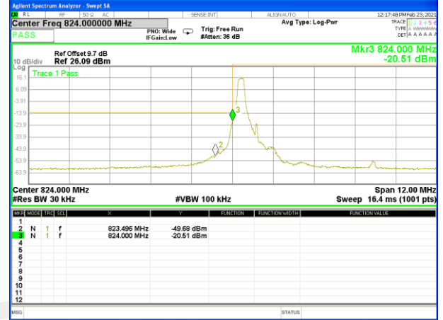
Band26_1.4M_QPSK_Low_Full-RB
