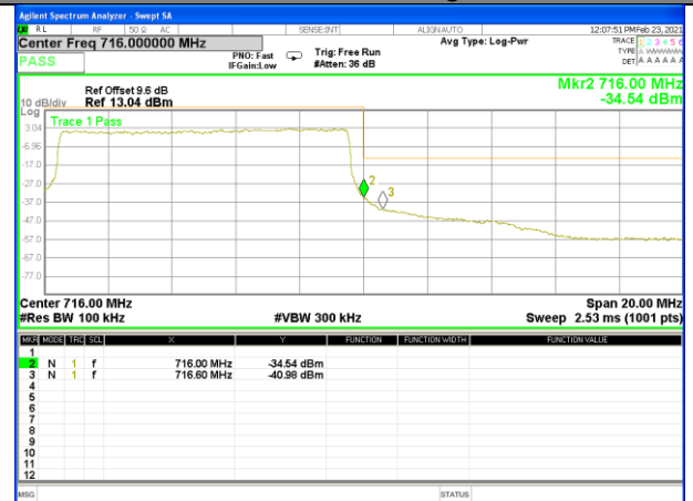
Band17_10M_QPSK_High_Full-RB
