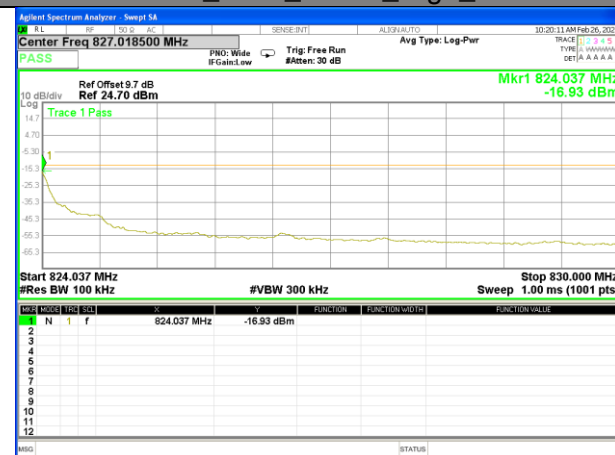
Band 26_1.4M_QPSK_High_1-RB
