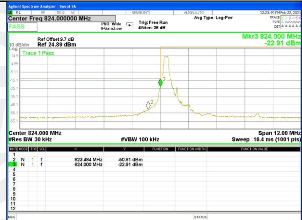
Band26_1.4M_16QAM_Low_Full-RB
