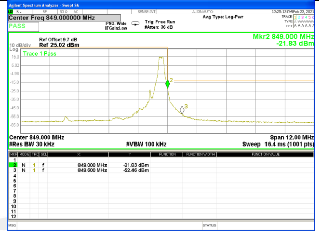
Band26_1.4M_16QAM_High_Full-RB
