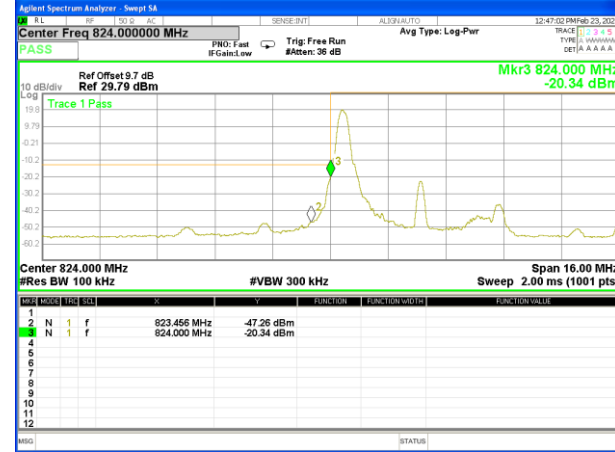
Band26_5M_16QAM_High_1-RB
