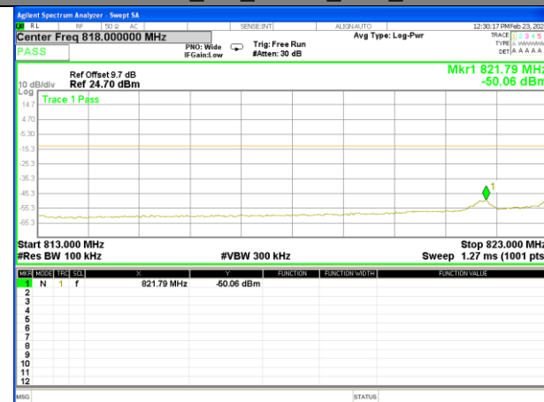
Band26_3M_QPSK_Low_1-RB
