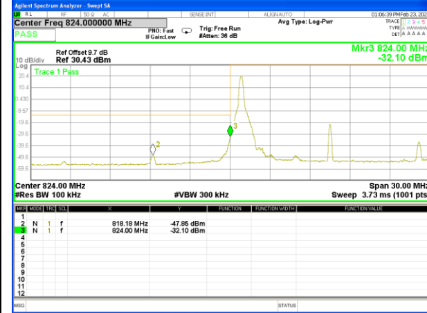
Band26_15M_QPSK_High_1-RB
