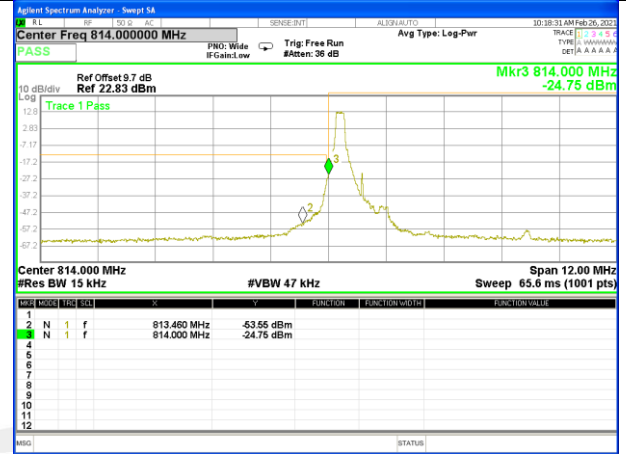
Band 26_1.4M_QPSK_Low_Full-RB
