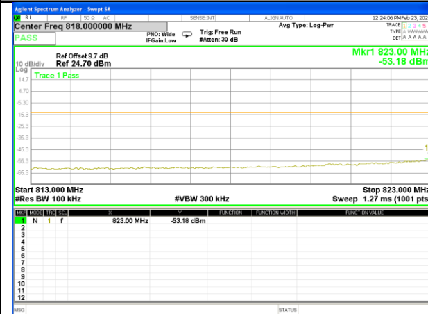
Band26_1.4M_16QAM_Low_Full-RB
