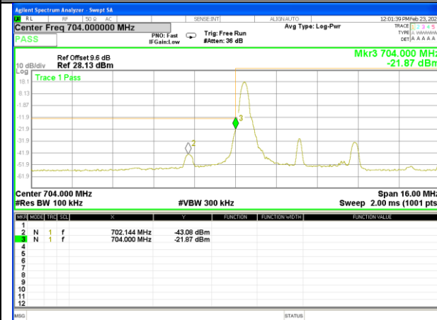
Band17_5M_16QAM_Low_1-RB
