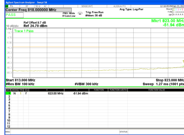
Band26_1.4M_QPSK_Low_Full-RB
