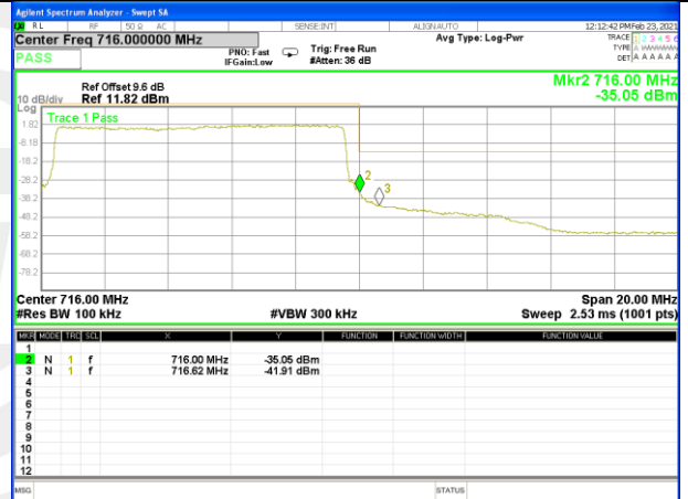
Band17_10M_16QAM_High_Full-RB
