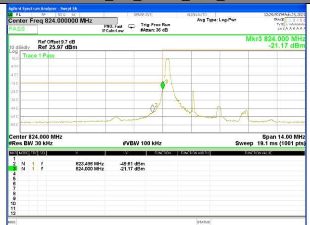
Band26_3M_QPSK_Low_1-RB
