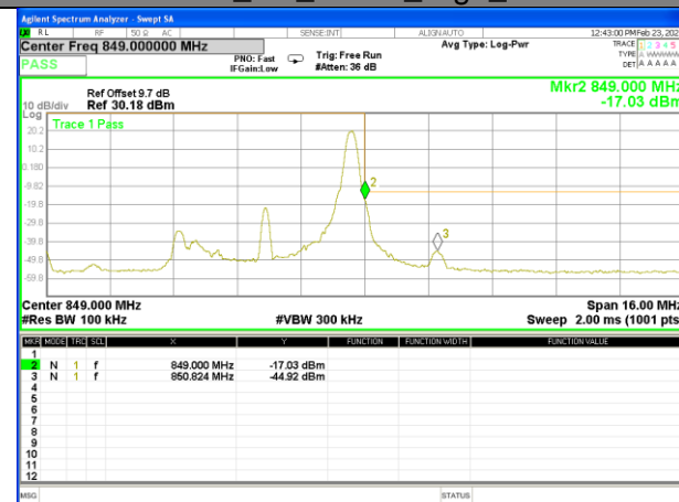
Band26_5M_QPSK_High_1-RB
