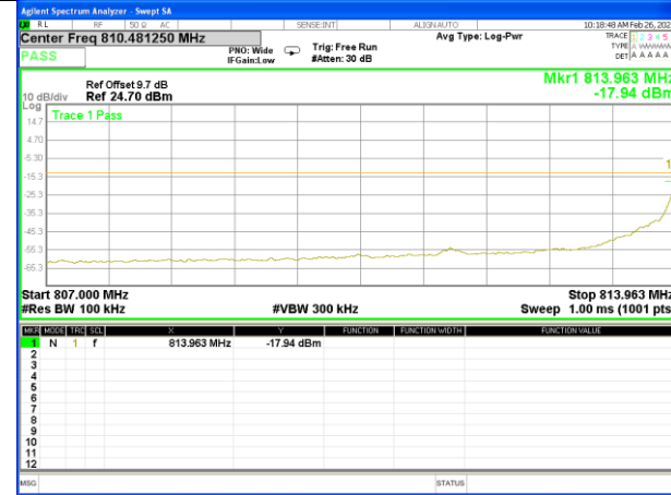
Band 26_1.4M_QPSK_Low_Full-RB
