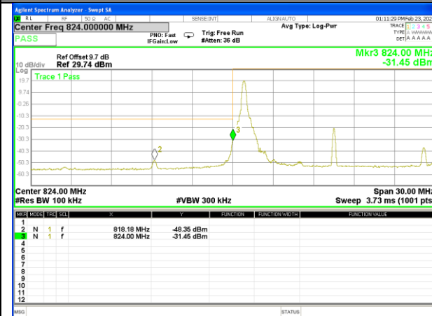
Band26_15M_16QAM_Low_1-RB
