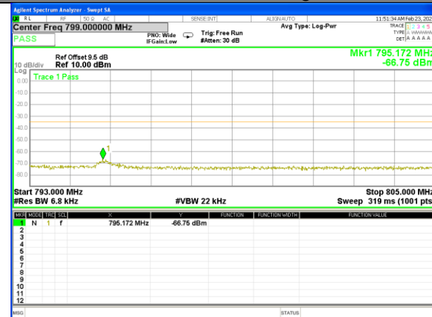
Band13_10M_16QAM_High_1-RB
