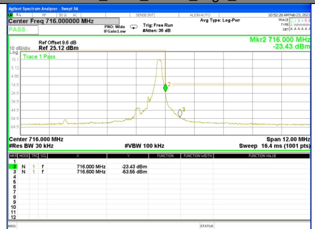
Band12_1.4M_QPSK_High_1-RB
