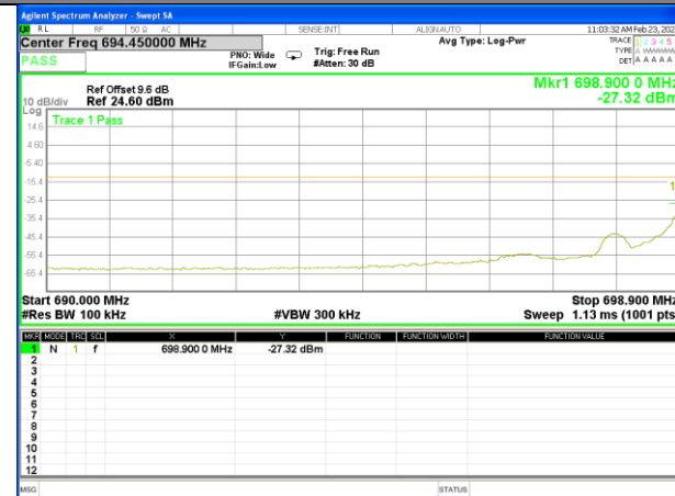
Band12_3M_QPSK_Low_1-RB
