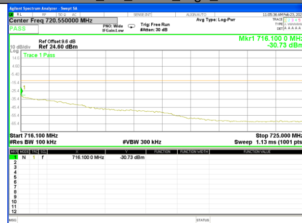
Band12_3M_QPSK_High_Full-RB
