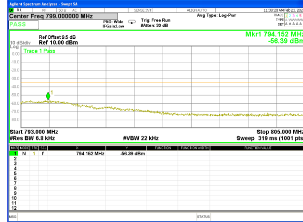
Band13_5M_16QAM_Low_1-RB
