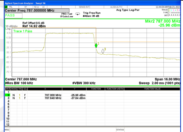
Band13_10M_QPSK_Low_1-RB
