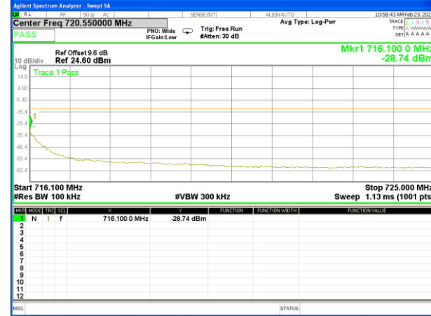
Band12_1.4M_16QAM_High_Full-RB
