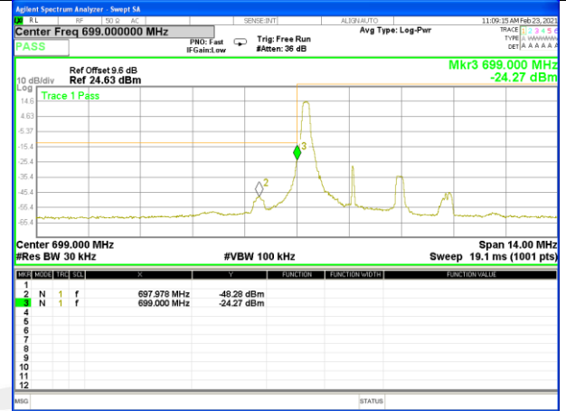
Band12_3M_16QAM_Low_Full-RB
