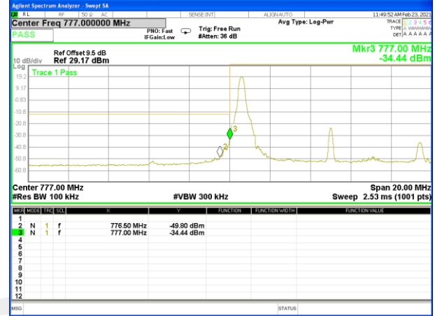
Band13_10M_16QAM_Low_Full-RB
