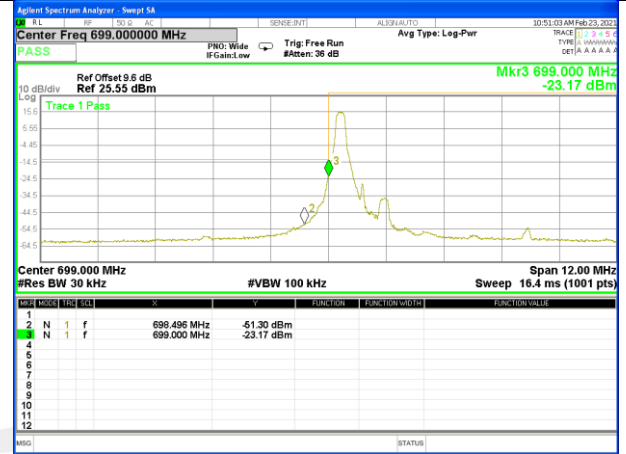
Band12_1.4M_QPSK_Low_Full-RB
