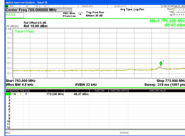
Band13_10M_16QAM_Low_Full-RB
