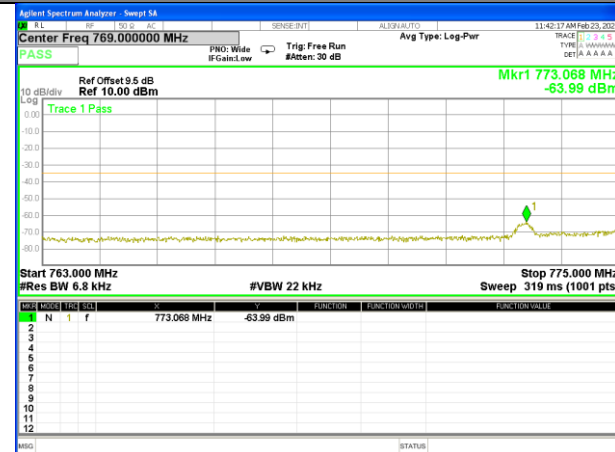
Band13_5M_16QAM_Low_Full-RB
