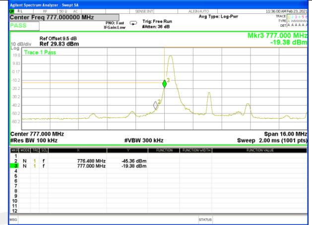
Band13_5M_QPSK_Low_Full-RB
