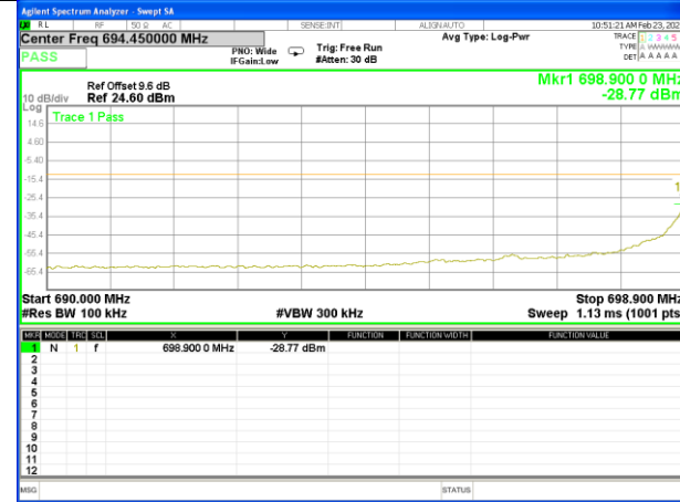
Band12_1.4M_QPSK_Low_Full-RB
