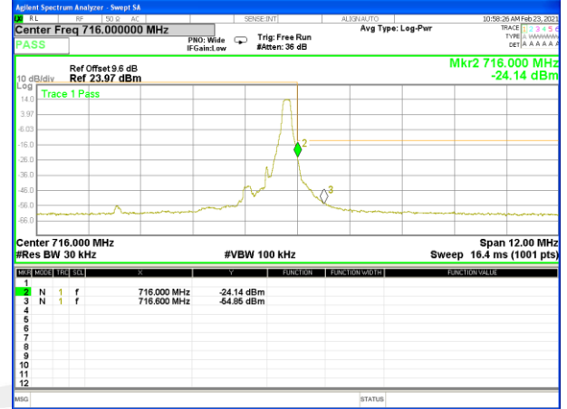
Band12_1.4M_16QAM_High_Full-RB
