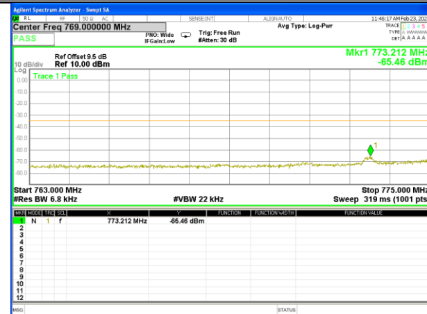
Band13_10M_QPSK_Low_1-RB
