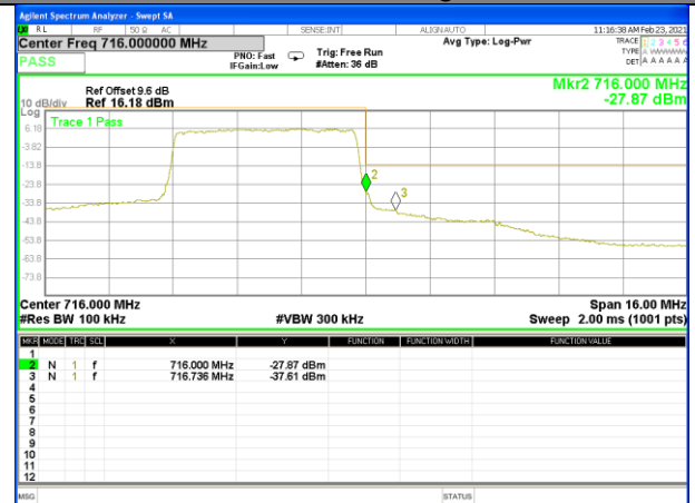
Band12_5M_QPSK_High_Full-RB
