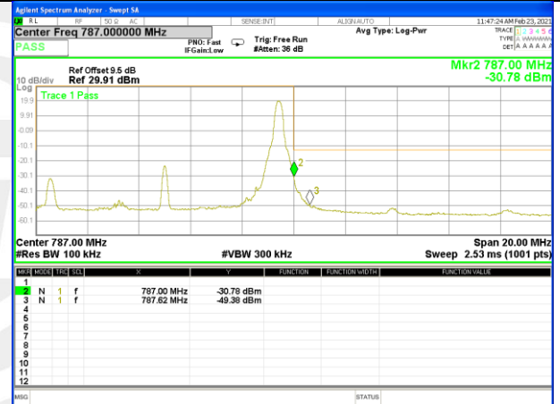
Band13_10M_QPSK_High_Full-RB
