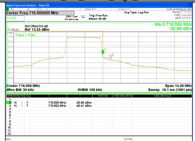
Band12_3M_QPSK_High_Full-RB
