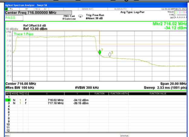
Band12_10M_16QAM_High_Full-RB
