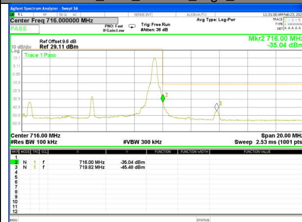
Band12_10M_16QAM_High_1-RB
