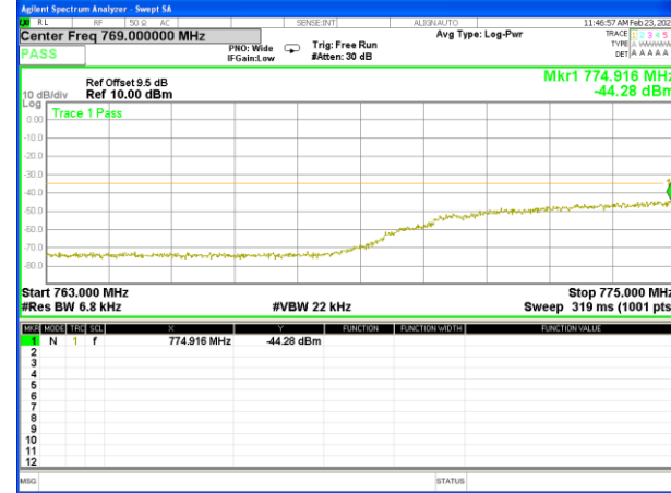
Band13_10M_QPSK_High_1-RB
