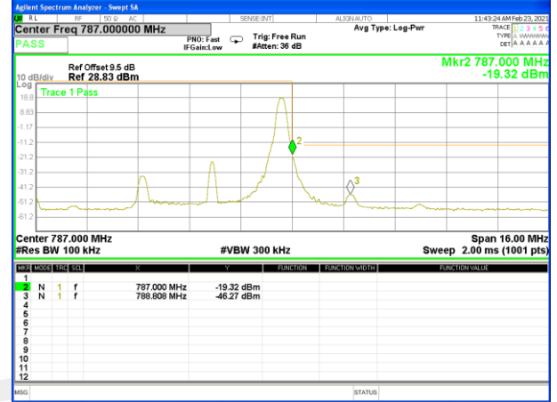
Band13_5M_16QAM_High_Full-RB
