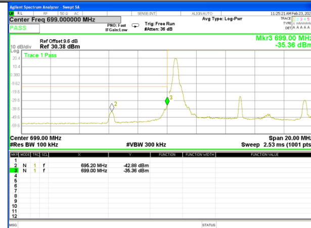
Band12_10M_QPSK_Low_1-RB
