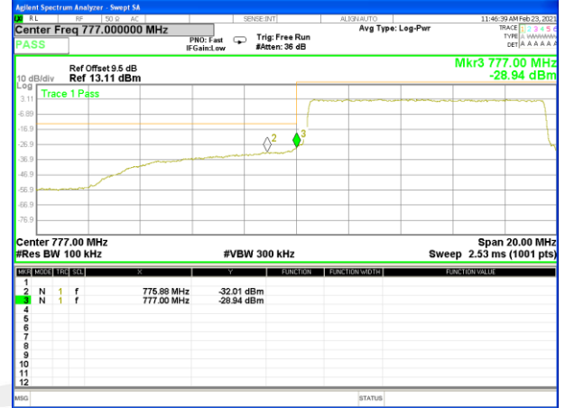
Band13_10M_QPSK_High_1-RB
