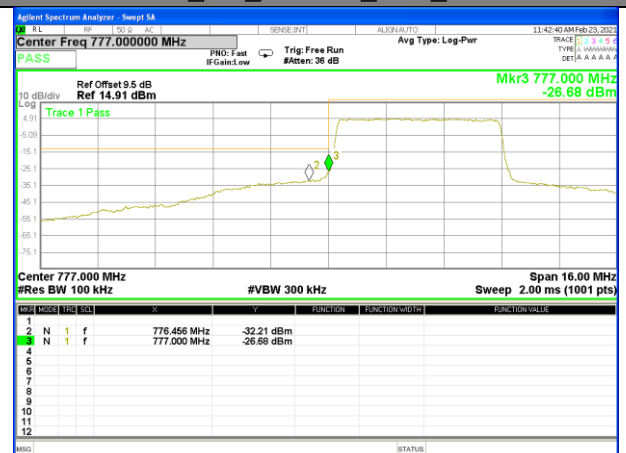
Band13_5M_16QAM_Low_Full-RB
