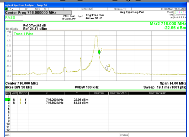
Band12_3M_16QAM_High_1-RB
