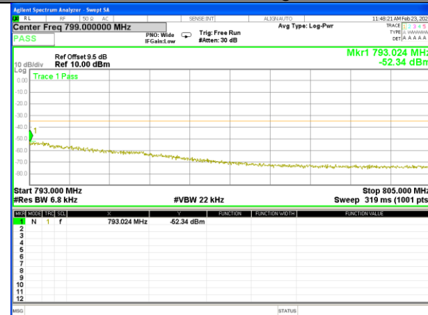
Band13_10M_QPSK_High_Full-RB
