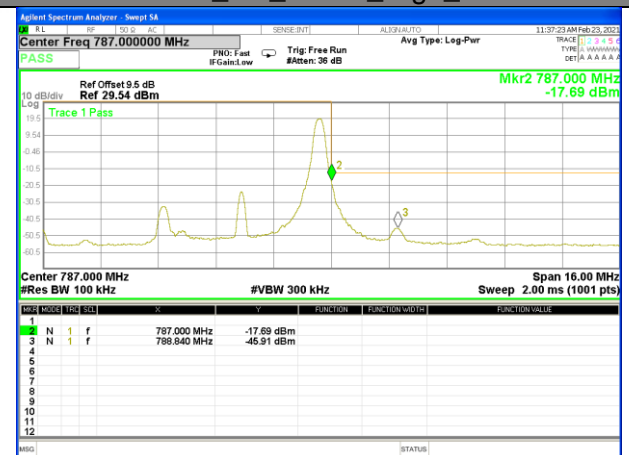
Band13_5M_QPSK_High_1-RB
