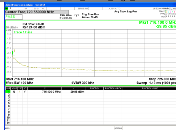
Band12_1.4M_QPSK_High_1-RB
