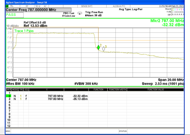
Band13_10M_16QAM_High_Full-RB
