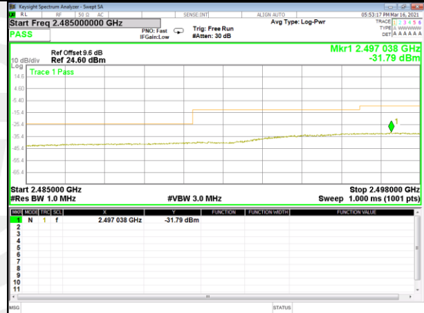
Band 7_10M_QPSK_Low_Full-RB
