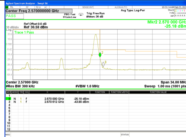
Band 7_15M_16QAM_High_Full-RB
