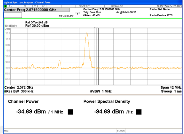
Band 7_15M_QPSK_High_Full-RB
