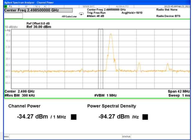
Band 7_15M_QPSK_Low_Full-RB
