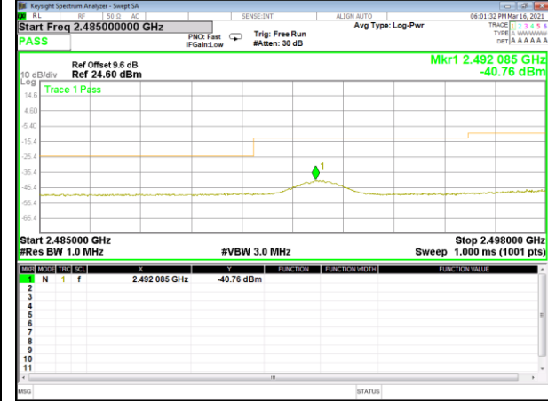
Band 7_20M_16QAM_Low_1-RB
