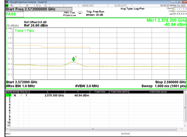
Band 7_10M_QPSK_High_1-RB
