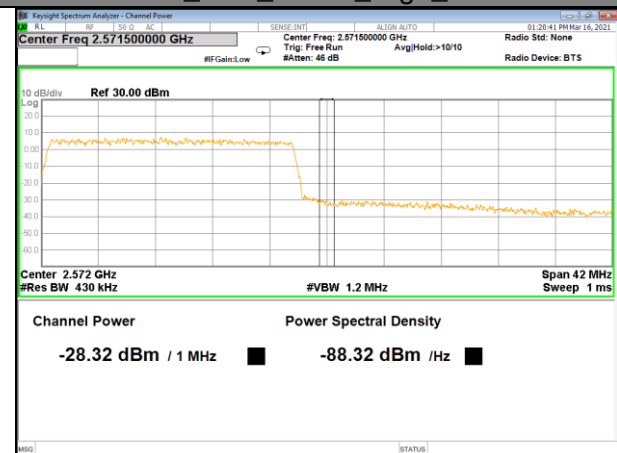
Band 7_20M_QPSK_High_Full-RB
