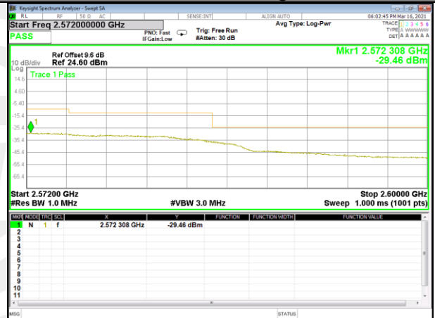
Band 7_20M_QPSK_High_Full-RB
