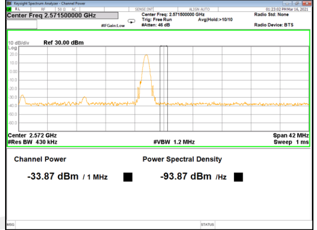
Band 7_20M_16QAM_High_Full-RB
