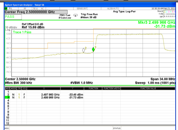
Band 7_15M_16QAM_Low_Full-RB
