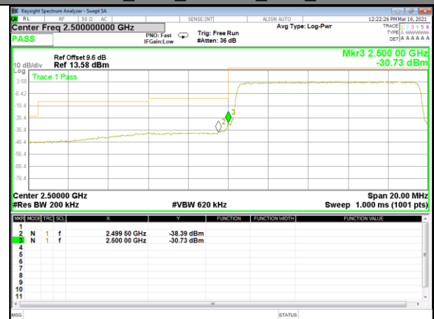
Band 7_10M_16QAM_Low_Full-RB
