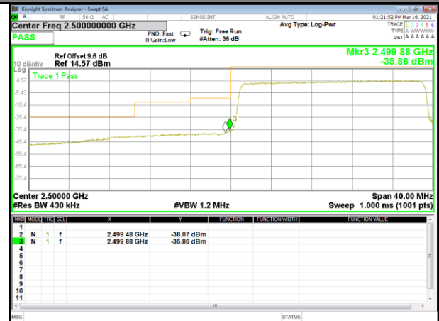
Band 7_20M_16QAM_Low_Full-RB
