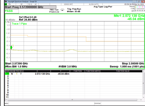
Band 7_15M_QPSK_High_1-RB
