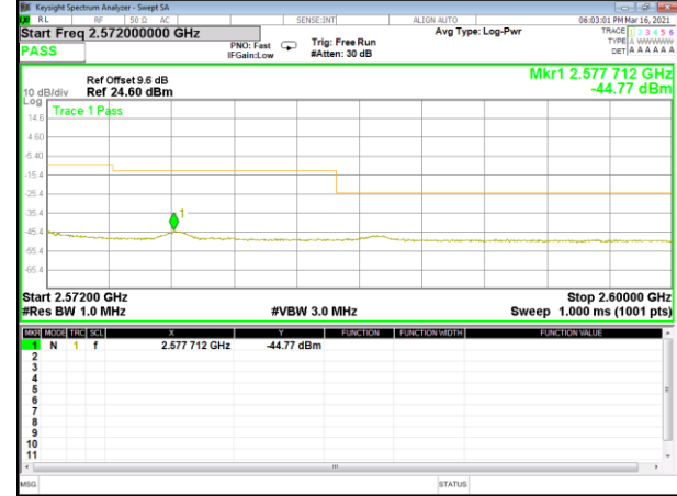
Band 7_20M_QPSK_High_1-RB
