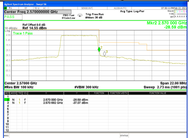
Band 7_5M_16QAM_High_Full-RB
