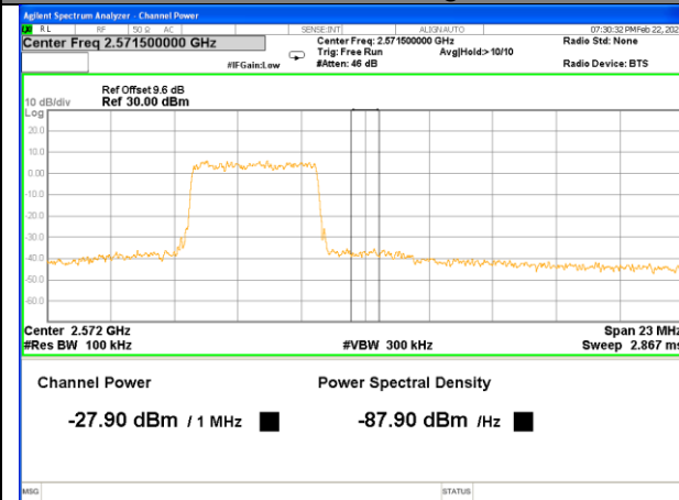
Band 7_5M_16QAM_High_Full-RB
