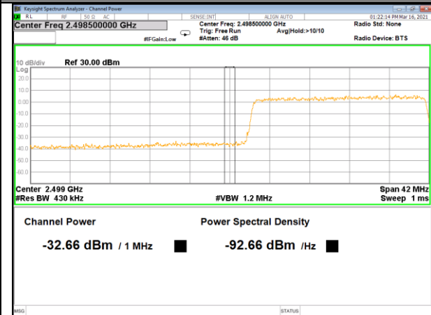
Band 7_20M_16QAM_Low_Full-RB
