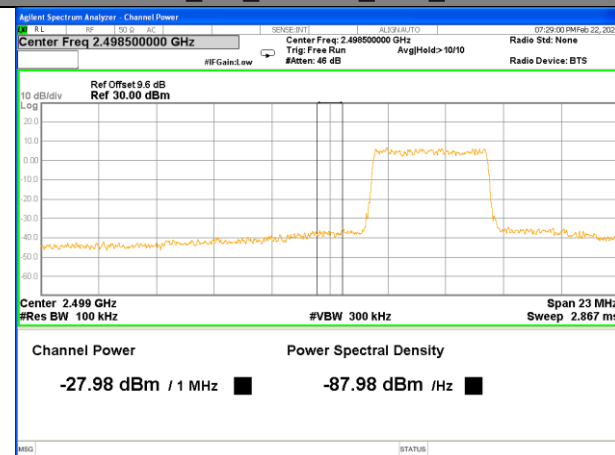
Band 7_5M_16QAM_Low_Full-RB
