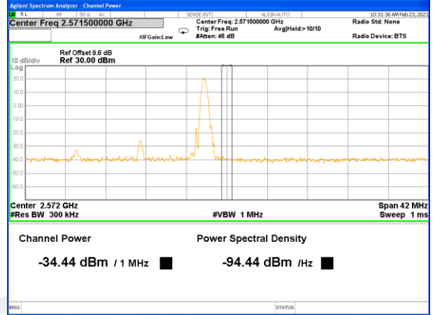
Band 7_15M_16QAM_High_Full-RB
