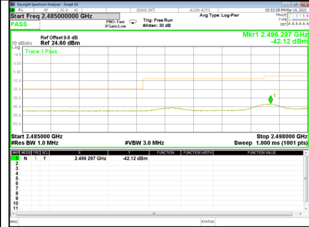
Band 7_10M_16QAM_Low_1-RB
