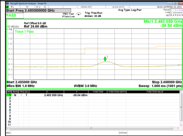
Band 7_20M_QPSK_Low_1-RB
