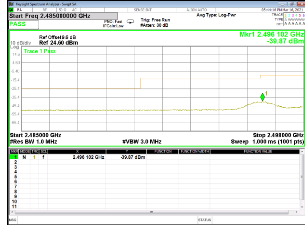
Band 7_5M_16QAM_Low_1-RB
