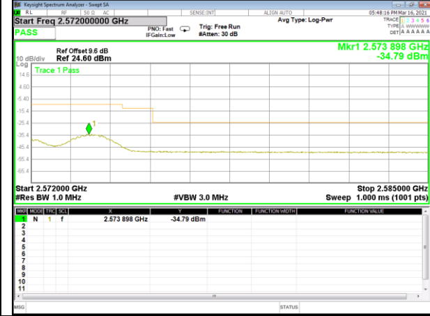
Band 7_5M_16QAM_High_1-RB
