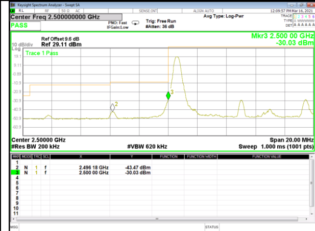
Band 7_10M_QPSK_Low_Full-RB
