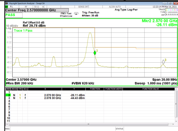
Band 7_10M_16QAM_High_Full-RB
