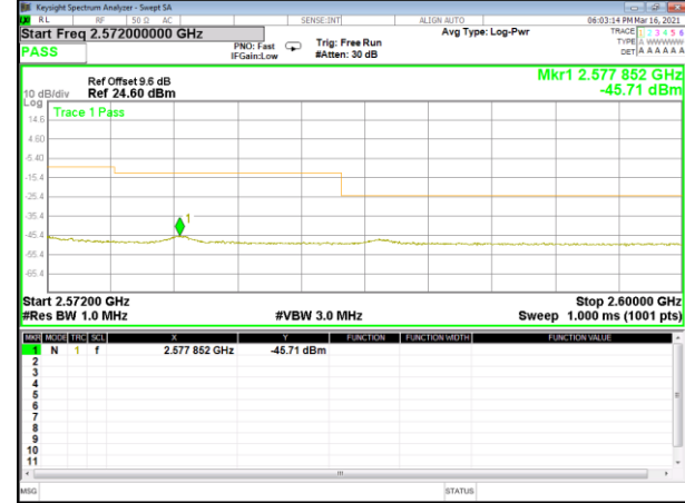
Band 7_20M_16QAM_High_1-RB
