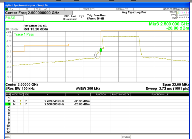
Band 7_5M_16QAM_Low_Full-RB
