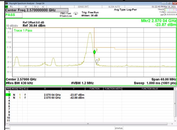
Band 7_20M_16QAM_High_Full-RB
