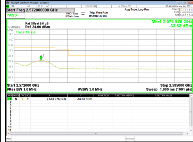
Band 7_5M_QPSK_High_1-RB
