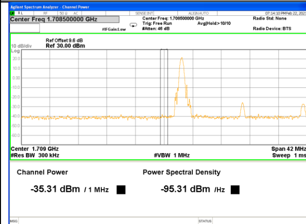
Band4_20M_16QAM_Low_1-RB
