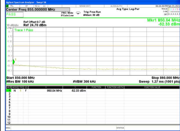
Band5_1.4M_16QAM_High_Full-RB
