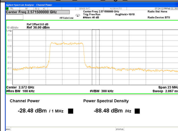
Band 7_5M_QPSK_High_Full-RB
