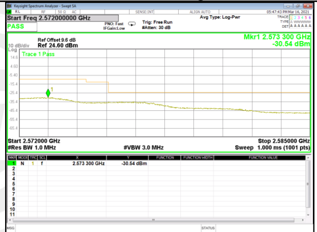
Band 7_5M_QPSK_High_Full-RB
