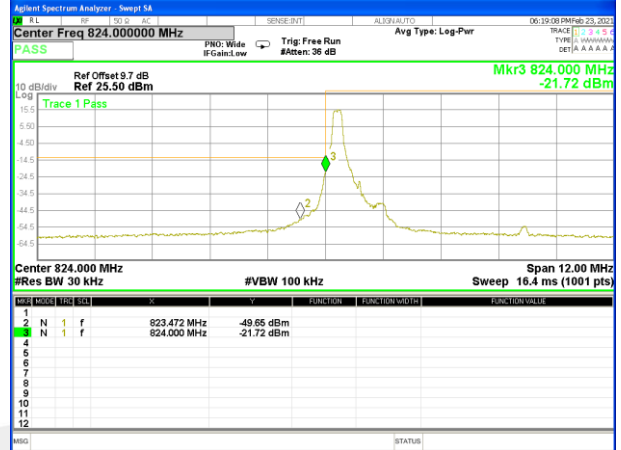
Band5_1.4M_QPSK_Low_Full-RB
