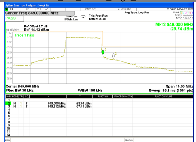
Band5_3M_QPSK_High_Full-RB
