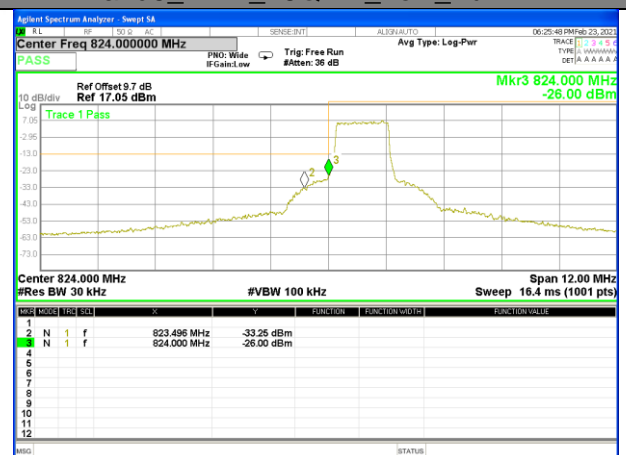
Band5_1.4M_16QAM_Low_Full-RB
