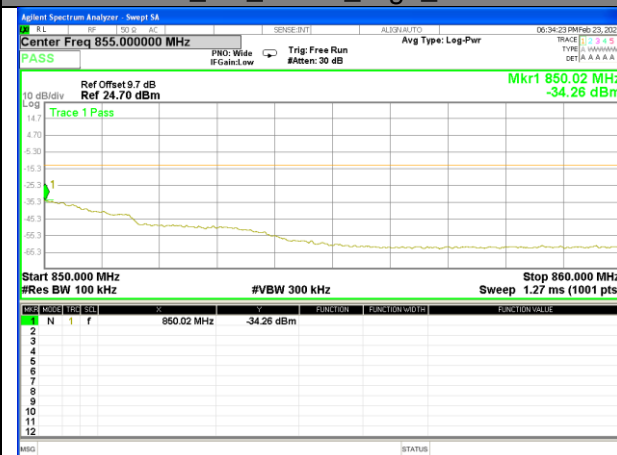
Band5_3M_QPSK_High_Full-RB
