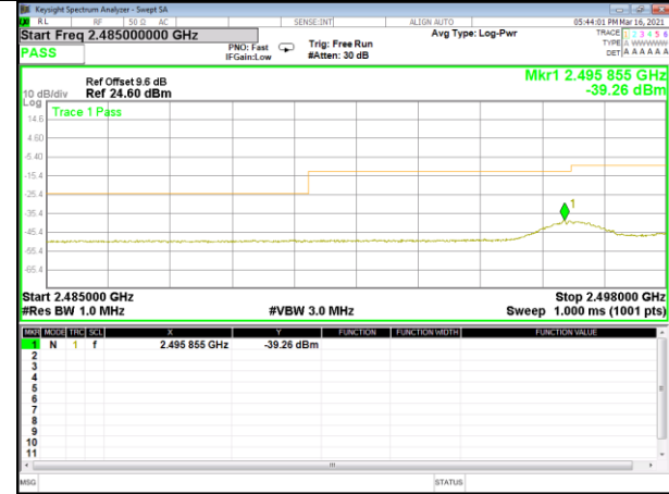
Band 7_5M_QPSK_Low_1-RB
