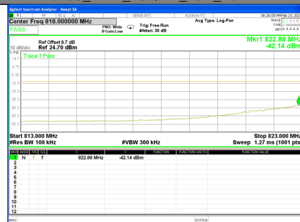
Band5_1.4M_16QAM_Low_Full-RB
