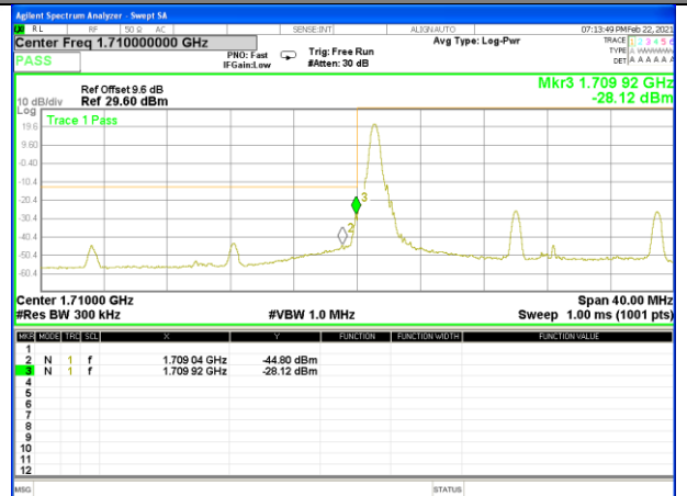
Band4_20M_16QAM_Low_1-RB
