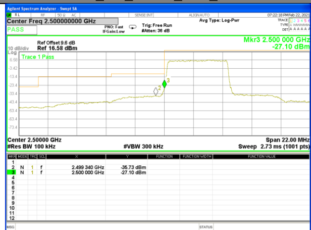
Band 7_5M_QPSK_Low_Full-RB
