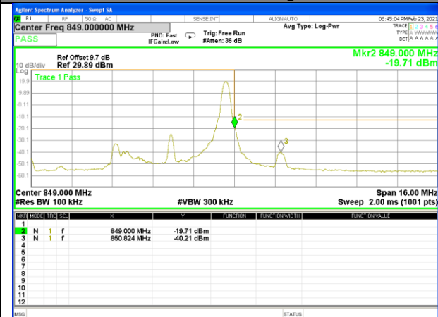
Band5_5M_QPSK_High_1-RB
