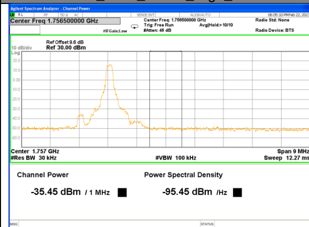
Band4_1.4M_QPSK_High_1-RB
