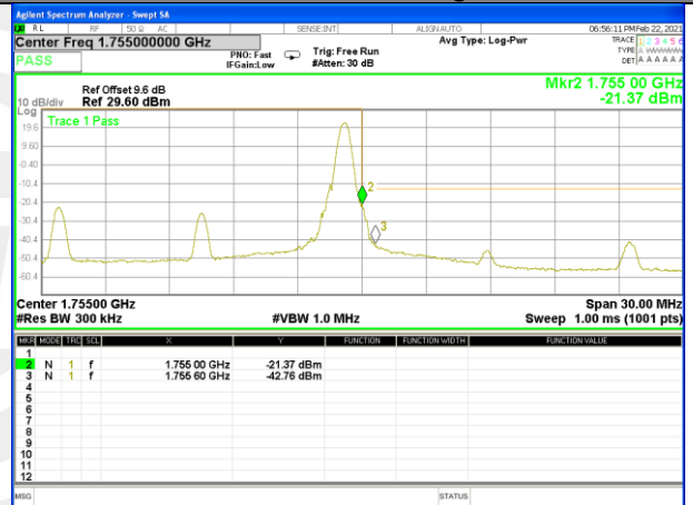
Band4_15M_QPSK_High_Full-RB
