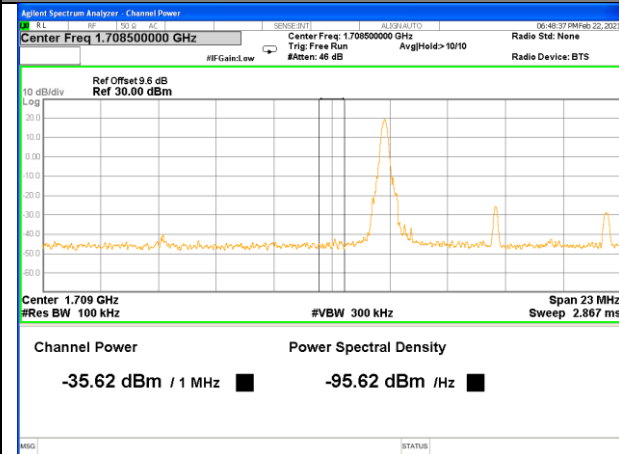
Band4_10M_16QAM_Low_Full-RB
