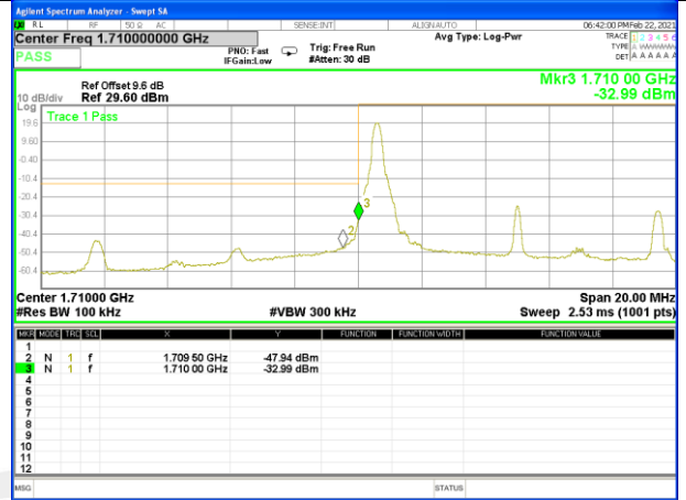
Band4_10M_QPSK_Low_Full-RB
