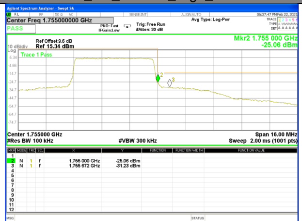
Band4_5M_16QAM_High_Full-RB
