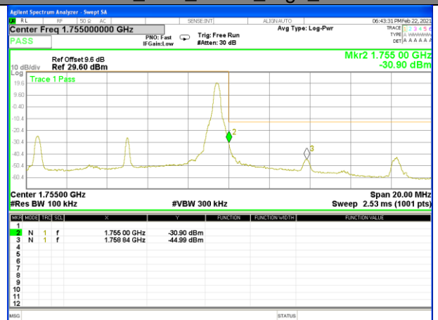
Band4_10M_QPSK_High_1-RB
