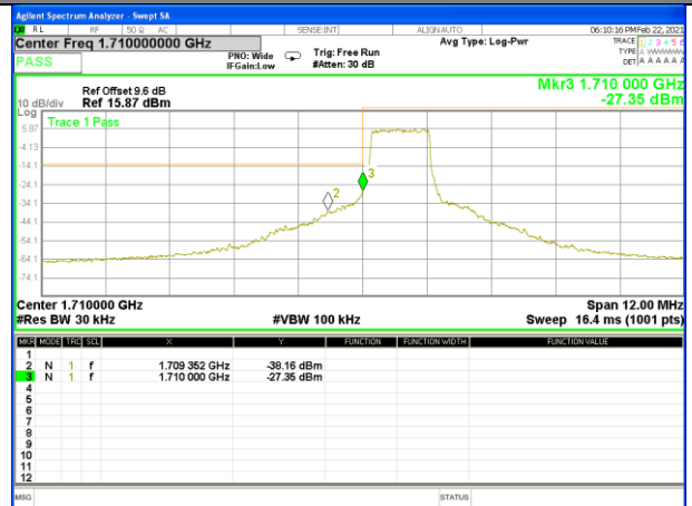
Band4_1.4M_16QAM_Low_Full-RB
