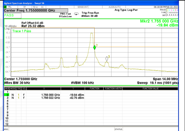
Band4_3M_QPSK_High_Full-RB
