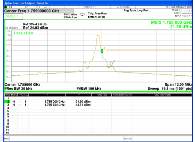
Band4_1.4M_16QAM_High_Full-RB
