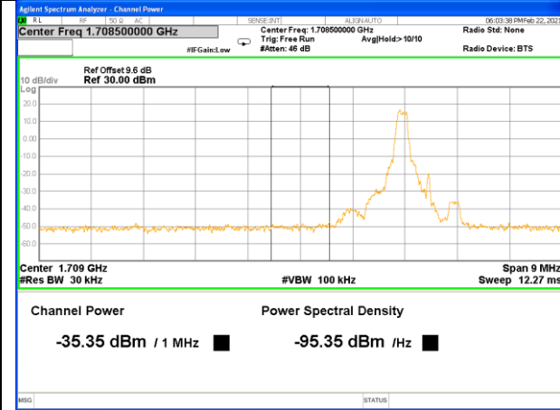
Band4_1.4M_QPSK_Low_Full-RB
