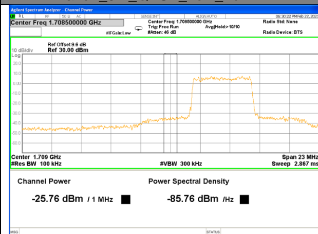
Band4_5M_QPSK_Low_Full-RB
