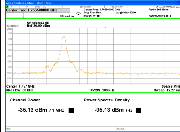
Band4_1.4M_16QAM_High_Full-RB
