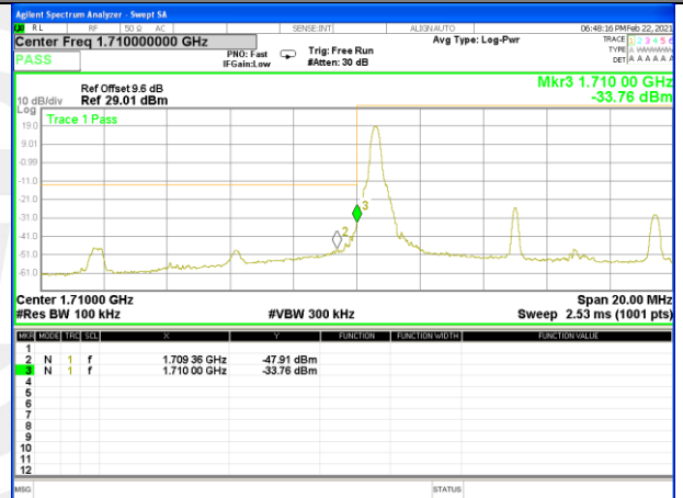
Band4_10M_16QAM_Low_Full-RB
