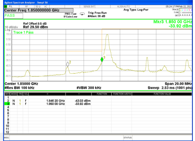
Band2_10M_QPSK_Low_Full-RB
