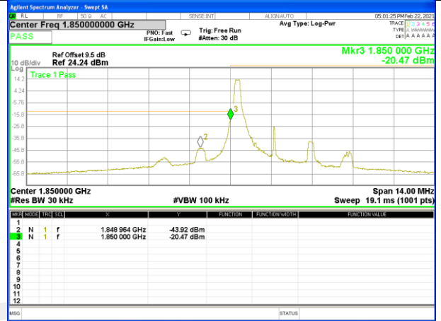
Band2_3M_16QAM_Low_Full-RB
