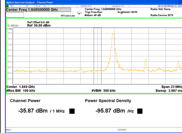
Band2_10M_QPSK_Low_Full-RB
