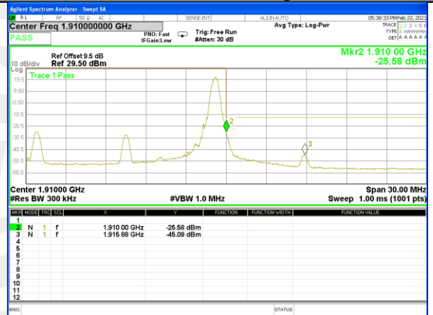
Band2_15M_QPSK_High_Full-RB
