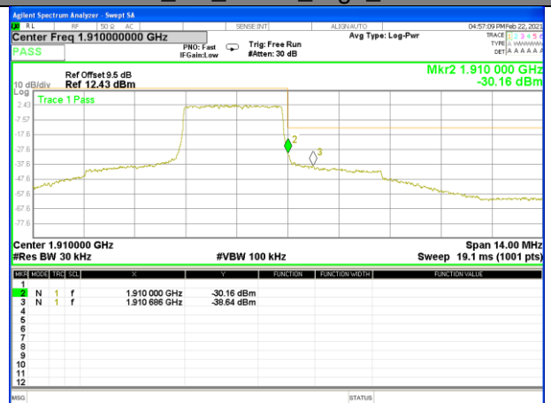
Band2_3M_QPSK_High_Full-RB
