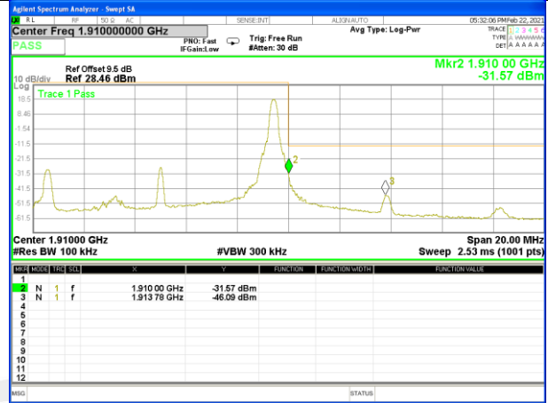
Band2_10M_16QAM_High_Full-RB
