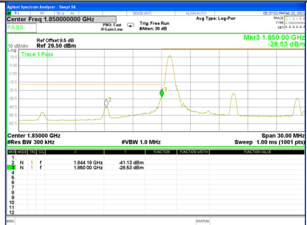
Band2_15M_QPSK_Low_1-RB
