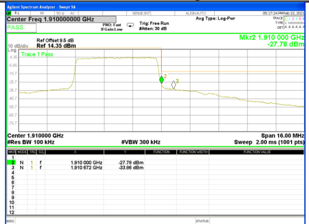
Band2_5M_16QAM_High_Full-RB
