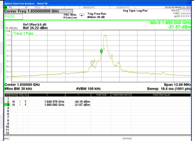
Band2_1.4M_16QAM_Low_Full-RB
