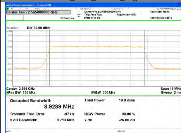
Band7_10M_QPSK_High
