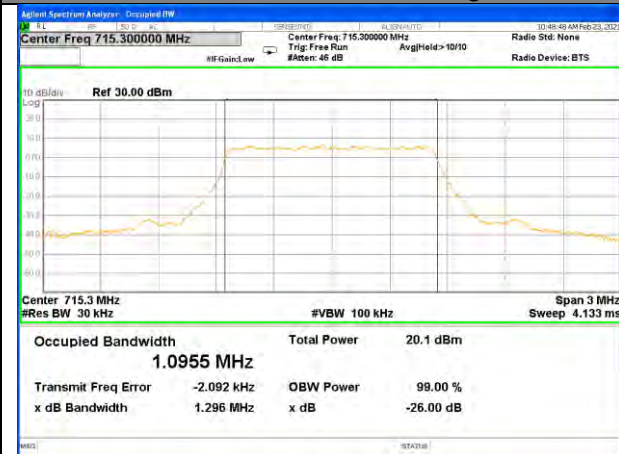
Band12_1.4M_QPSK_High
