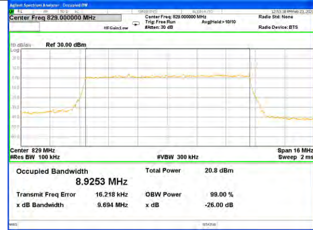
Band26_10M_QPSK_Middle
