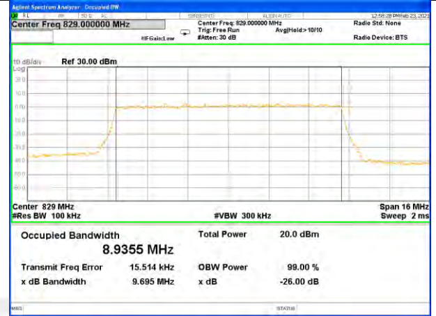
Band26_10M_16QAM_Middle
