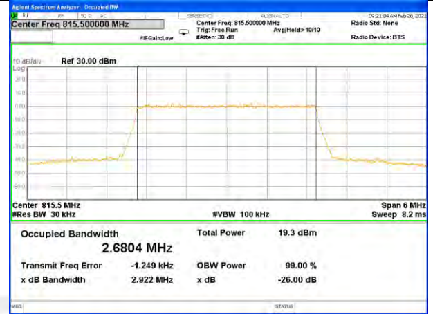
Band26_3M_16QAM_Middle
