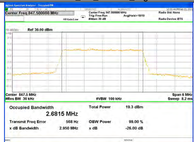
Band26_3M_16QAM_High
