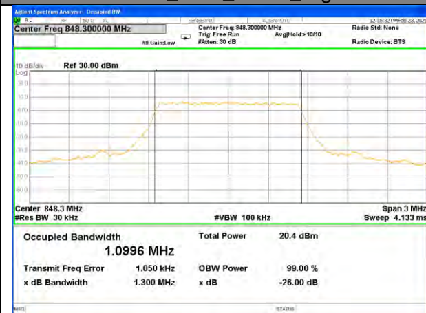
Band26_1.4M_QPSK_High
