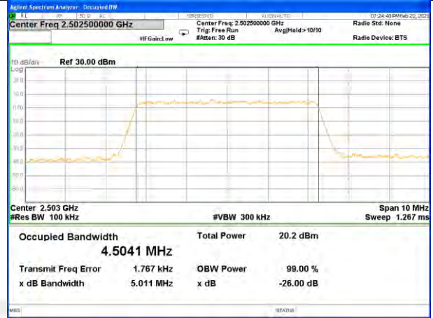
Band7_5M_16QAM_Middle
