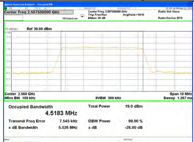
Band7_5M_16QAM_High
