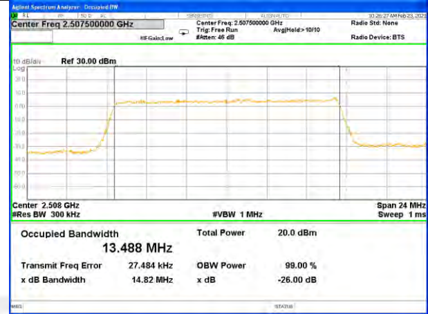
Band7_15M_16QAM_Middle
