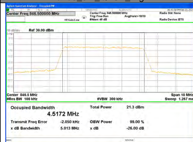
Band5_5M_QPSK_High
