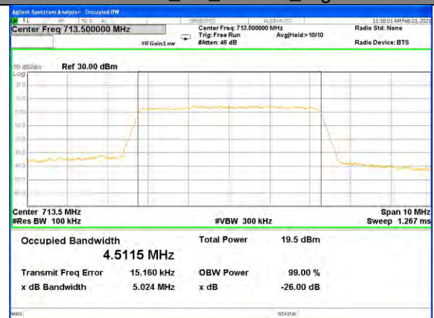
Band12_5M_16QAM_High
