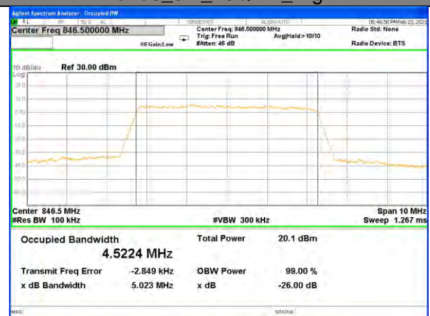
Band5_5M_16QAM_High
