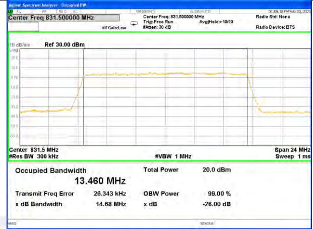
Band26_15M_16QAM_Middle
