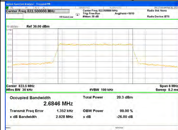
Band26_3M_QPSK_High
