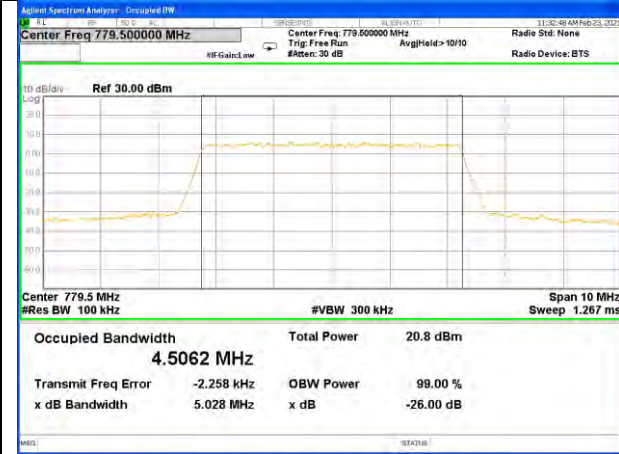
Band13_5M_QPSK_Middle
