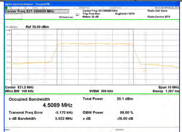
Band26_5M_16QAM_High
