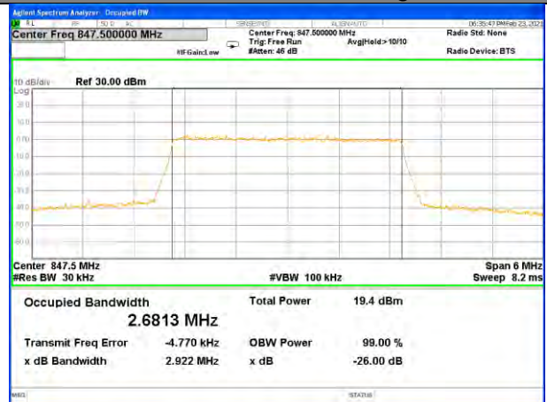
Band5_3M_16QAM_High
