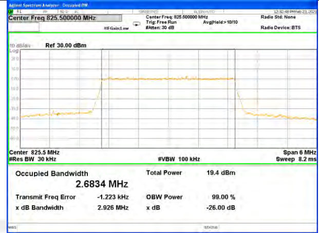
Band26_3M_16QAM_Middle
