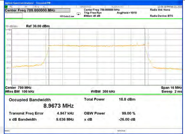
Band17_10M_16QAM_Middle
