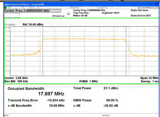
Band41_20M_16QAM_High
