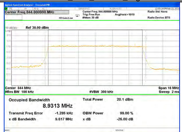
Band26_10M_16QAM_High
