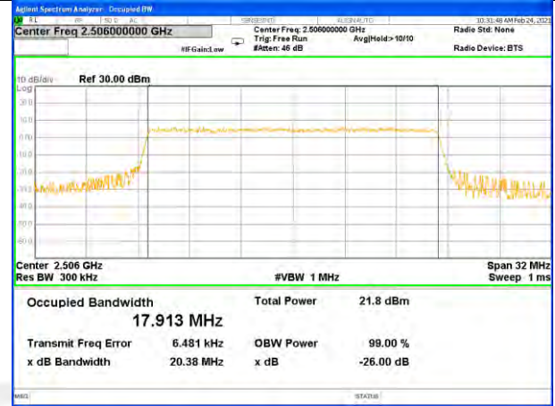
Band41_20M_16QAM_Middle
