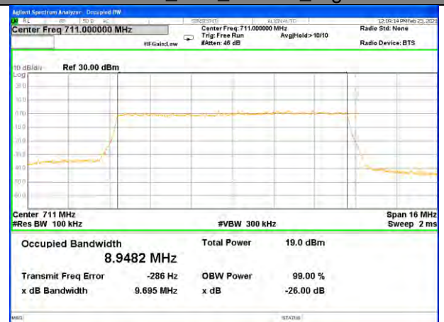
Band17_10M_16QAM_High
