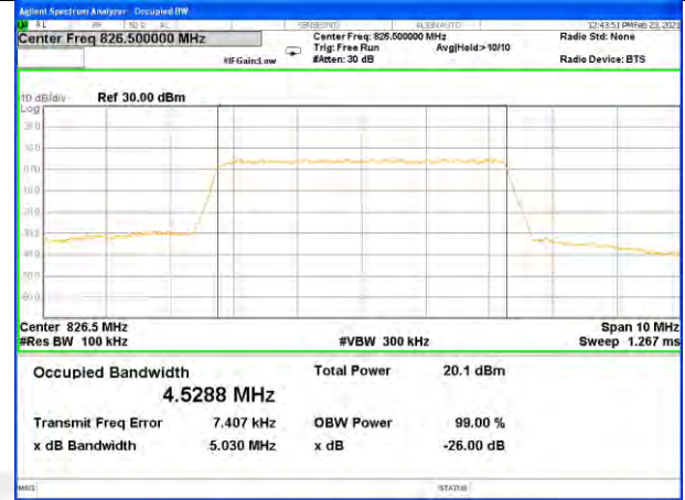
Band26_5M_16QAM_Middle
