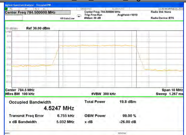
Band13_5M_16QAM_High
