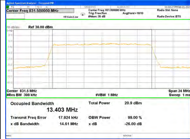
Band26_15M_QPSK_Middle
