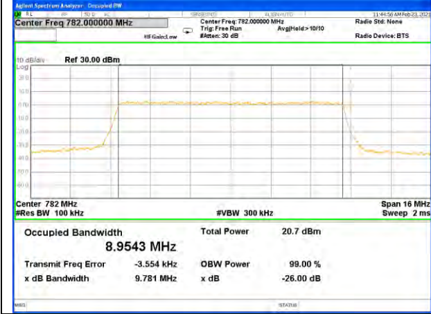
Band13_10M_QPSK_Middle
