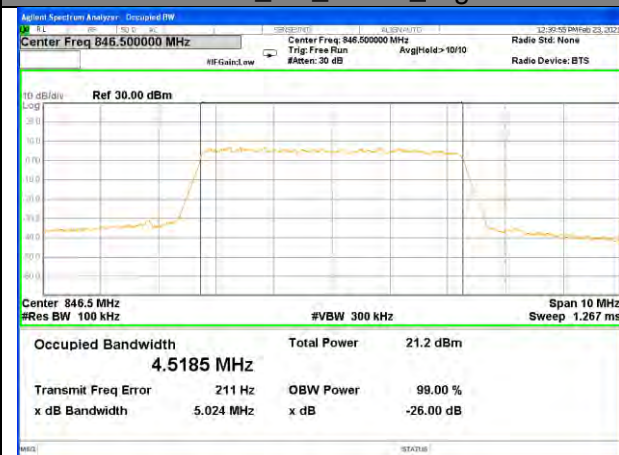
Band26_5M_QPSK_High
