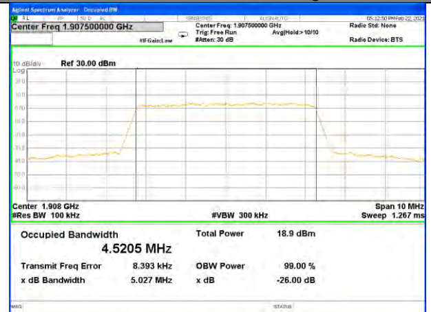
Band2_5M_16QAM_High
