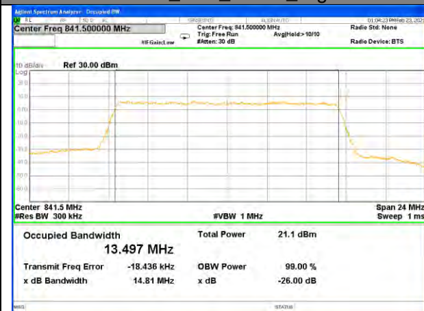
Band26_15M_QPSK_High
