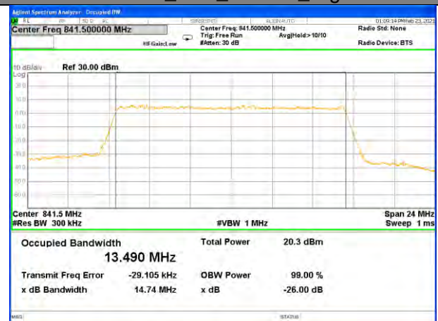
Band26_15M_16QAM_High
