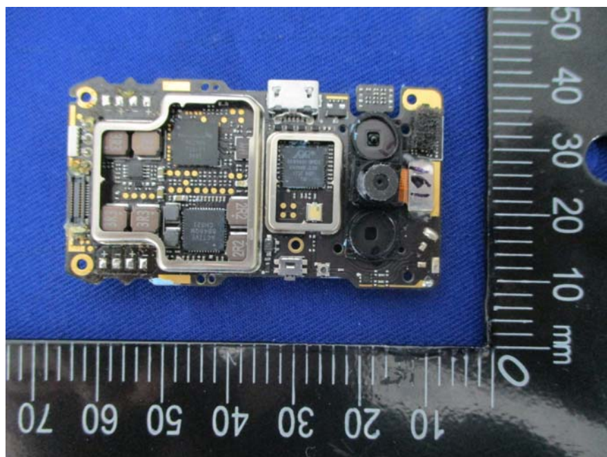
EUT – Mainboard Top Uncover 1 View
