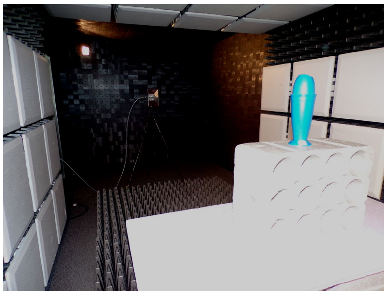
Radiated emissions 30MHz-1GHz (Equipment 80cm above floor)
