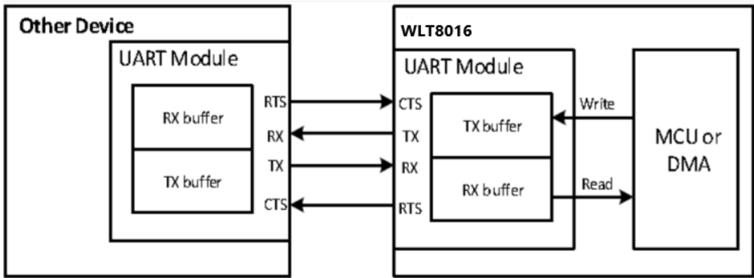
Figure 3-2 UART communication
