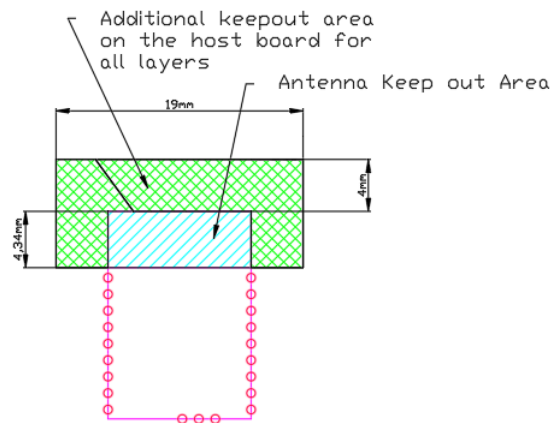
Figure 4-3 Keep out
