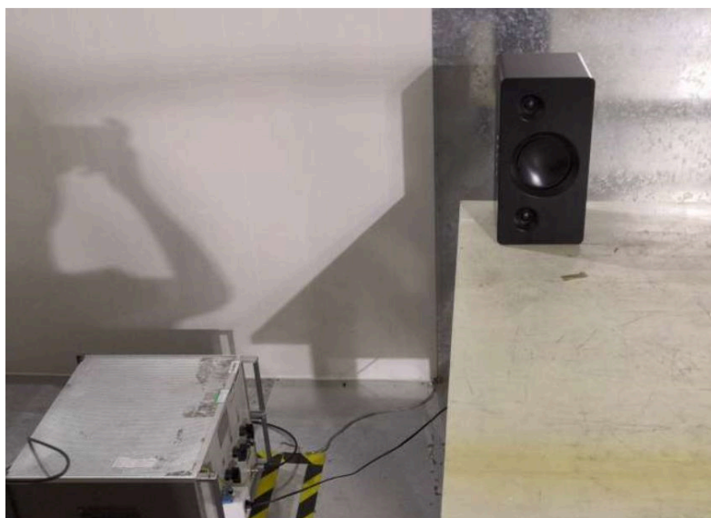
Conducted Emission
