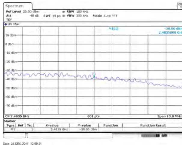
802.11n-20 MHz HIGH CHANNEL, Band Edge
