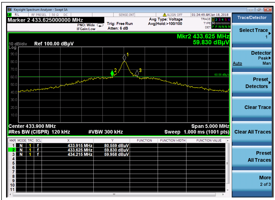
(Bandwidth_433.92MHz)
