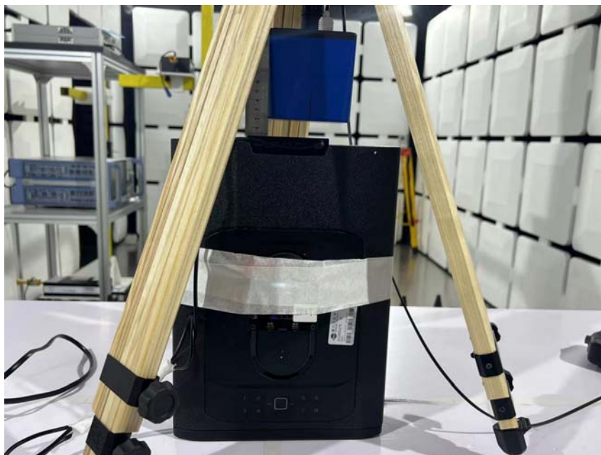
Right Side (Test distance: 2cm)
