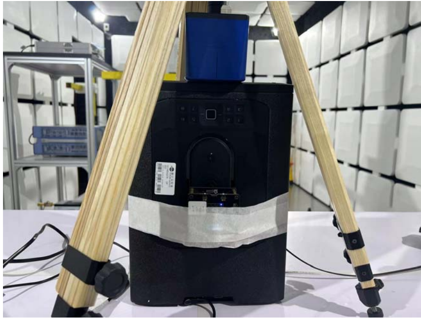
Left Side (Test distance: 0cm)
