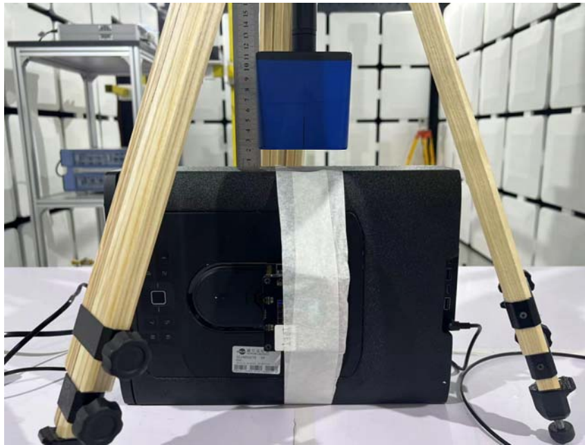
Top Side (Test distance: 2cm)
