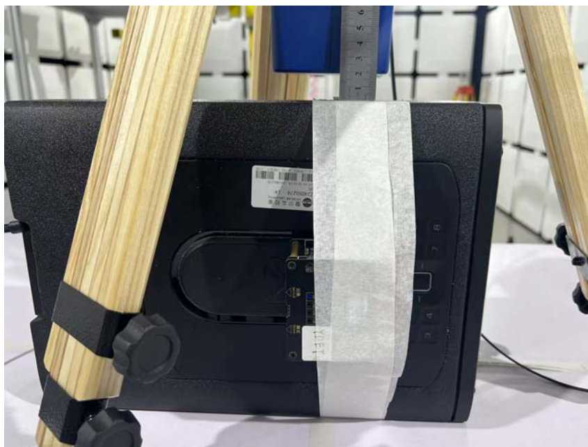
Bottom Side (Test distance: 2cm)
