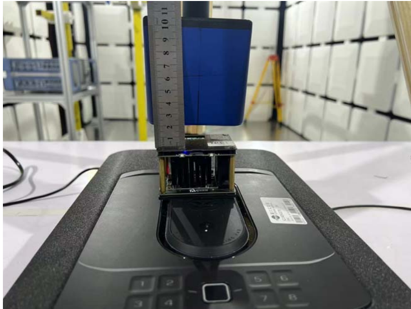
Front Side (Test distance: 2cm)
