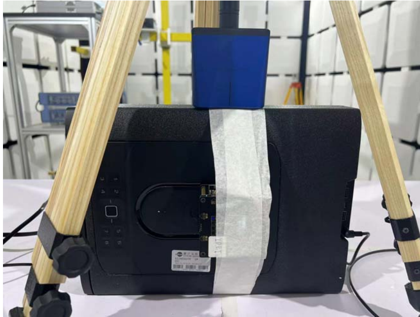
Top Side (Test distance: 0cm)
