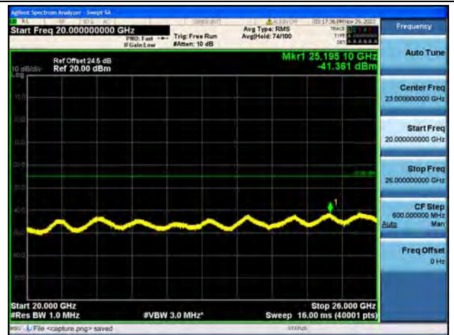
Band7-20G-26G / 20MHz / Mid CH / 16QAM
